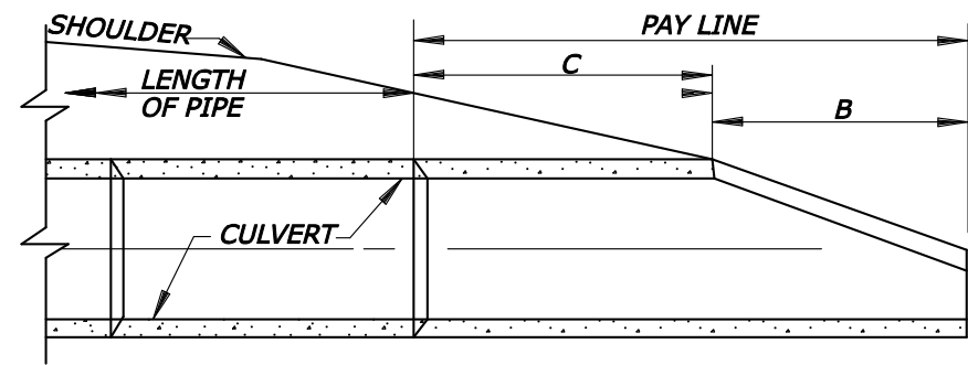
SLOPE DETAIL
