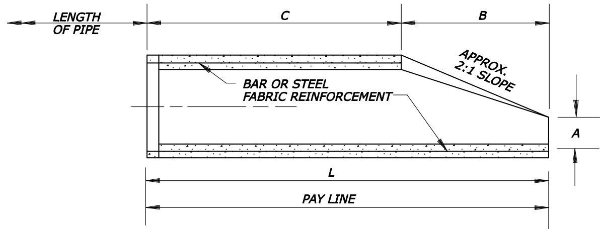
SECTION X-X
