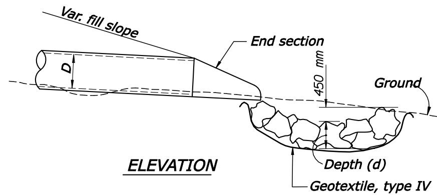
CULVERT WITH END SECTION
