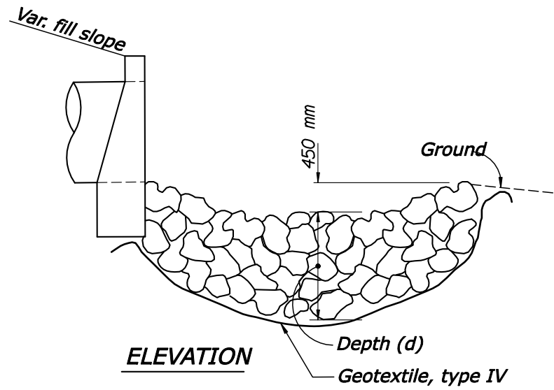
CULVERT WITH HEADWALL
