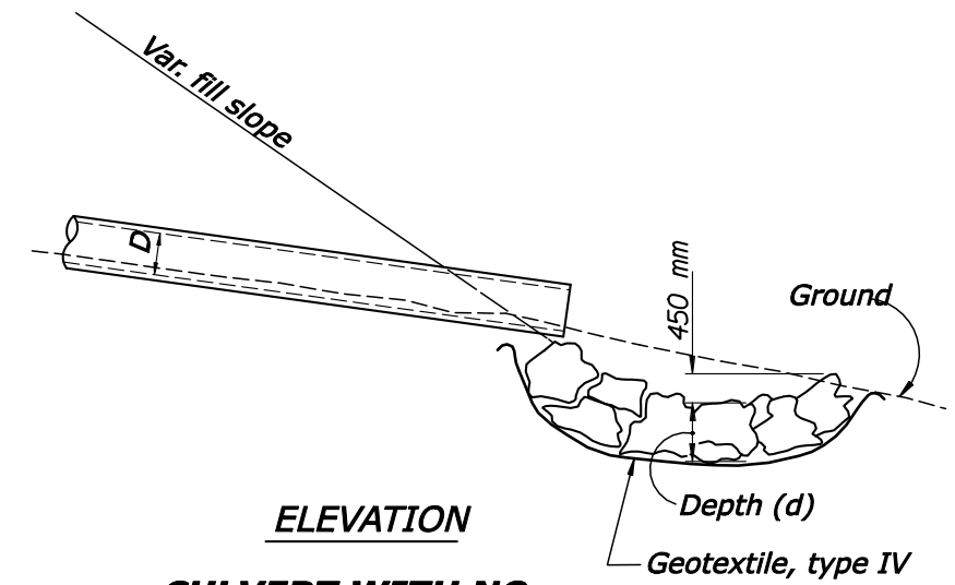
CULVERT WITH NO END TREATMENT
