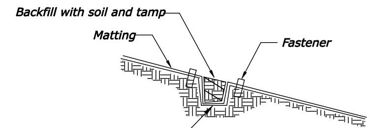
SECTION A-A Erosion Stop (Check Slot) Detail
