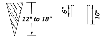
DETAIL A Typical Ground Fasteners
