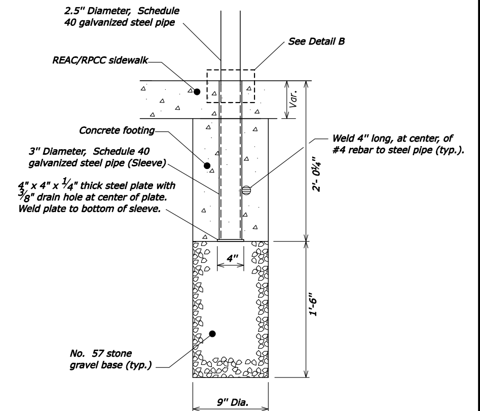
REMOVABLE POST
