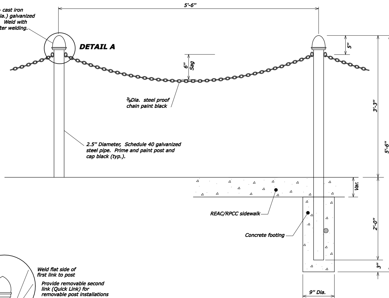
NON-REMOVABLE POST
