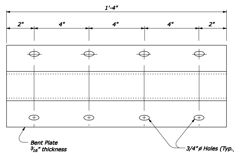
ANCHOR PLATE ARTBA RE-71-79
