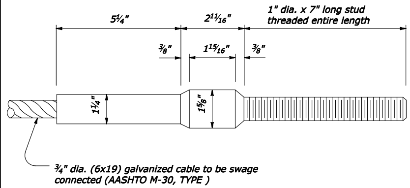
Standard swaged fitting and stud CABLE ASSEMBLY ARTBA F-37-76
