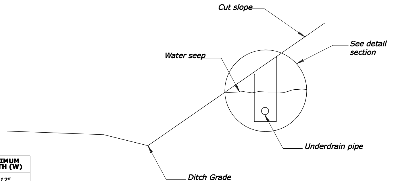
CROSS SECTION
