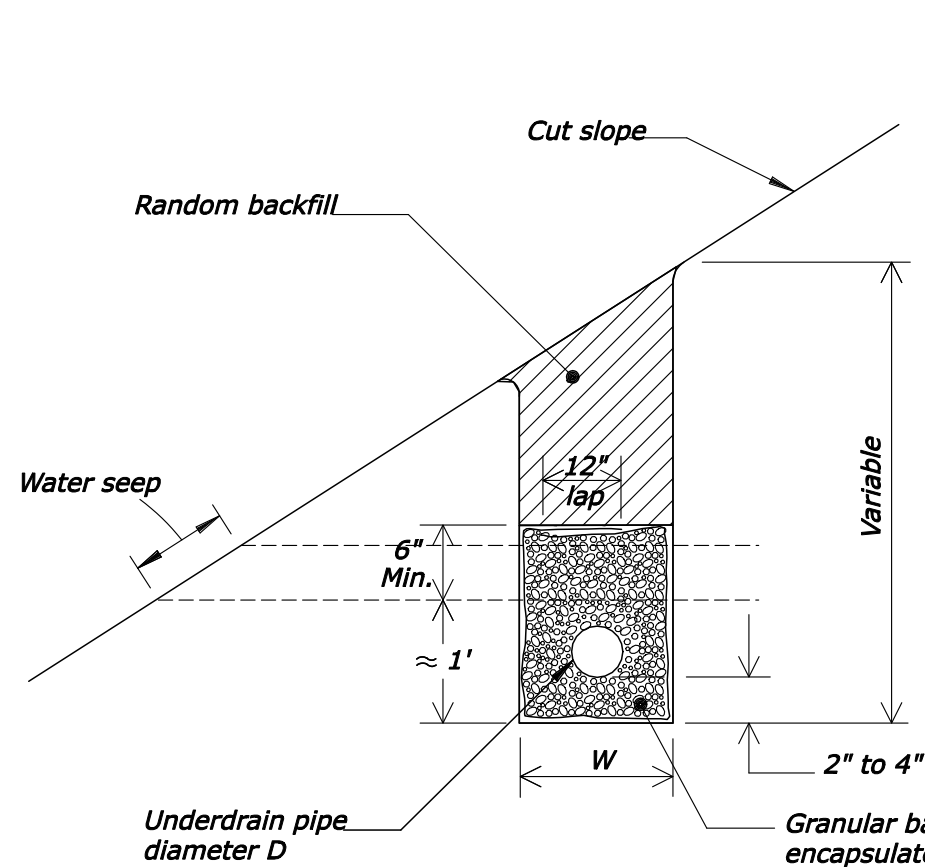
DETAIL SECTION
