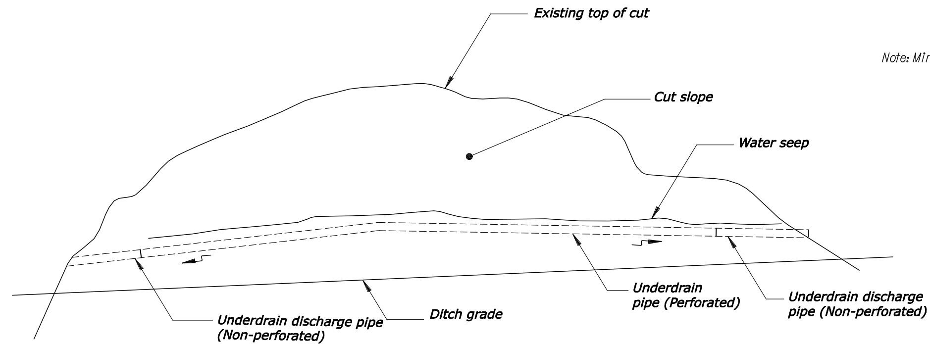
PROFILE VIEW
