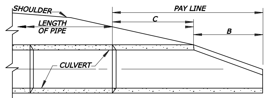
SLOPE DETAIL
