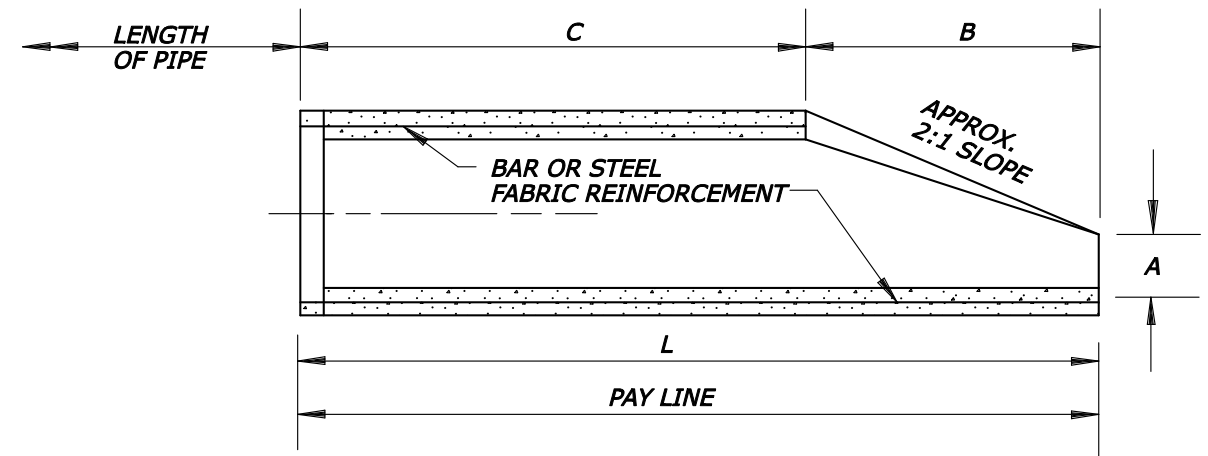
SECTION X-X
