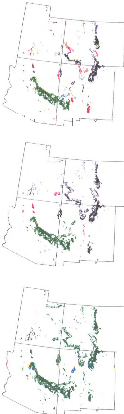
Figure 3.3. Landscape mosaics of discrete clusters of Douglas-fir and Ponderosa pine habitat types, as (a) largest 254 clusters, and at (b) 30-km, and (c) 60-km joining distances. Colors have no significance beyond labelling discrete clusters.
