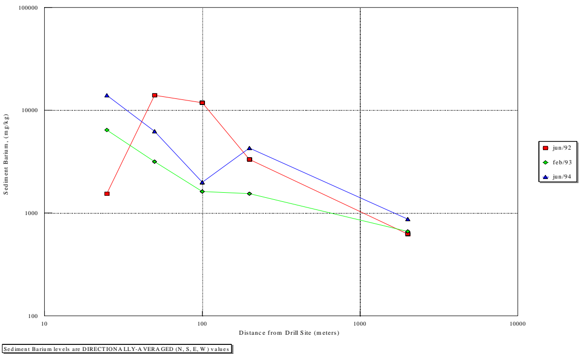
Exhibit 9-9. Sediment Barium vs. Distance from Drill Site
