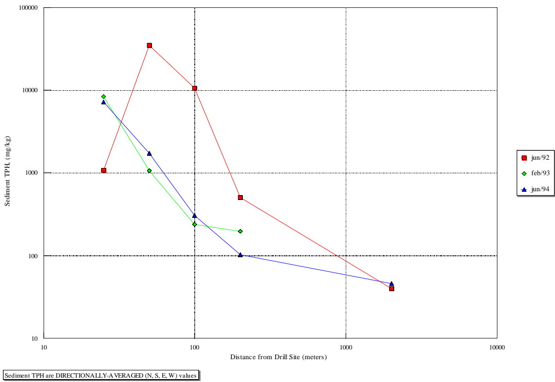
Exhibit 9-8. Sediment TPH vs. Distance from Drill Site
