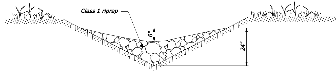
CROSS SECTION
