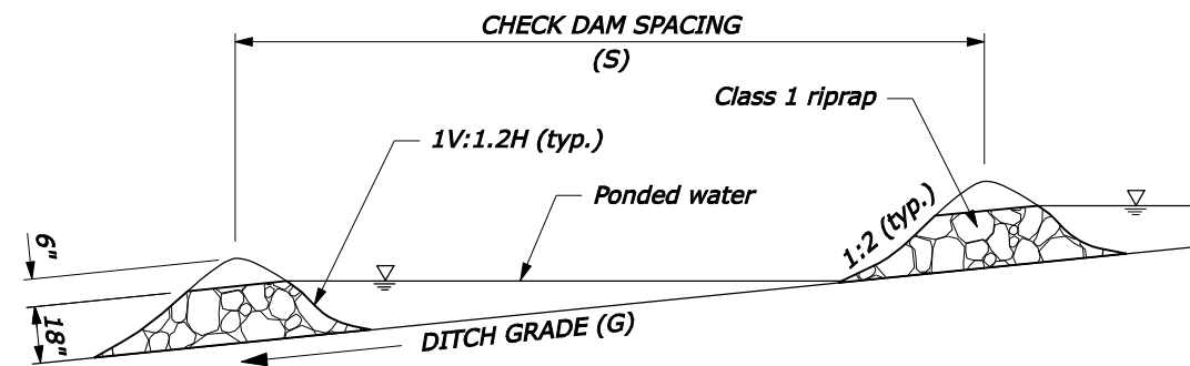
PROFILE VIEW
