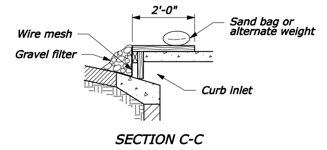
CURB INLET PROTECTION, WOODEN WEIR (TYPE E)
