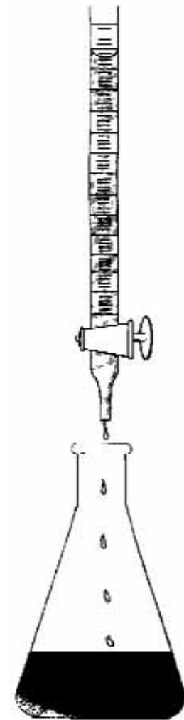
Figure 5.8 Titrating a DO sample using a buret
