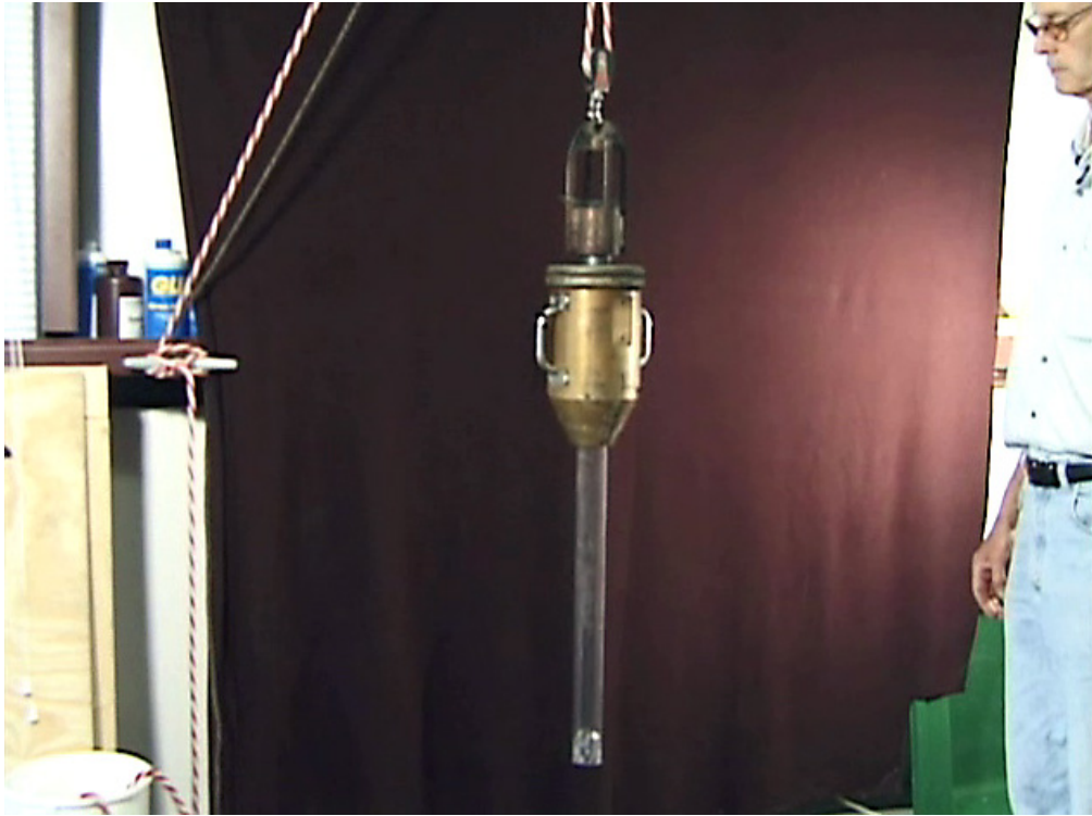
Figure 13. Gravity Core Sampler
