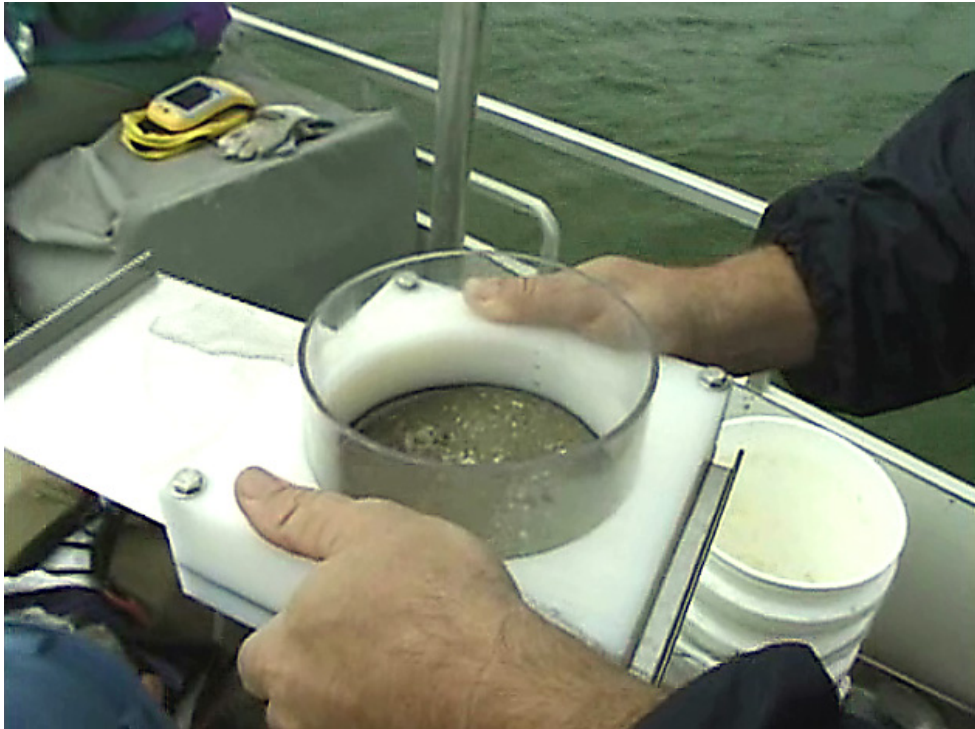
Figure 30. Slicer Block Assembly on Core Tube for Sub-sampling
