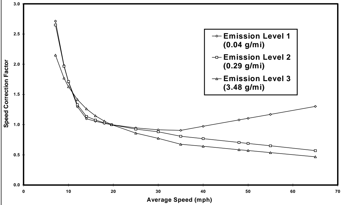
Figure 5a Freeway Speed Correction Factors for Total Hydrocarbons (THC)
