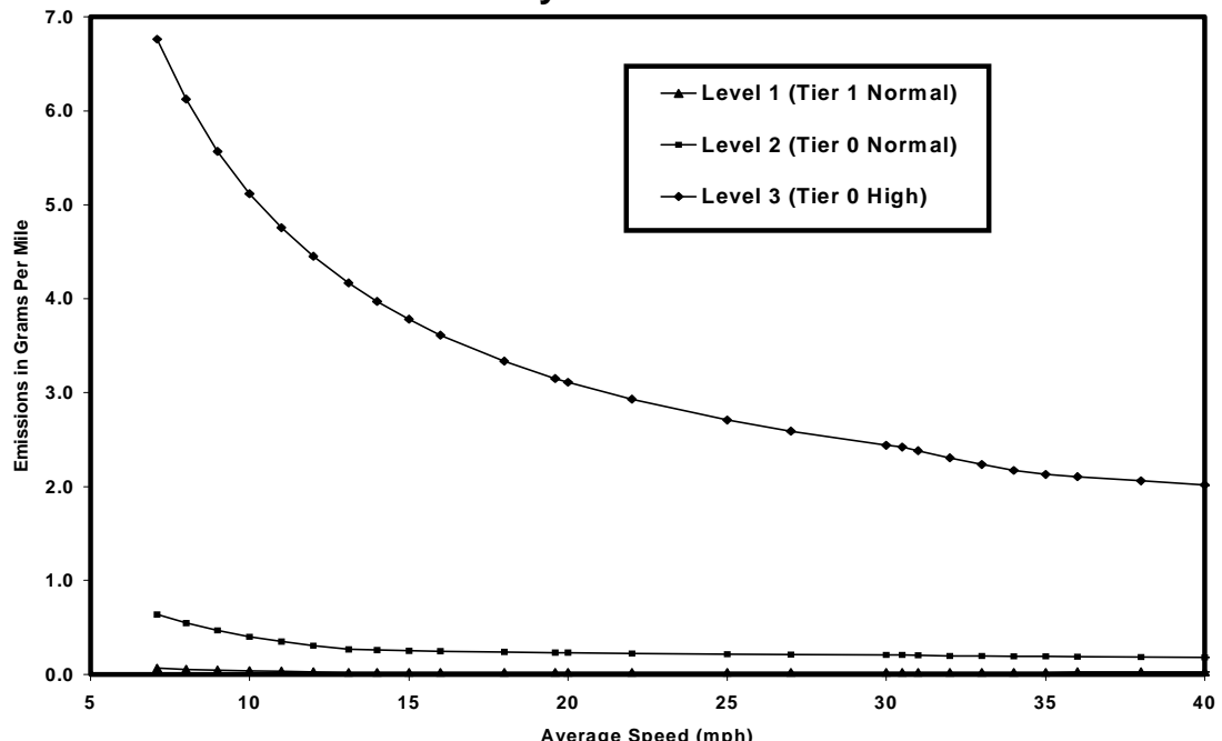
Figure 4d Non-Methane Hydrocarbons (NMHC) Freeway Emission Levels
