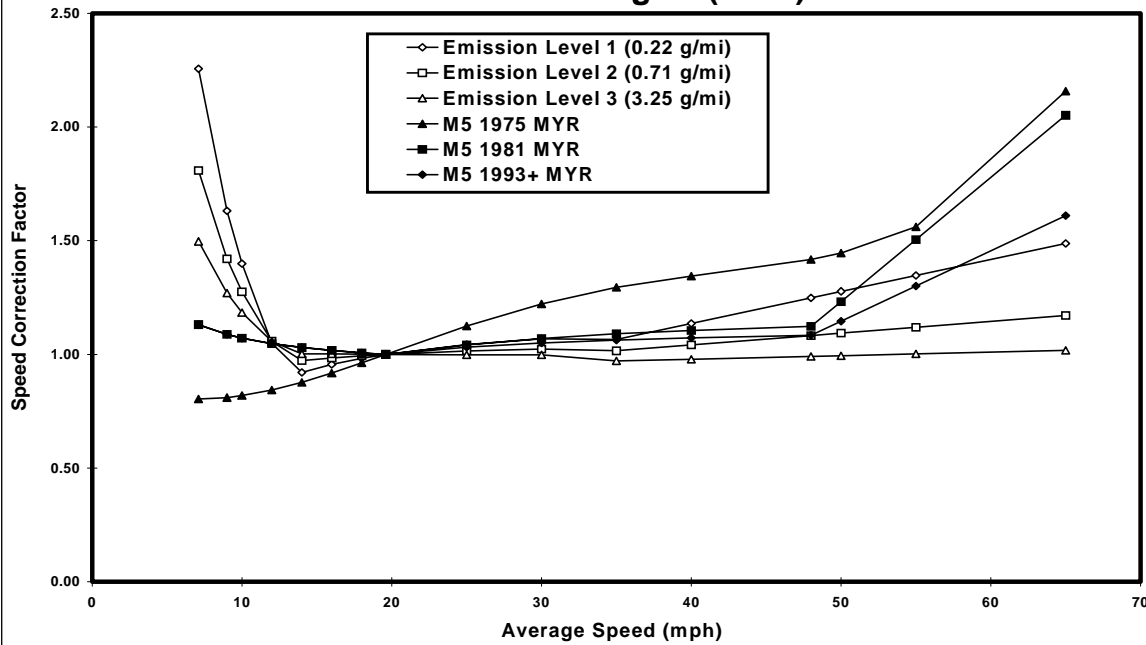
Figure 6c Comparison to MOBILE5 Speed Correction Factors for Oxides of Nitrogen (NO x )
