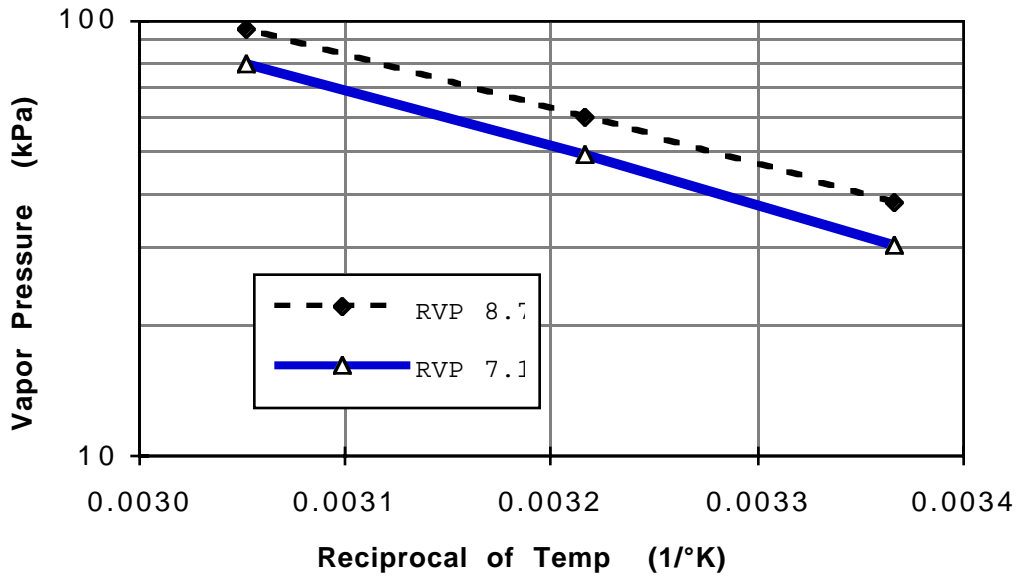
Comparison of Vapor Pressure to Temperature
