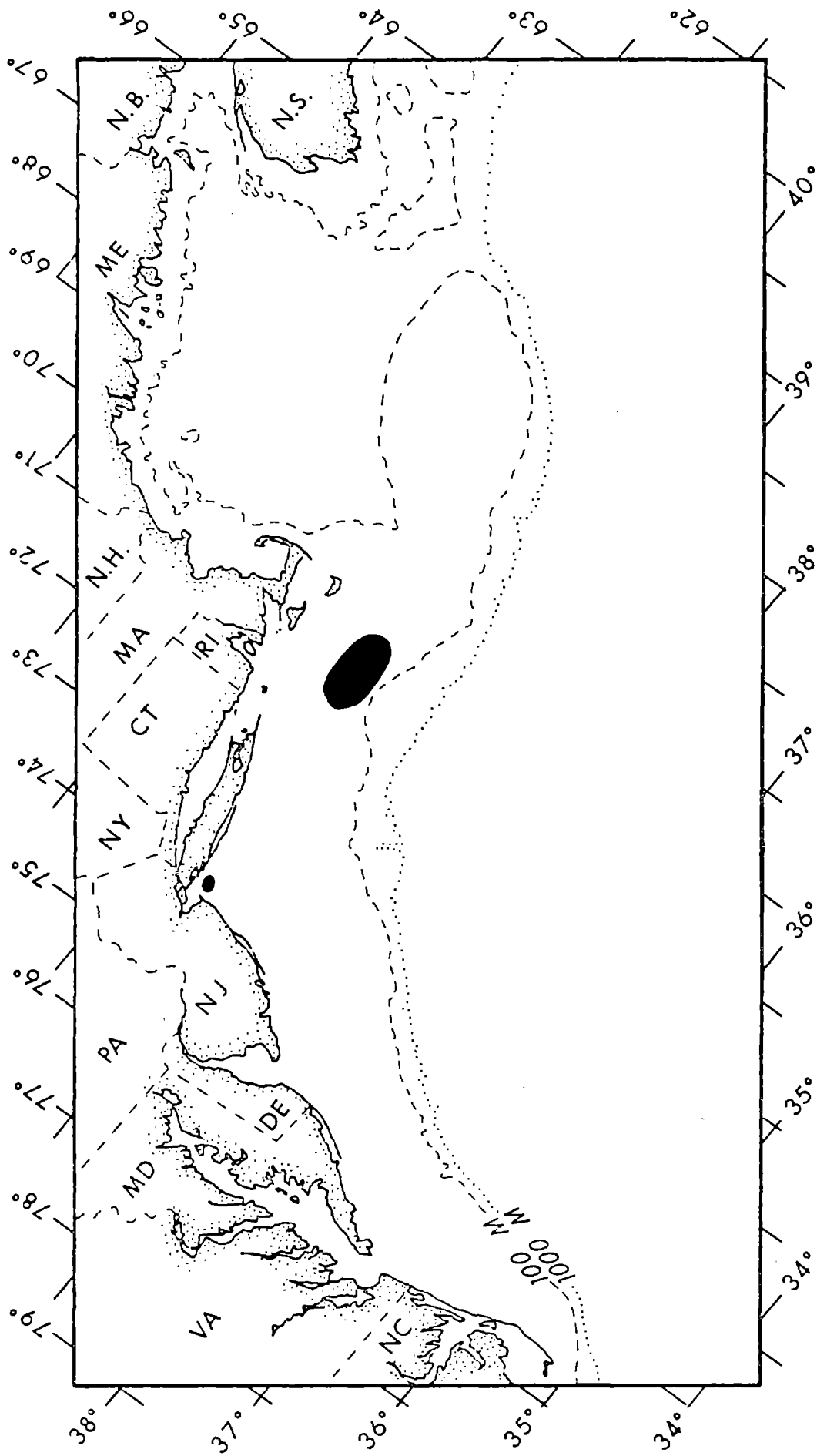
Figure 21. Long-term depositional areas on the continental shelf, excluding submarine canyons.
