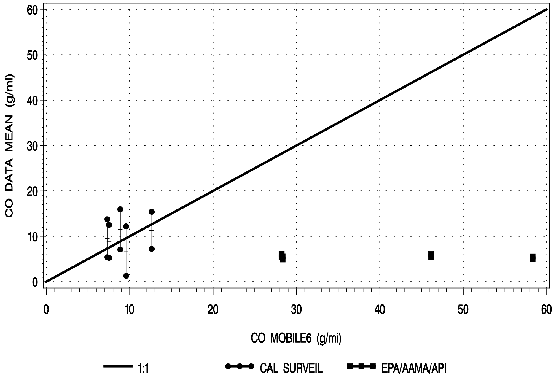
Figure 2: CO COMPARISON OF ACTUAL FTP DATA WITH PROPOSED OHIO-BASED MOBILE6 ESTIMATES 1988-93 TBI TRUCKS: 95% CONFIDENCE INTERVALS
