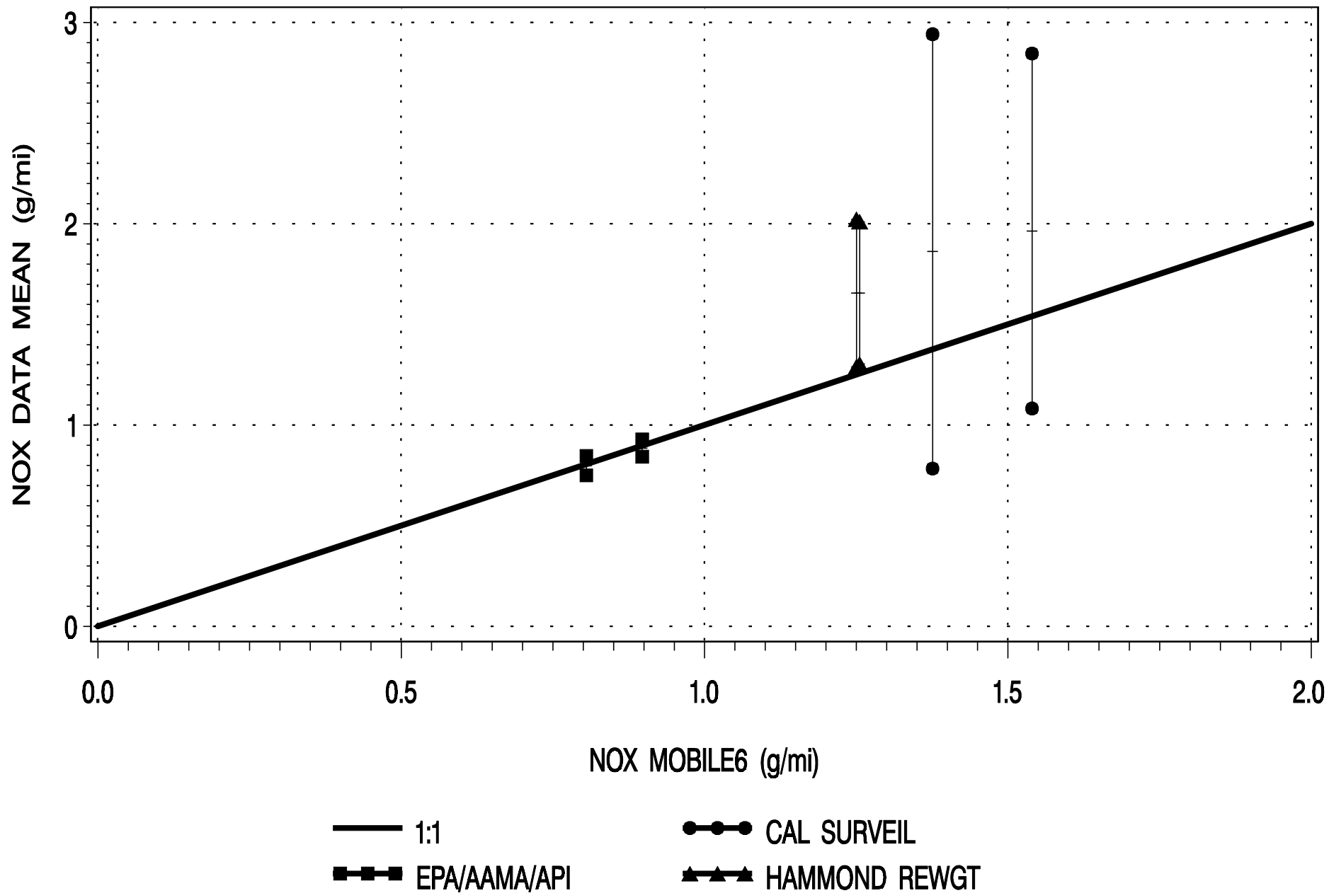
Figure 2: NOX COMPARISON OF ACTUAL FTP DATA WITH PROPOSED OHIO-BASED MOBILE6 ESTIMATES 1981-82 CARB CARS: 95% CONFIDENCE INTERVALS
