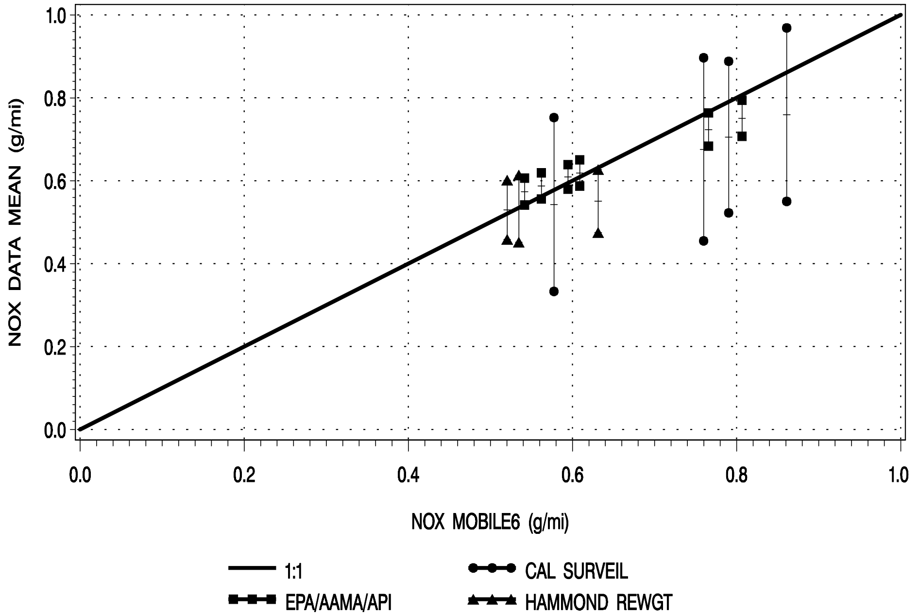
Figure 2: NOX COMPARISON OF ACTUAL FTP DATA WITH PROPOSED OHIO-BASED MOBILE6 ESTIMATES 1988-93 TBI CARS: 95% CONFIDENCE INTERVALS
