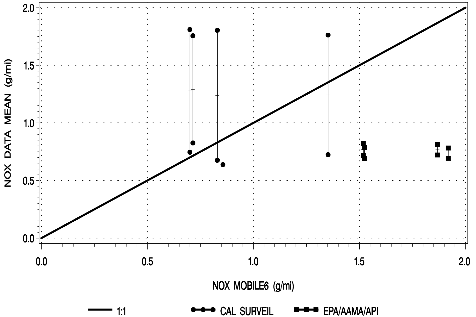
Figure 2: NOX COMPARISON OF ACTUAL FTP DATA WITH PROPOSED OHIO-BASED MOBILE6 ESTIMATES 1988-93 TBI TRUCKS: 95% CONFIDENCE INTERVALS
