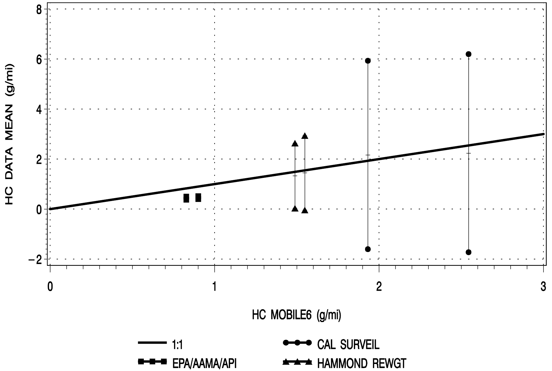
Figure 2: HC COMPARISON OF ACTUAL FTP DATA WITH PROPOSED OHIO-BASED MOBILE6 ESTIMATES 1981-82 FI CARS: 95% CONFIDENCE INTERVALS
