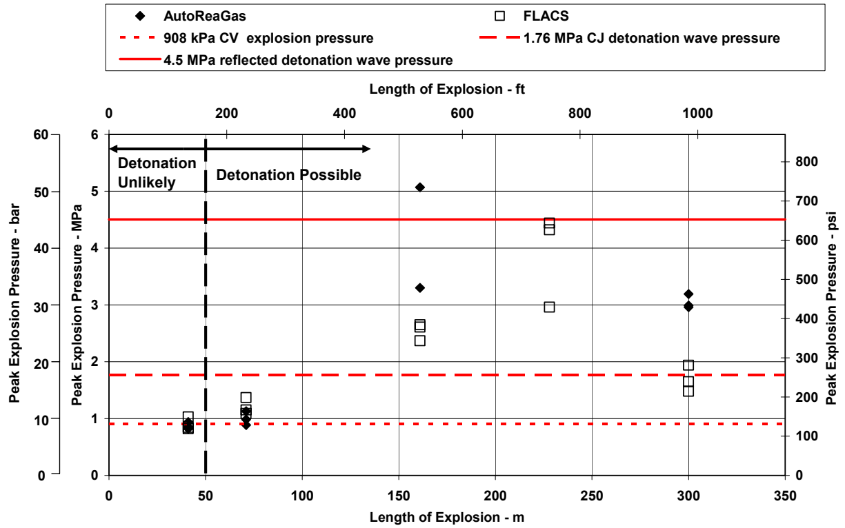
Figure 19.—Peak explosion pressure versus run-up length.
