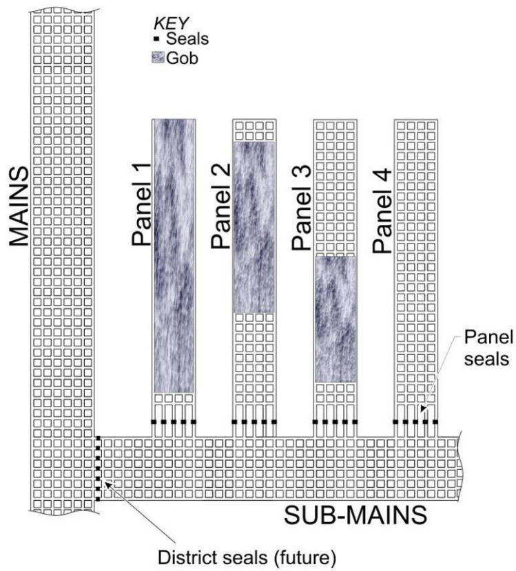
Figure 3.—Typical layout of room-and-pillar mine using bleederless ventilation system. Also shown are typical locations for district and panel seals.
