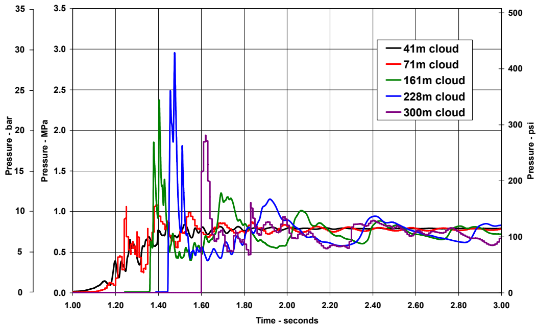
Figure 18.—Calculated pressure-time histories at seal for large-volume explosions using AutoReaGas ( top ) and FLACS ( bottom ).
