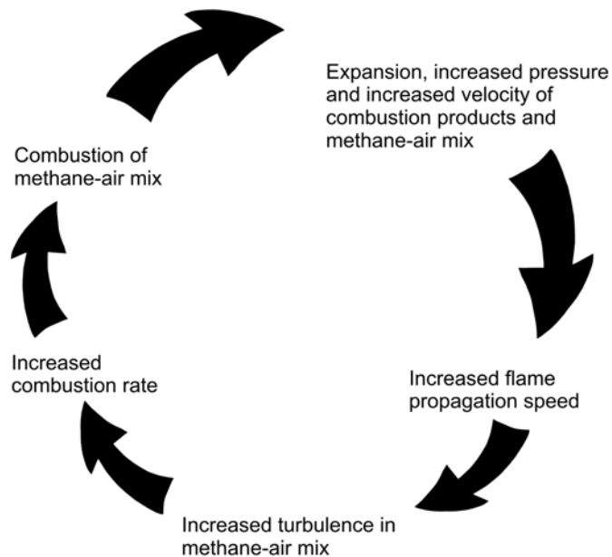
Figure 13.—Strong positive feedback loop between pressure increase, turbulence, and combustion rate.
