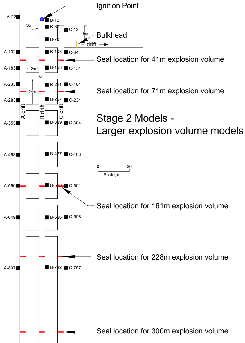
Figure 17.—Layout of large-volume confined explosion models.
