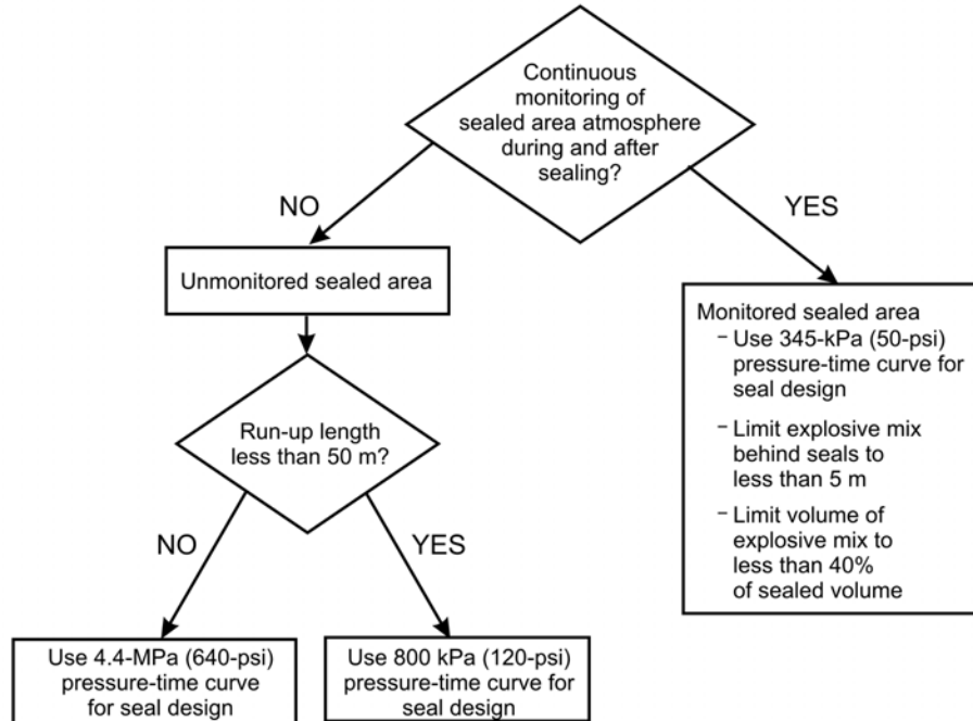
Figure 1.—Flowchart for selecting design pressure-time curve for new seals.
