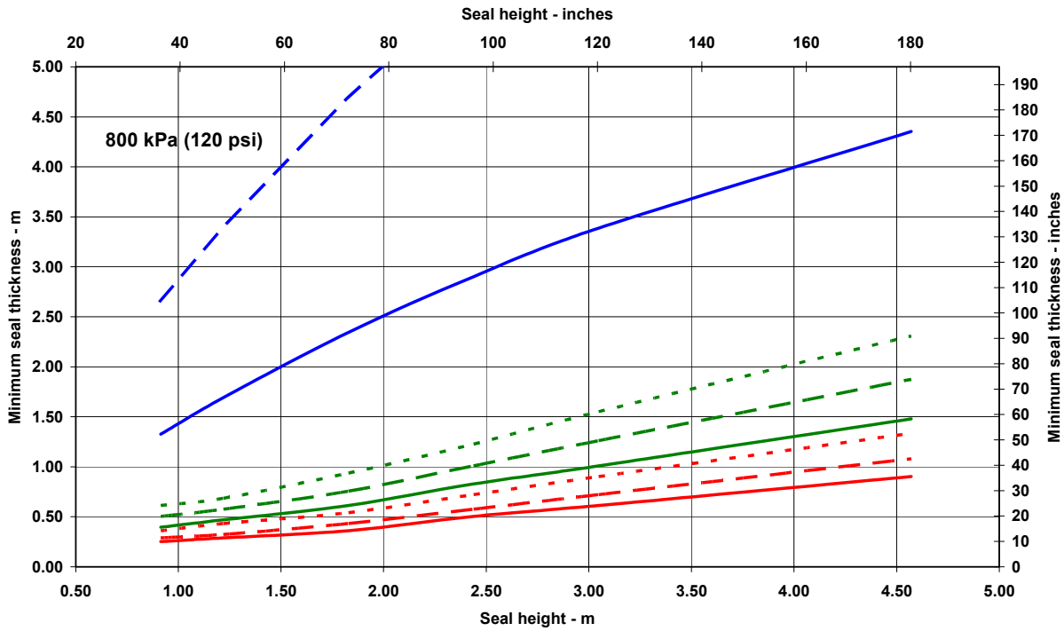
Figure 30.—Design chart for minimum seal thickness with 800-kPa (120-psig) design pressure-time curve using various construction materials. (UCS = uniaxial compressive strength; S.G. = specific gravity.)
