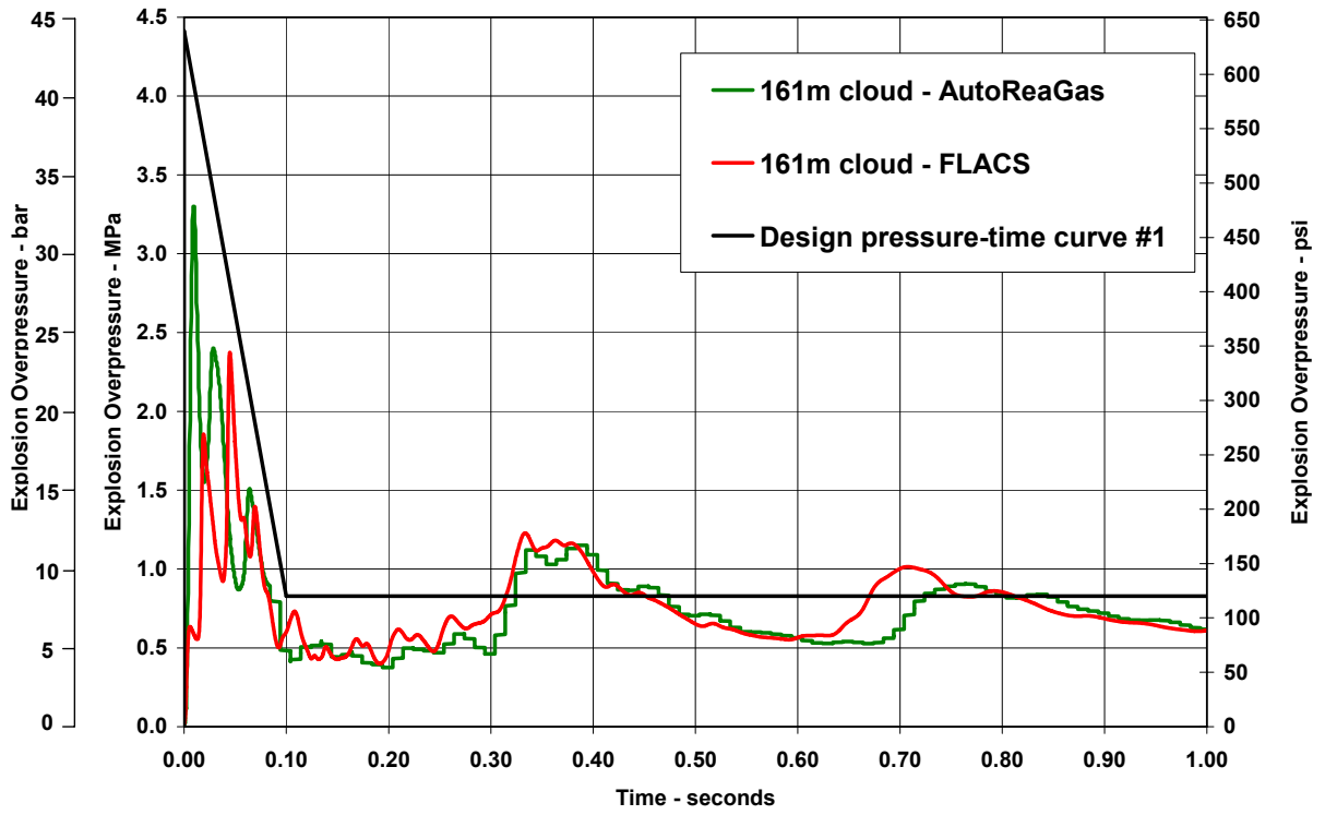
NIOSH Design Pressure-Time Curve #1 - Unlimited, Confined Volume Pressures are Overpressure
