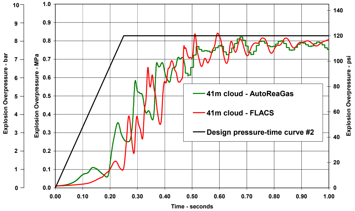
NIOSH Design Pressure-Time Curve #2 - Limited, Confined Volume Pressures are Overpressure
