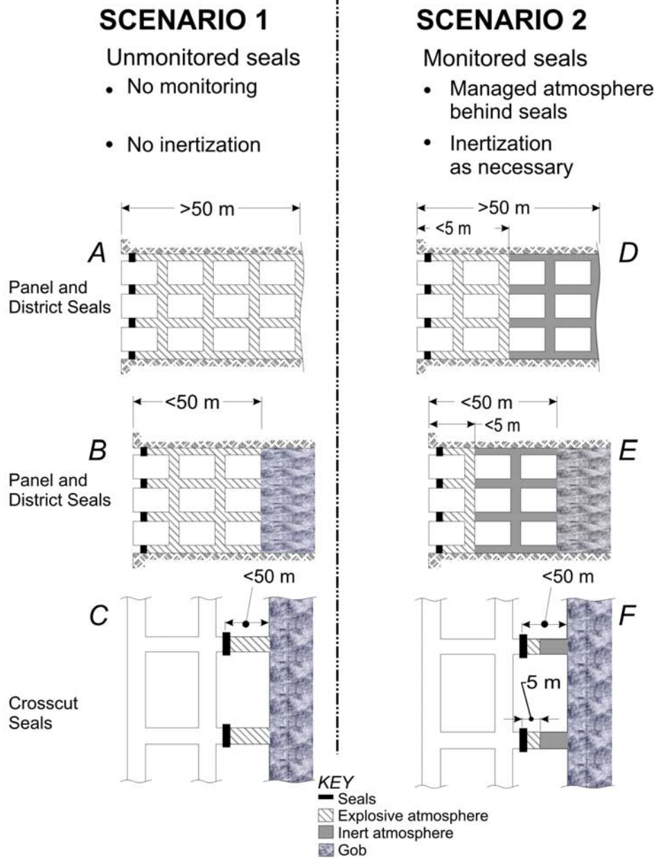
Figure 26.—Illustration of design pressure-time curve application for new seal construction. Scenario 1 depicts unmonitored seals with no monitoring and no inertization. Scenario 2 depicts monitored seals with a managed atmosphere behind the seals and inertization as required. Note that not meeting the requirements for limiting the run-up length, the explosive mix volume, and the venting of a possible explosion or the monitoring criteria necessitates use of the 4.4-MPa (640-psig) design pressure-time curve for seal design. Run-up length is the distance from ignition point to DDT. See section 5.0. For explanation of explosive volume fill, confinement, and venting, see section 3.10.
