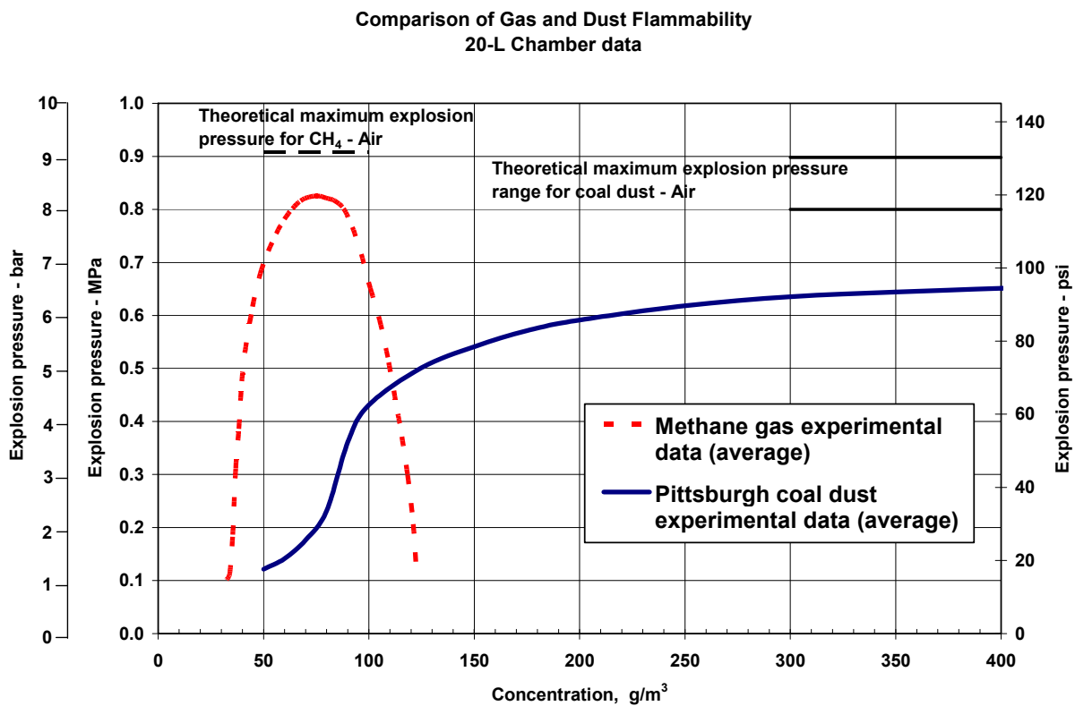
Figure 11.—Variation of absolute pressure for methane-air and coal dust-air [Cashdollar 1996].
