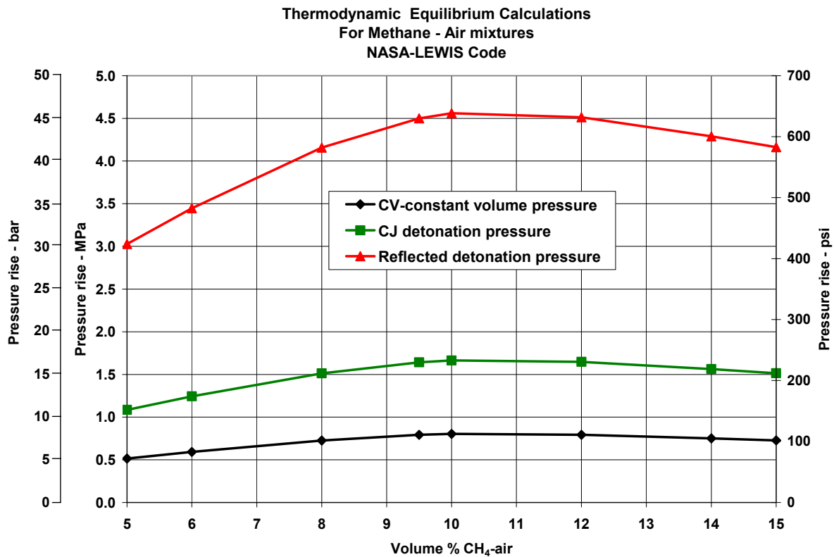
Figure 14.—Variation of theoretical pressure increase ratio versus methane concentration for CV explosion pressure, detonation wave pressure, and reflected detonation wave pressure.
