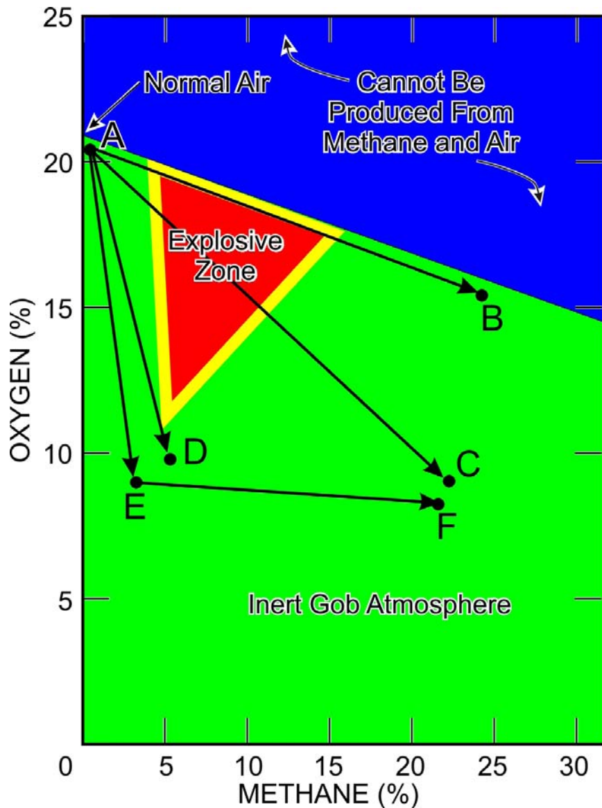
Figure 6.—Coward triangle for explosive zone of methane in air [Coward and Jones 1952]. Also shown are different paths to an inert atmosphere.
