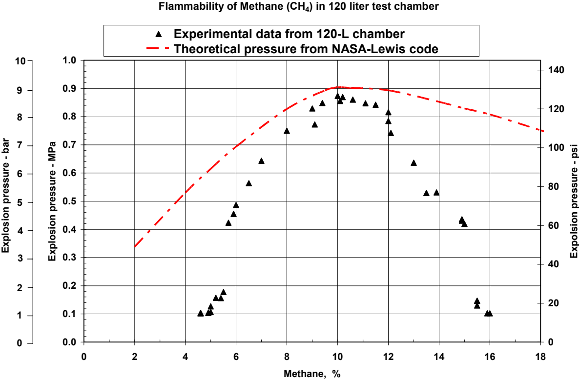
Figure 10.—Variation of absolute pressure versus methane concentration: theoretical and experimental determinations [Cashdollar et al. 2000].
