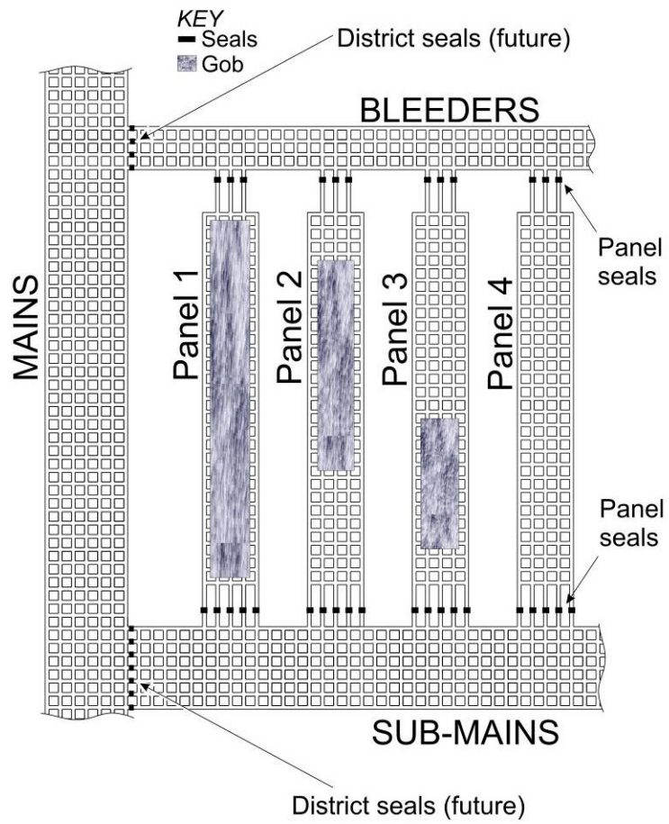
Figure 2.—Typical layout of room-and-pillar mine using bleeders in ventilation system. Also shown are typical locations for district and panel seals.
