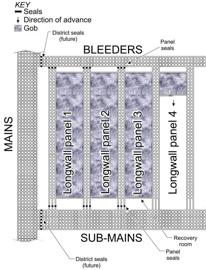
Figure 4.—Typical layout of longwall mining with delayed panel sealing. Also shown are typical locations for district and panel seals.
