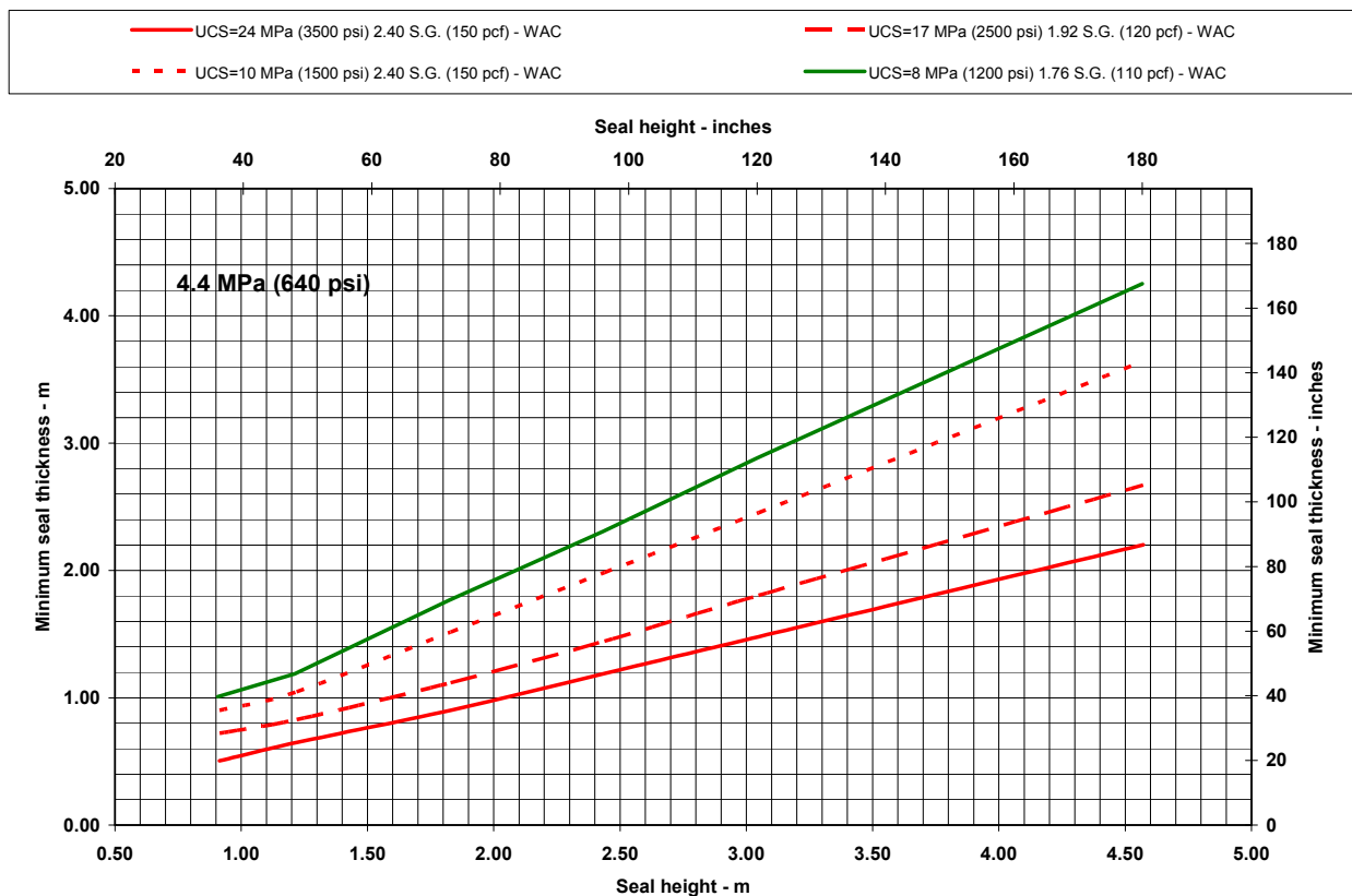
Figure 29.—Design chart for minimum seal thickness with 4.4-MPa (640-psig) design pressure-time curve using various construction materials. (UCS = uniaxial compressive strength; S.G. = specific gravity.)
