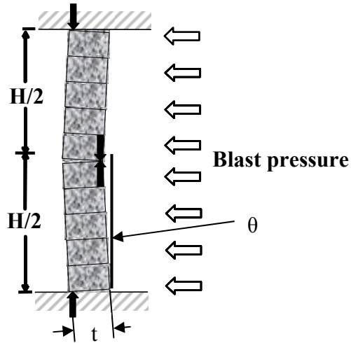
Figure 27.—One-way arching failure mechanism in Wall Analysis Code (WAC).
