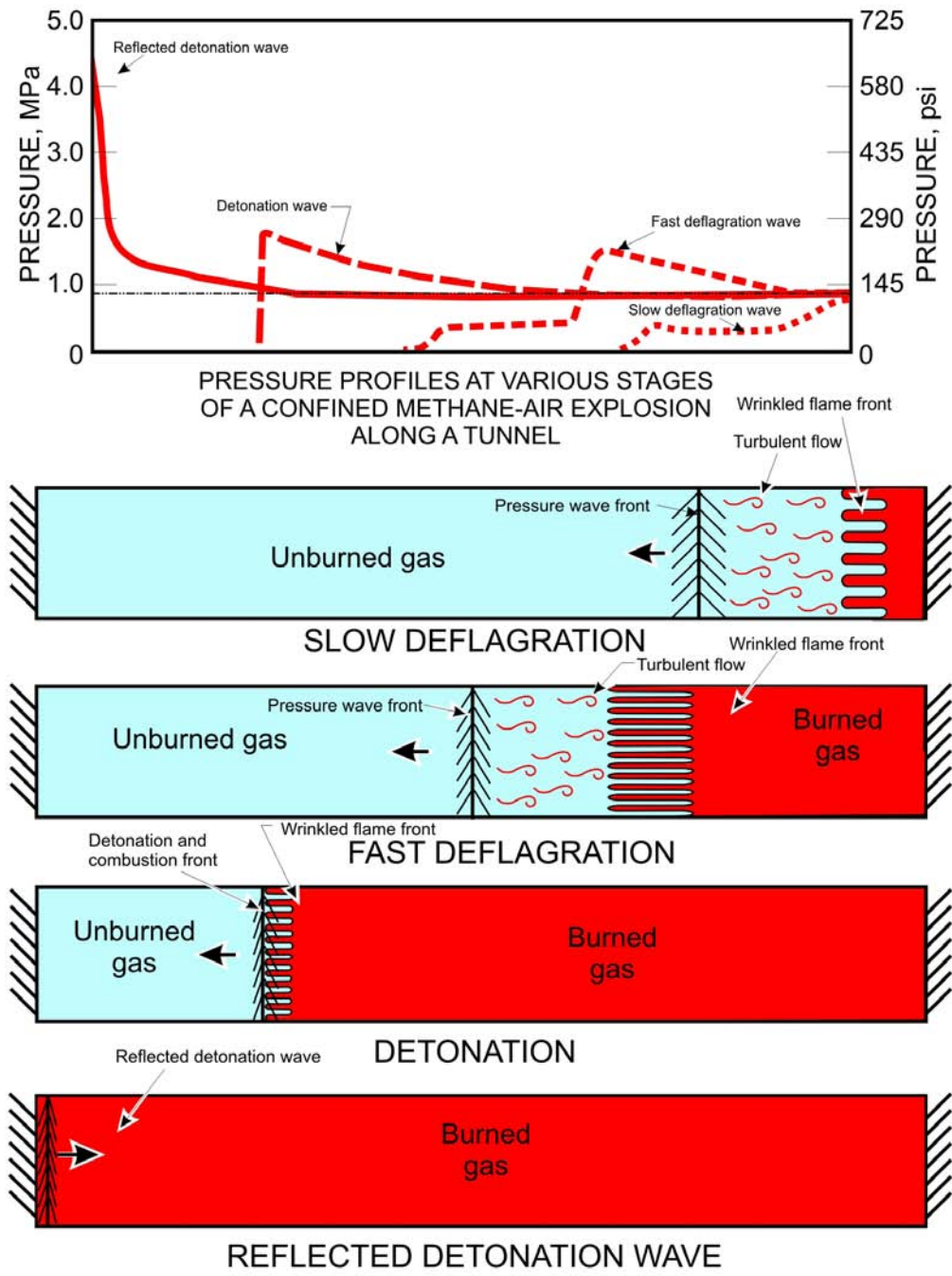
Figure 12.—Four stages of combustion process in a closed tunnel and the approximate pressures.
