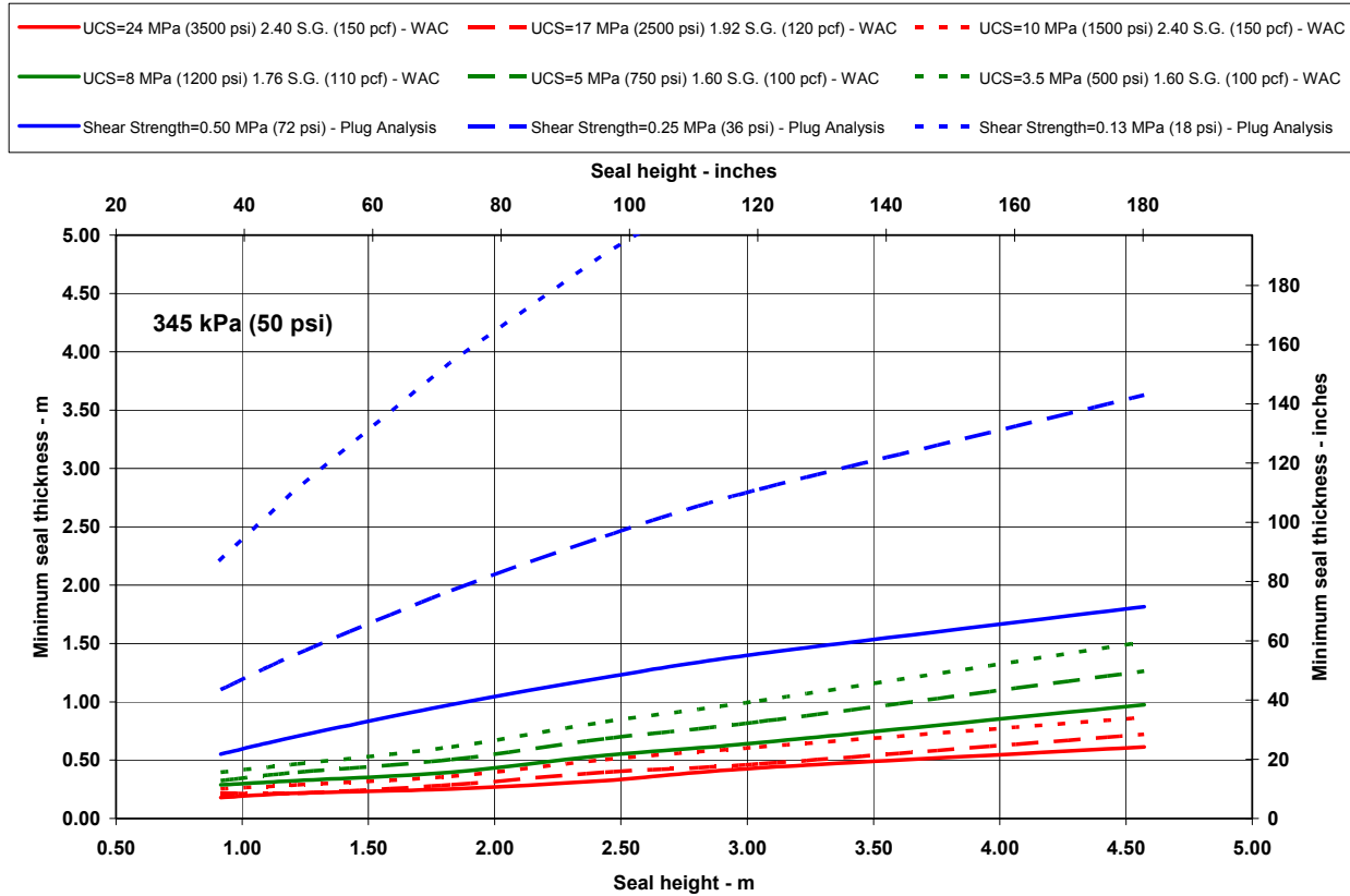
Figure 31.—Design chart for minimum seal thickness with 345-kPa (50-psig) design pressure-time curve using various construction materials. (UCS = uniaxial compressive strength; S.G. = specific gravity.)
