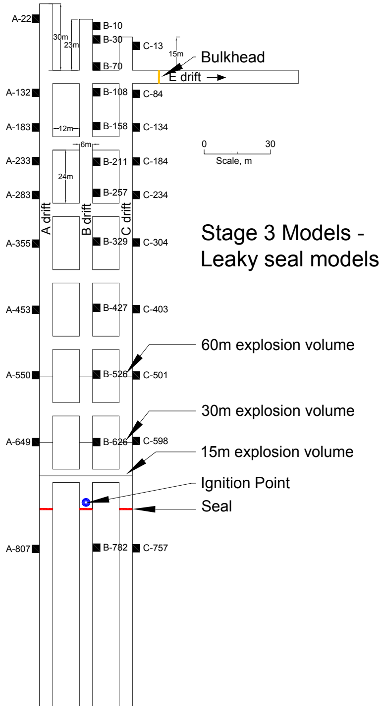
Figure 20.—Layout of partially confined, partially filled explosion models.
