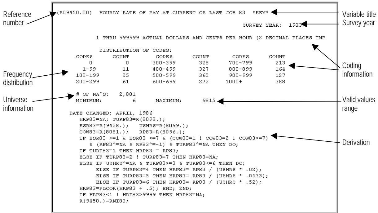
Figure 3.3.1 Sample Created Variable Codeblock
