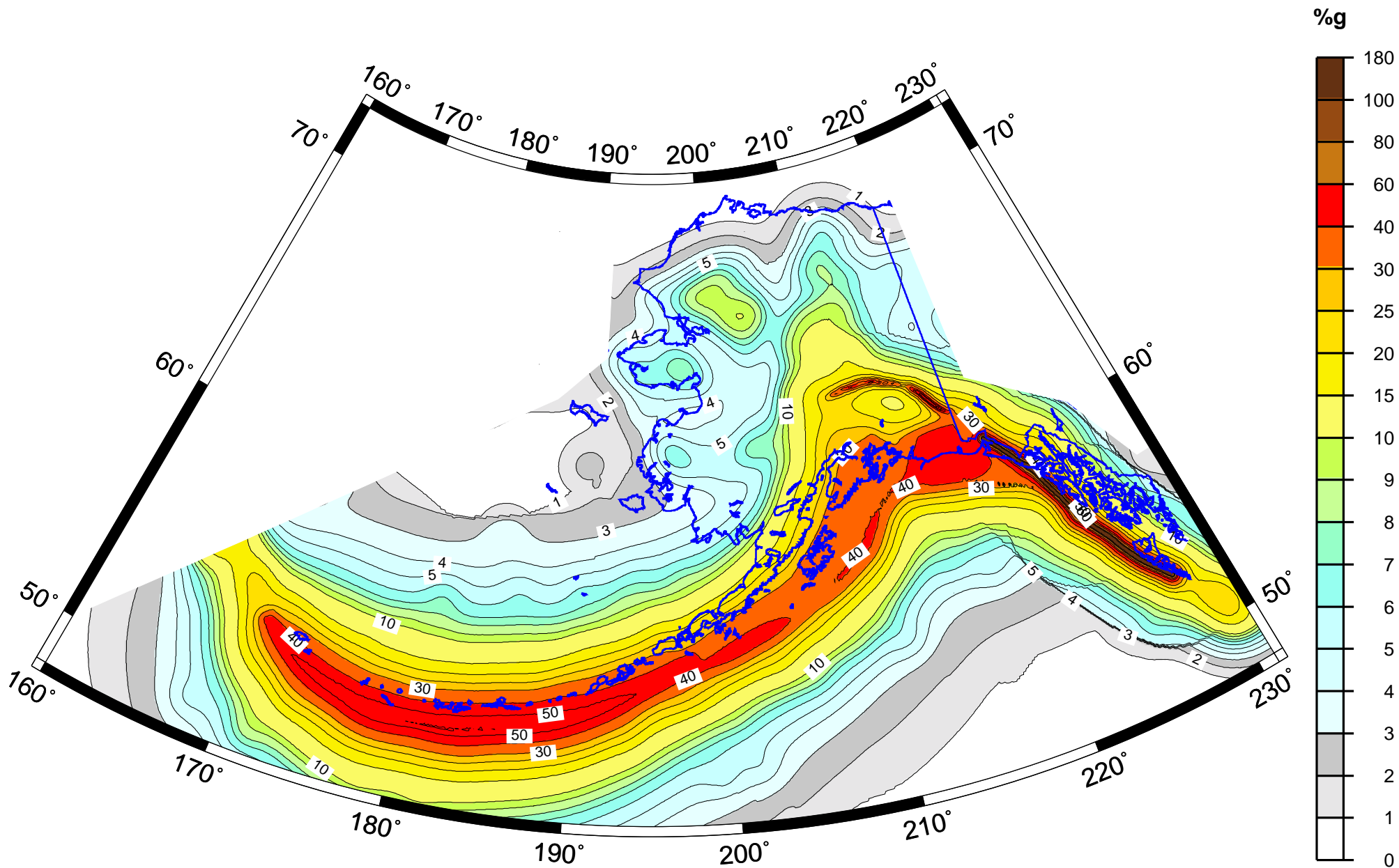
1 Hz Spectral Acceleration (%g) with 10% Probability of Exceedance in 50 Years
