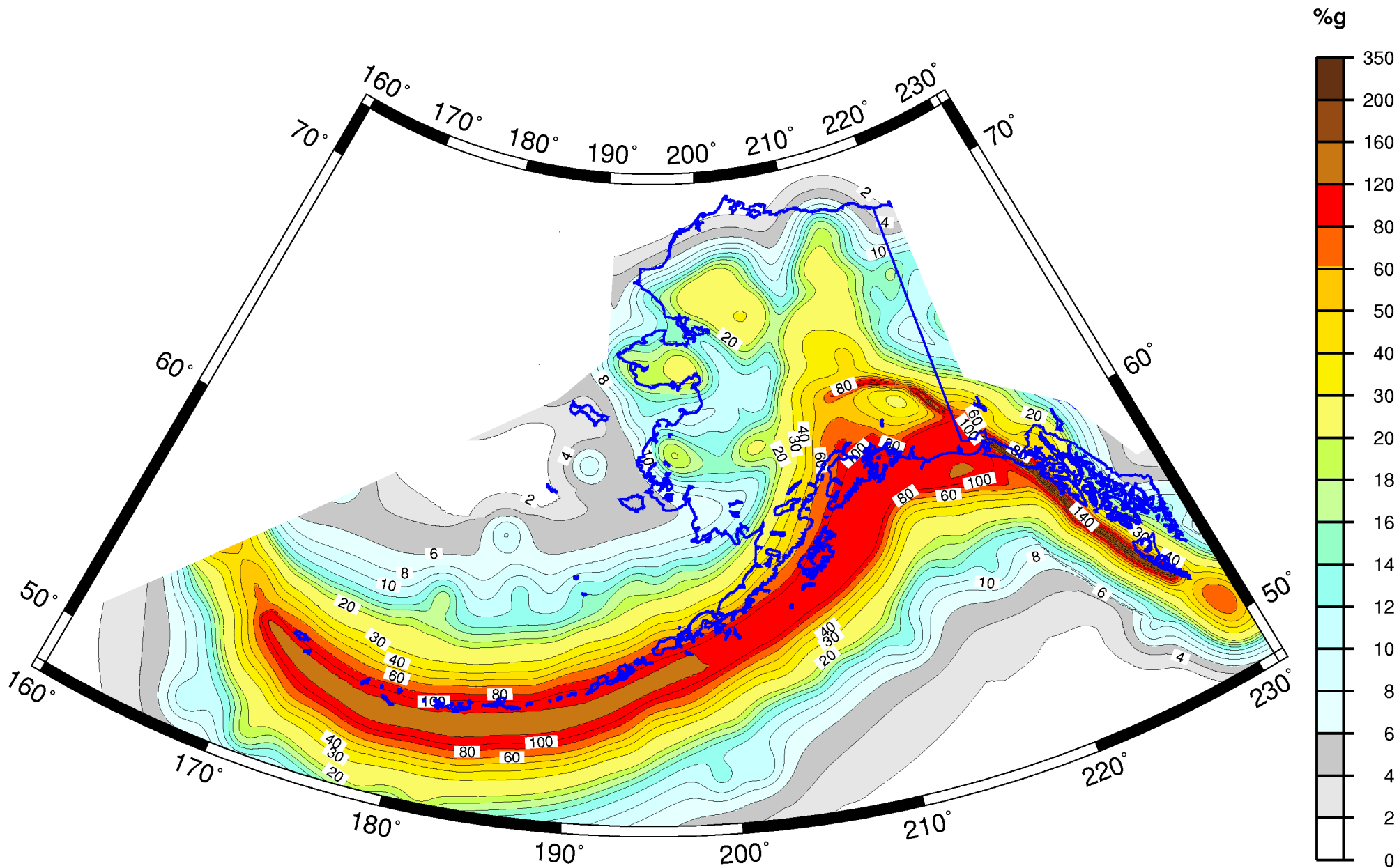
3 Hz Spectral Acceleration (%g) with 10% Probability of Exceedance in 50 Years
