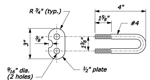
U-BOLT DETAIL
