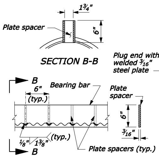
GRATE SLOT
