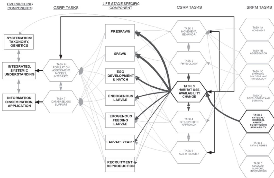
Figure D2. Diagram showing relations of Comprehensive Sturgeon Research Project (CSRП) tasks to life-stage components of pallid sturgeon, and relations of Sturgeon Response to Flow Modification (SRFM) tasks to CSRП. Information flow (curvilinear lines) from task 3 of CSRП (this study) are illustrated with weights commensurate with sequence of emphasis; in the early parts of this project, emphasis has been on prespawning and spawning, but emphasis will shift to larval and juvenile habitats over time. A subset of intertask arrows (rectilinear lines) are shown here, linking task 3 to other CSRП tasks. The double-headed arrows indicate two-way, iterative interaction among tasks, a feature that is essential to developing the comprehensive understanding of factors affecting sturgeon reproduction and survival in the Lower Missouri River.
