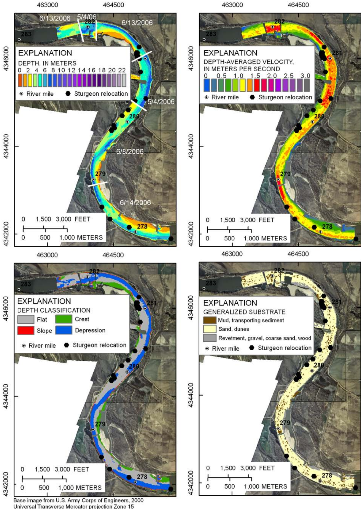
Figure D10. Maps of depth, velocity, terrain classification, and substrate for several reaches at Cranberry Bend, Kansas segment; reaches were mapped at different discharges, ranging from 36,600 ft 3 /s to 65,100 ft 3 /s.
