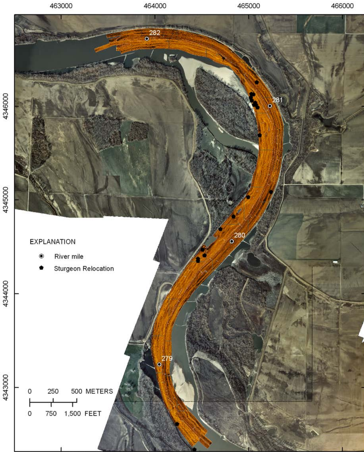
Figure D11. Side-scan sonar imagery for Cranberry Bend, Kansas segment.
