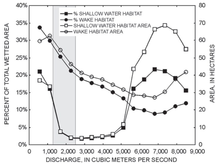
Figure D32. Example of discharge-habitat relations for two physical habitat classes simulated with a multidimensional hydrodynamic model on the Lower Missouri River near Boonville, Mo. (Johnson and others, 2006). The “wake” habitat is defined as regions of high spatial gradients of depth and velocity associated with flow separation.
