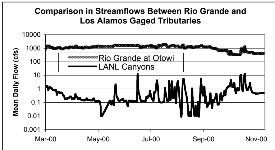
Figure 3. Comparison in streamflows between the Rio Grande at Otowi Bridge and the combined flows from LANL-gauged tributaries during part of CY 2000.
