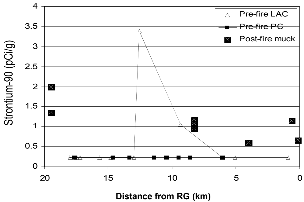
Figure 9. Strontium-90 spatial plot for Los Alamos and Pueblo Canyons sediment concentrations. Pre-fire data from Reneau et al. (1998a, b, and c). LAC = Los Alamos Canyon, PC = Pueblo Canyon, RG = Rio Grande.
