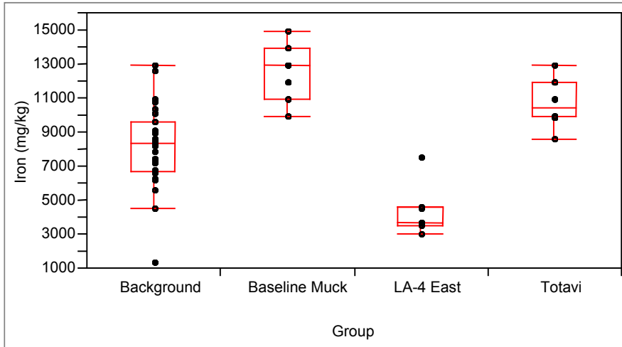
Figure A-16. Box plot for iron.
