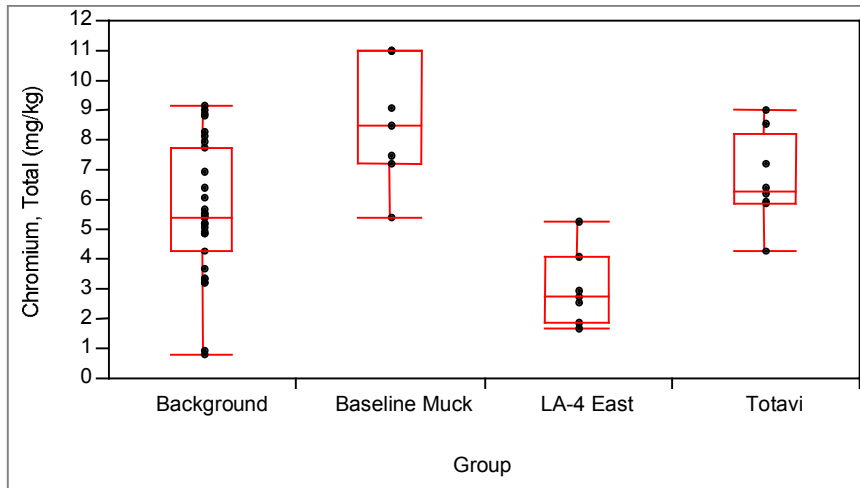
Figure A-13. Box plot for total chromium.
