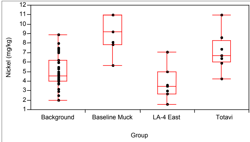
Figure A-21. Box plot for nickel
