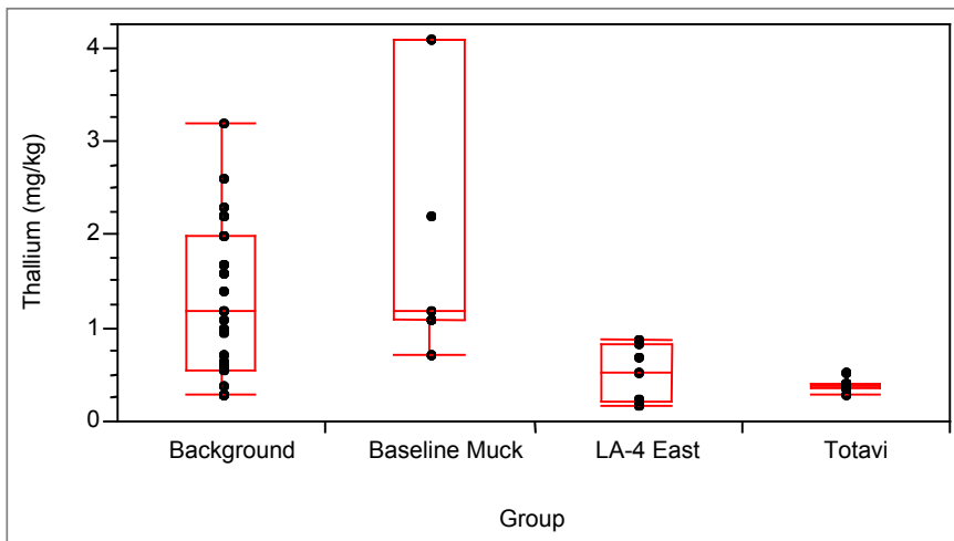
Figure A-26. Box plot for thallium (note that the background data for thallium were obtained from an analytical method with an insufficient detection limit).
