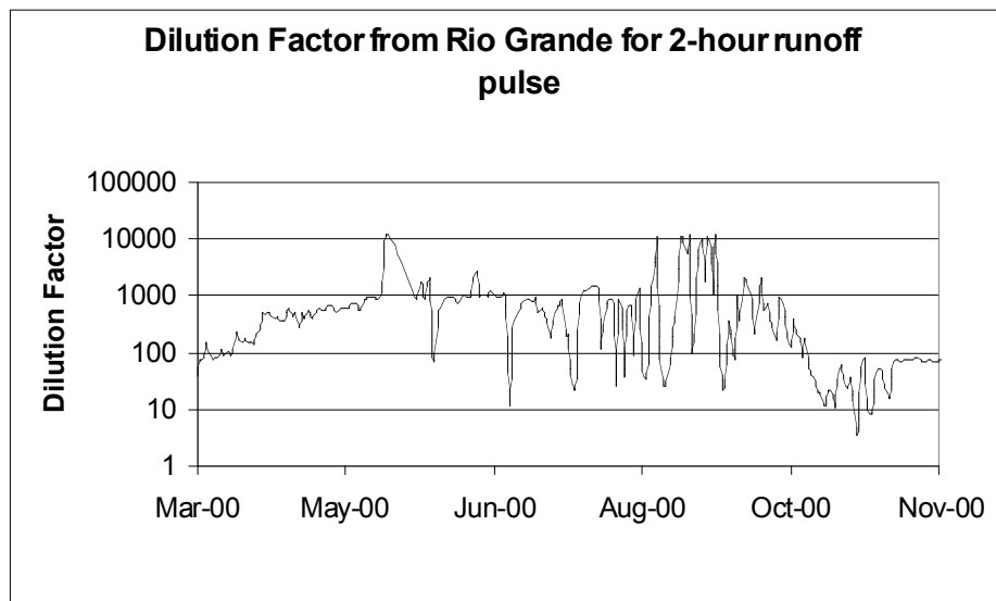
Figure 4. Dilution factors resulting from LANL-canyon runoff mixing with Rio Grande flows over a 2-hour period during part of CY 2000. Minimum dilution occurs on October 23.
