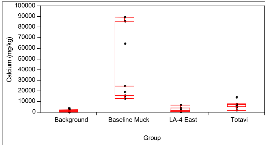
Figure A-12. Box plot for calcium.
