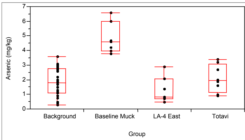
Figure A-8. Box plot for arsenic.
