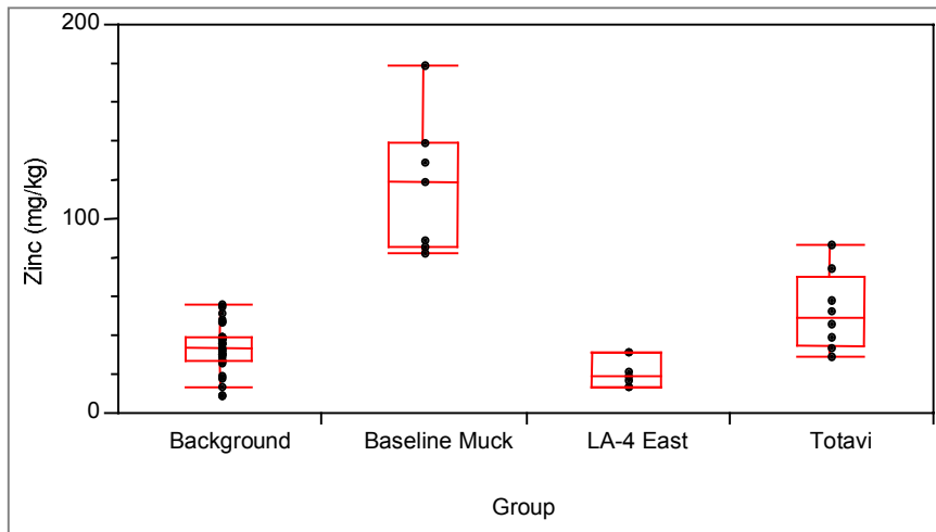
Figure A-28. Box plot for zinc.
