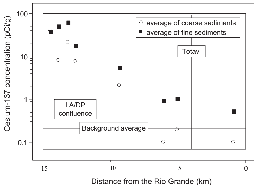
Figure 7. Plot of ^{137}\text{Cs} concentrations by particle size from DP Canyon [the PRS 21-011(k) outfall] to the Rio Grande. Background is the average of coarse- and fine-grained sediments.
