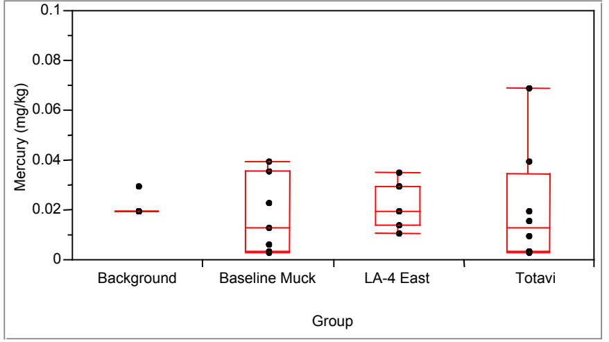
Figure A-20. Box plot for mercury.
