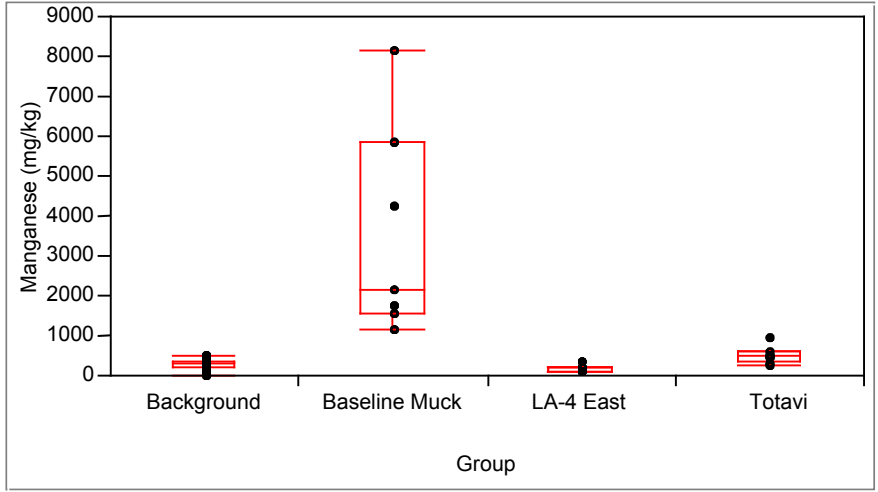
Figure A-19. Box plot for manganese.
