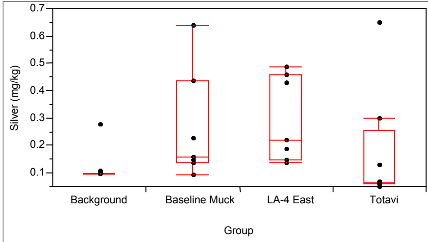
Figure A-24. Box plot for silver.
