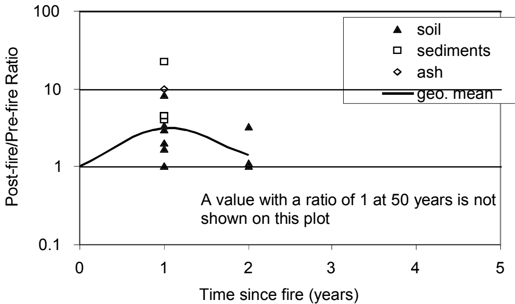
Figure 6. Compilation of changes seen post-fire in various media for metals and radionuclides (studies on nutrients like carbon and nitrogen were excluded from this compilation).
