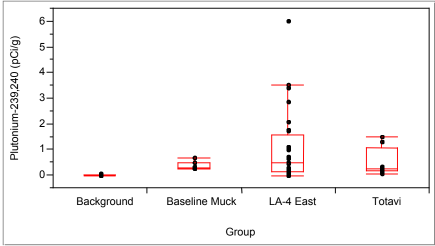
Figure A-4. Box plot for plutonium-239,240
