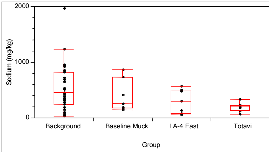
Figure A-25. Box plot for sodium.
