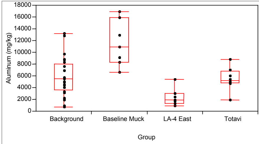
Figure A-6. Box plot for aluminum.
