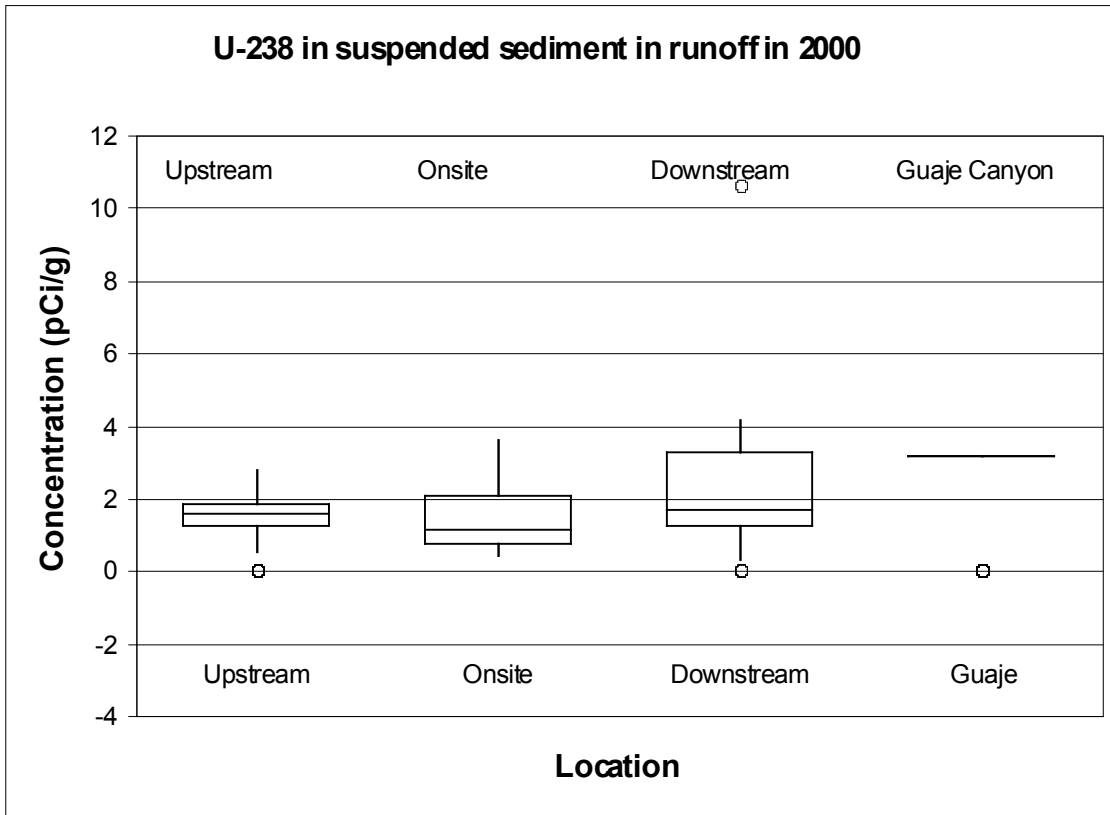
Figure 5. Concentrations of uranium isotopes in suspended sediment carried by runoff in LANL canyons and in Guaje Canyon. These box plots are useful for evaluating differences among groups of data. We use the plots to summarize the distribution of concentrations in sediments in locations upstream (of LANL), LANL onsite, downstream, and at Guaje Canyon for reference. The horizontal line in the middle of the box represents the median concentration. The upper and lower ends of the box delimit the spread of the data by including the middle 50% of the values. Possible statistical outliers are shown with circles.
