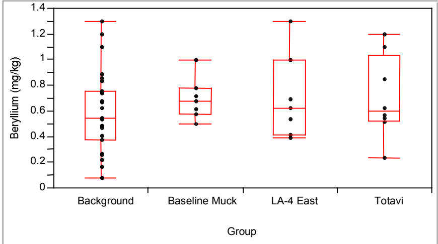
Figure A-10. Box plot for beryllium.
