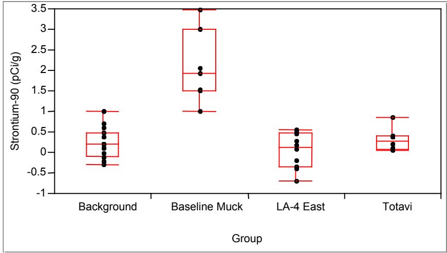
Figure A-5. Box plot for strontium-90
