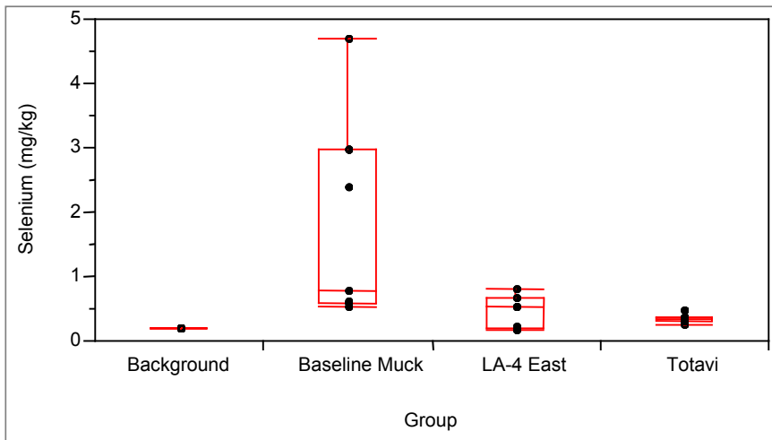
Figure A-23. Box plot for selenium.
