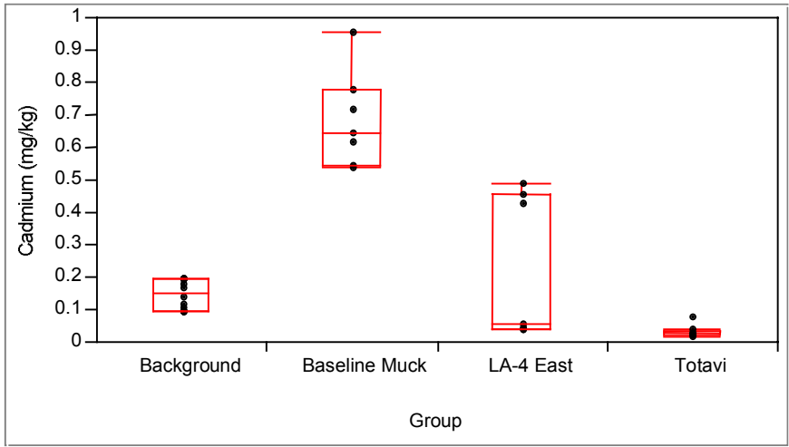
Figure A-11. Box plot for cadmium.
