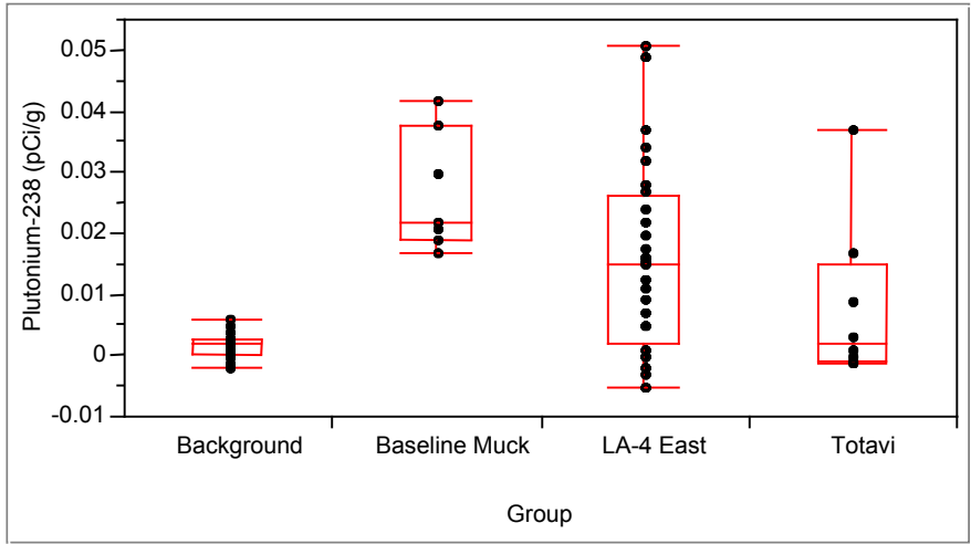
Figure A-3. Box plot for plutonium-238.
