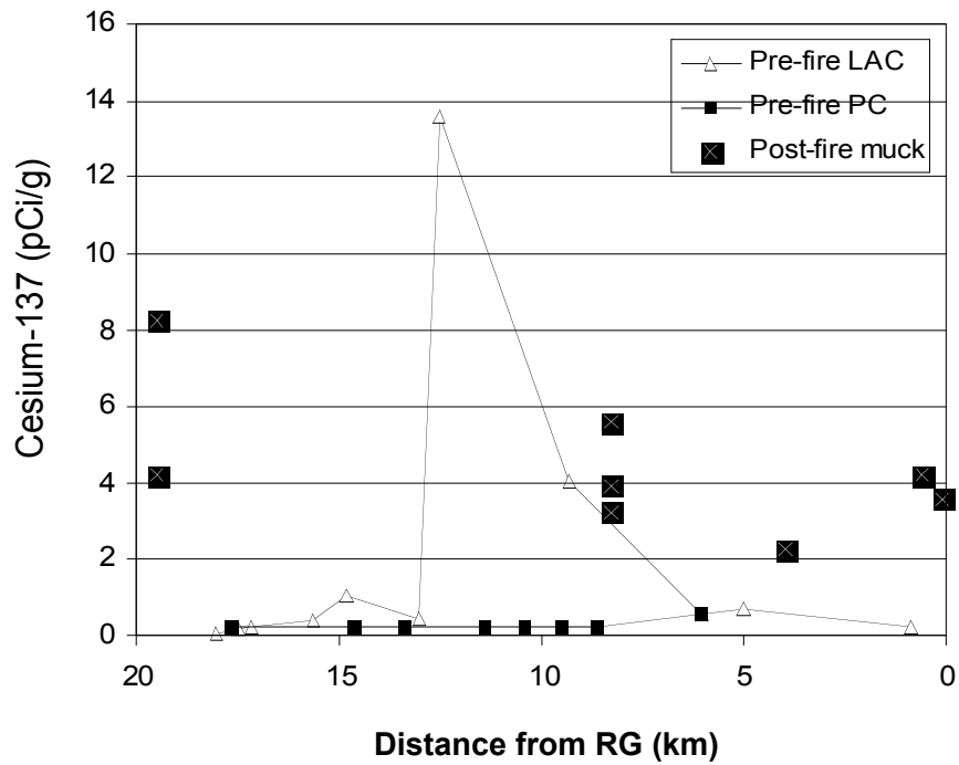
Figure 8. Cesium-137 spatial plot for Los Alamos and Pueblo Canyons sediment concentrations. Pre-fire data from Reneau et al. (1998a, b, and c). LAC = Los Alamos Canyon, PC = Pueblo Canyon, RG = Rio Grande.
