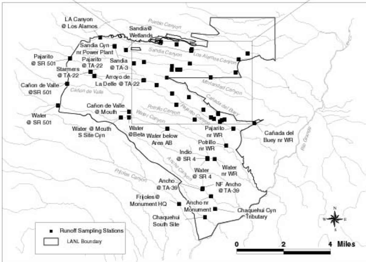
Figure 2. Location map of automated storm water quality sampling stations operated by the Los Alamos National Laboratory.
