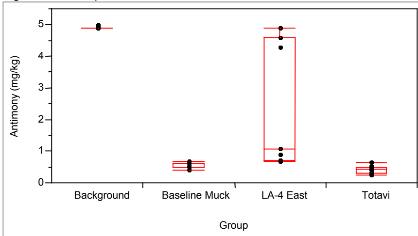
Figure A-7. Box plot for antimony (note that the background data for antimony were obtained from an analytical method with an insufficient detection limit, which is also the case for some results for LA-4 East).
