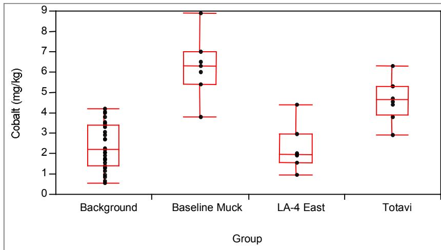
Figure A-14. Box plot for cobalt.
