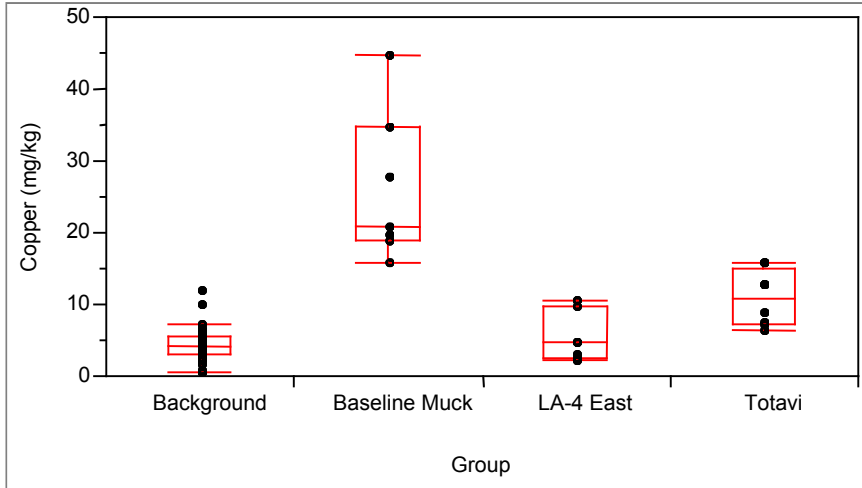
Figure A-15. Box plot for copper.
