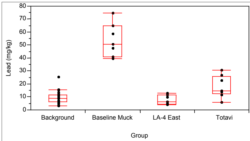
Figure A-17. Box plot for lead.
