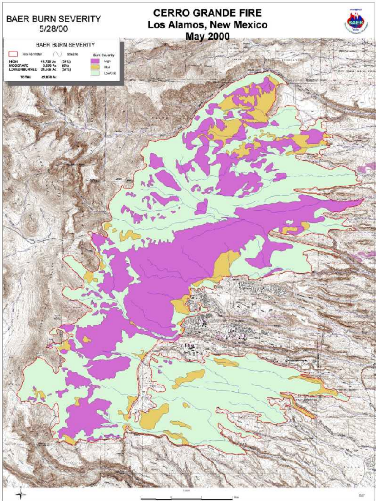
Figure 1. Burn severity and total area burned by the Cerro Grande Fire.
