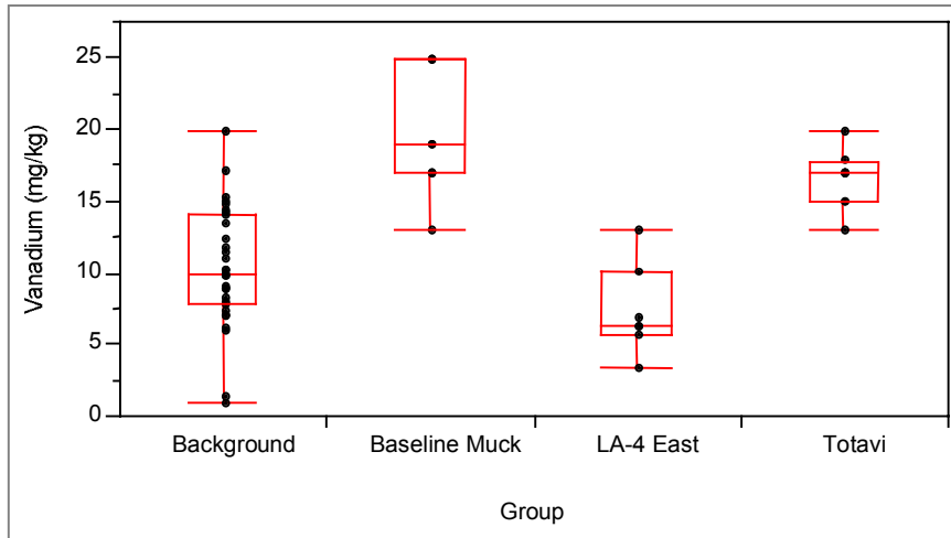
Figure A-27. Box plot for vanadium.
