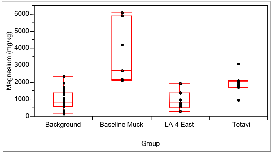
Figure A-18. Box plot for magnesium.
