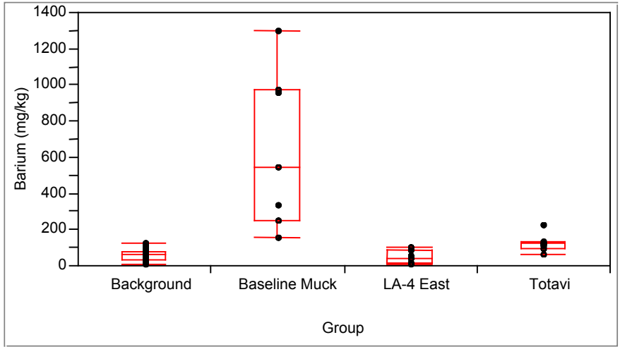
Figure A-9. Box plot for barium.
