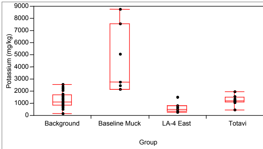
Figure A-22. Box plot for potassium.
