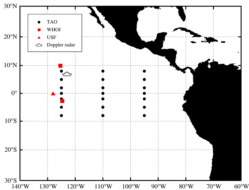
Figure 3.1. Summary of the location of process studies during the pilot phase of PACS. Shipboard studies were done from the R/V Ron Brown in August 1997, and moorings were deployed by the University of South Florida (USF) and the Woods Hole Oceanographic Institution (WHOI) between April 1997 and September 1998. The existing TAO (Tropical Atmosphere Ocean) buoy array is also shown.
