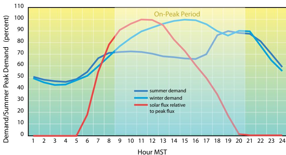
In New Mexico, the amount of electricity generated by a solar panel peaks around noon. (red curve), whereas the demand for electricity peaks closer to 4 p.m. during the summer, 7 p.m. during the winter. Storing the solar-generated electricity would allow the utility to meet demand.
