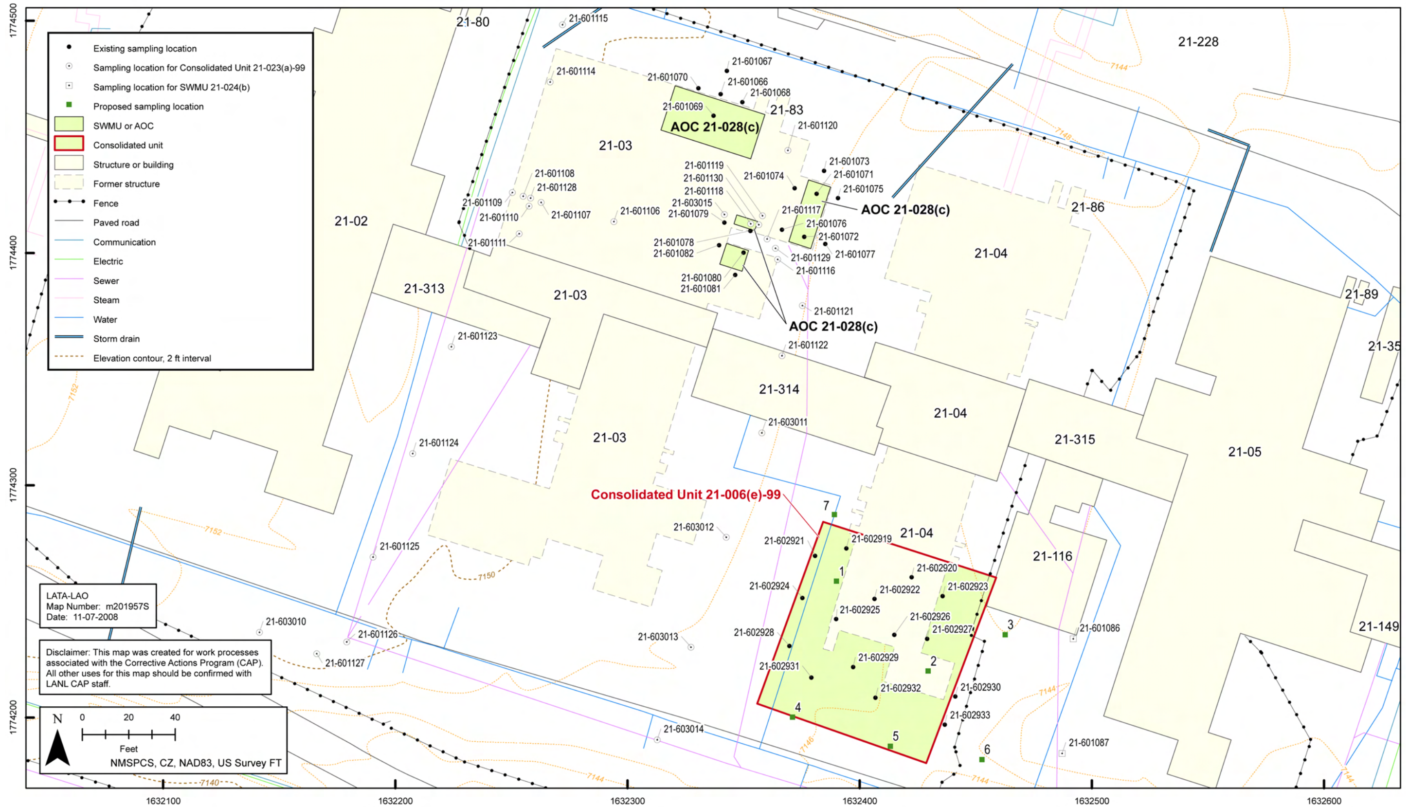
Figure 3.2-1 Proposed sampling locations at Consolidated Unit 21-006(e)-99
