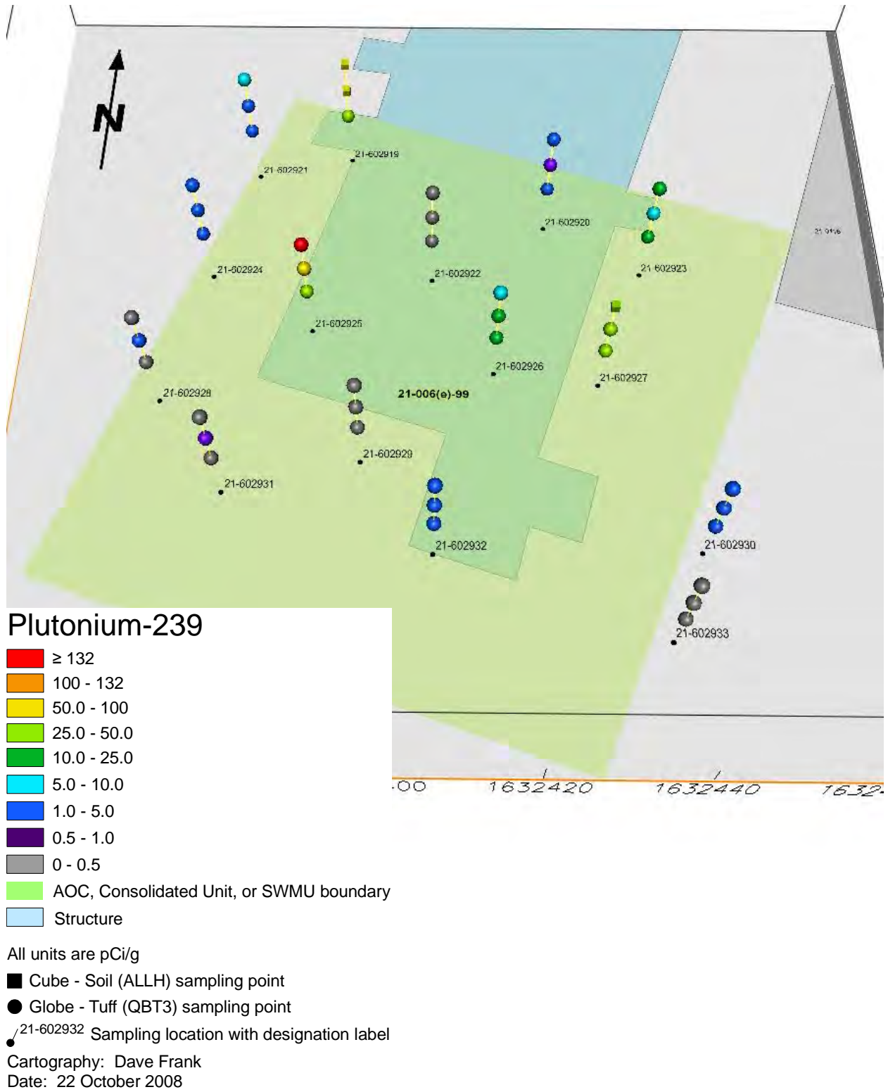
Figure C-5 Distribution of plutonium-239 at Consolidated Unit 21-006(e)-99
