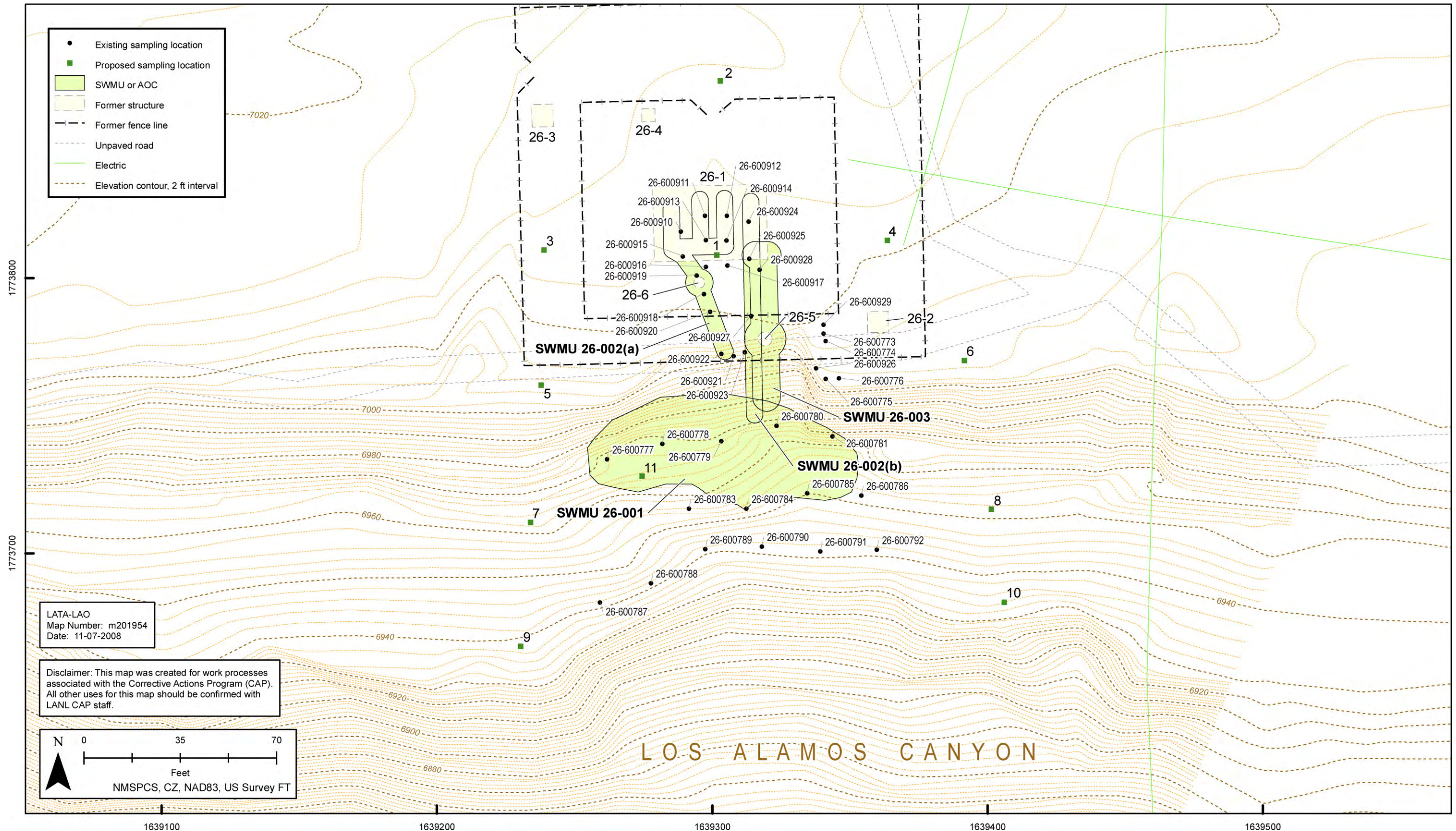
Figure 3.3-1 Proposed sampling locations at TA-26
