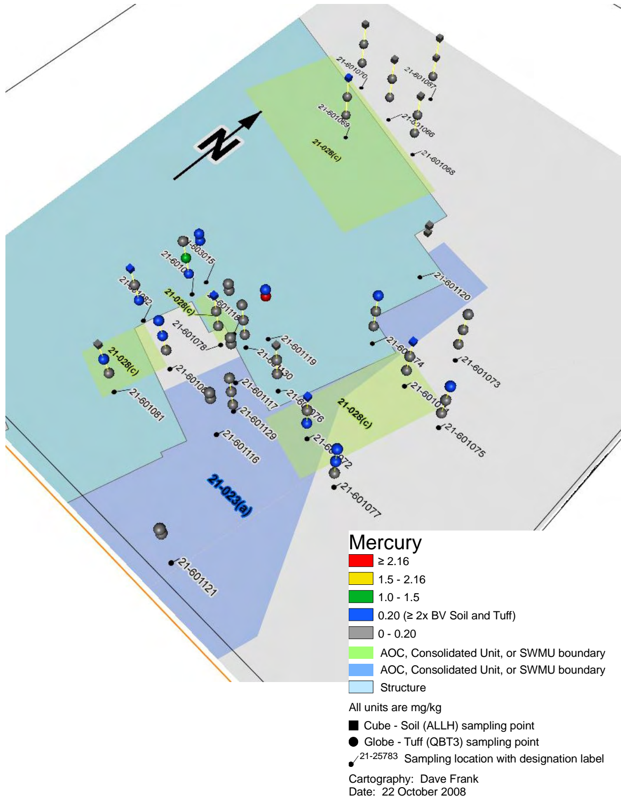
Figure C-12 Distribution of mercury at AOC 21-028(c)
