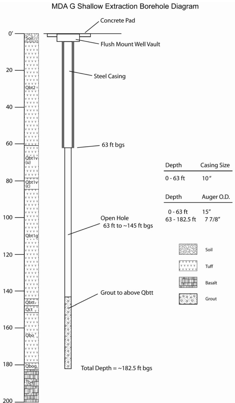
Figure 3.2-2 MDA G shallow-extraction borehole completion diagram
