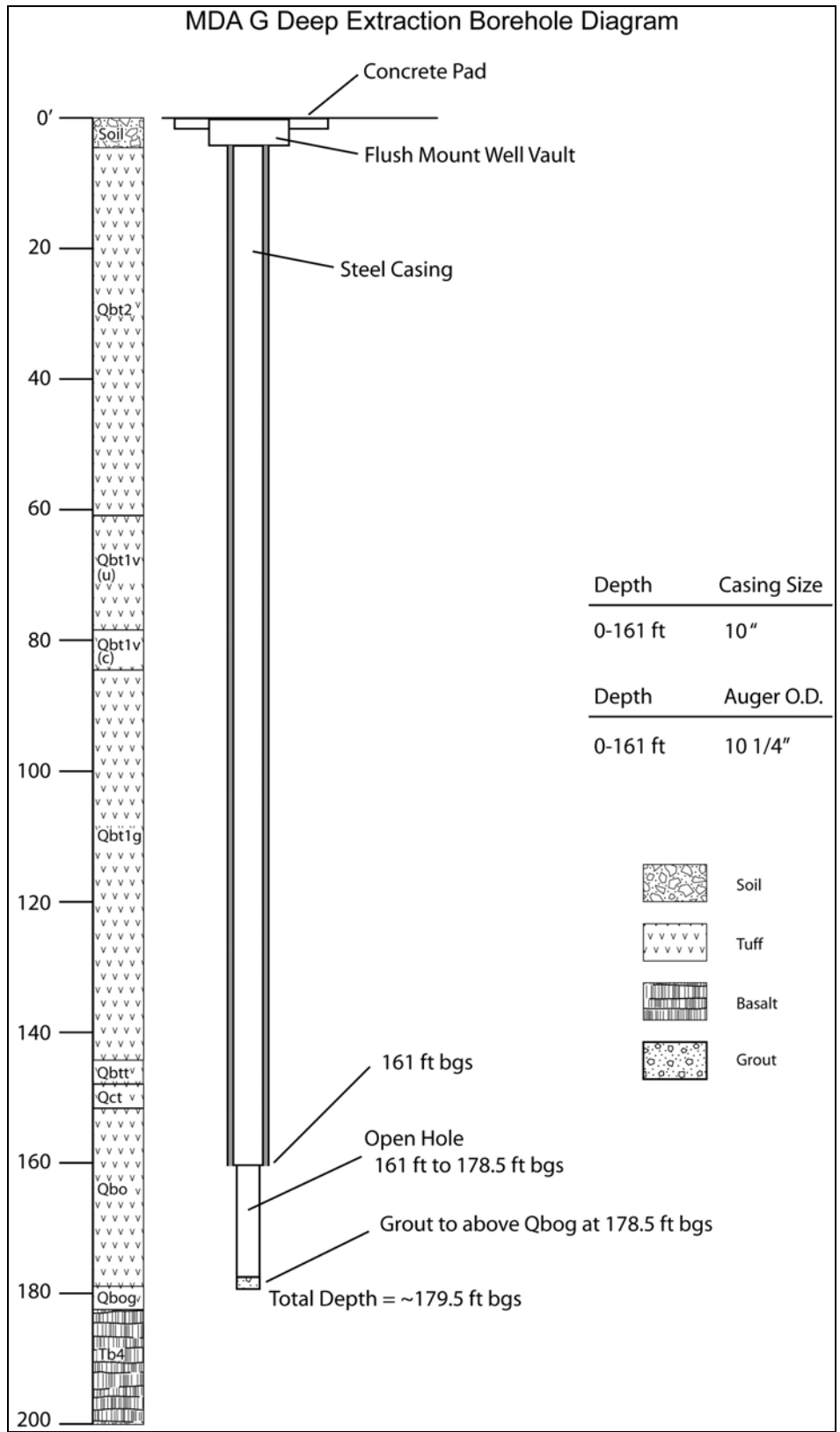
Figure 13 MDA G deep-extraction borehole
