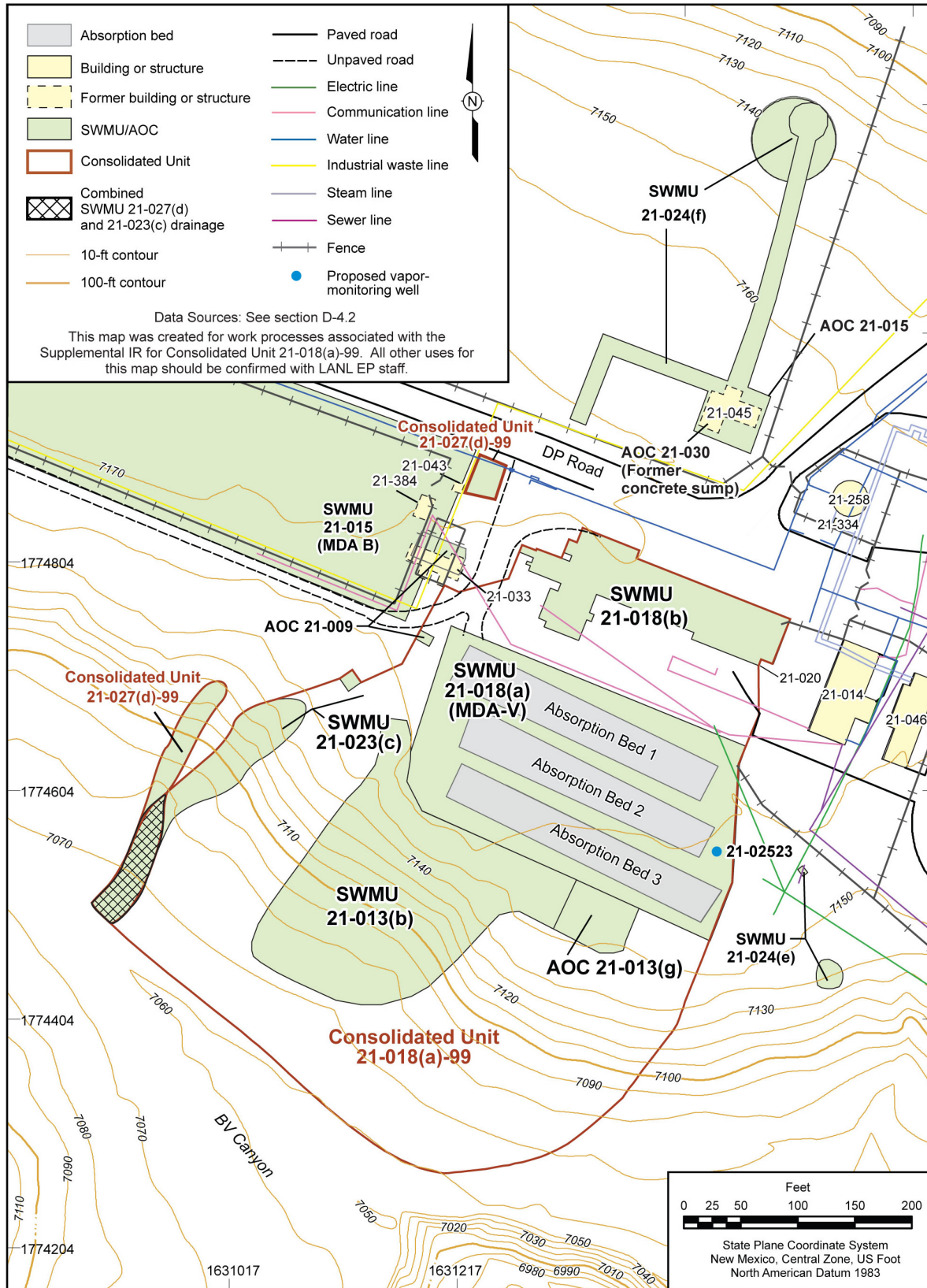
Figure D-3.1-1 Proposed vapor-monitoring well location
