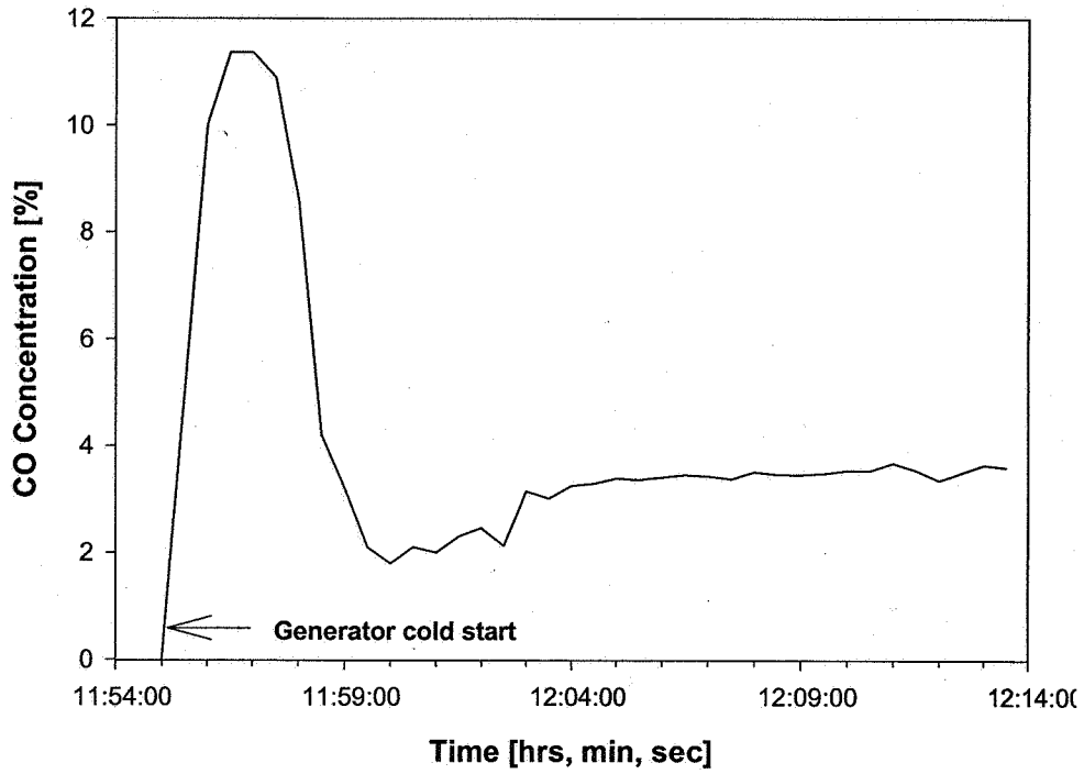
Figure 12. Cold-start data on Houseboat 22 with ECD.
