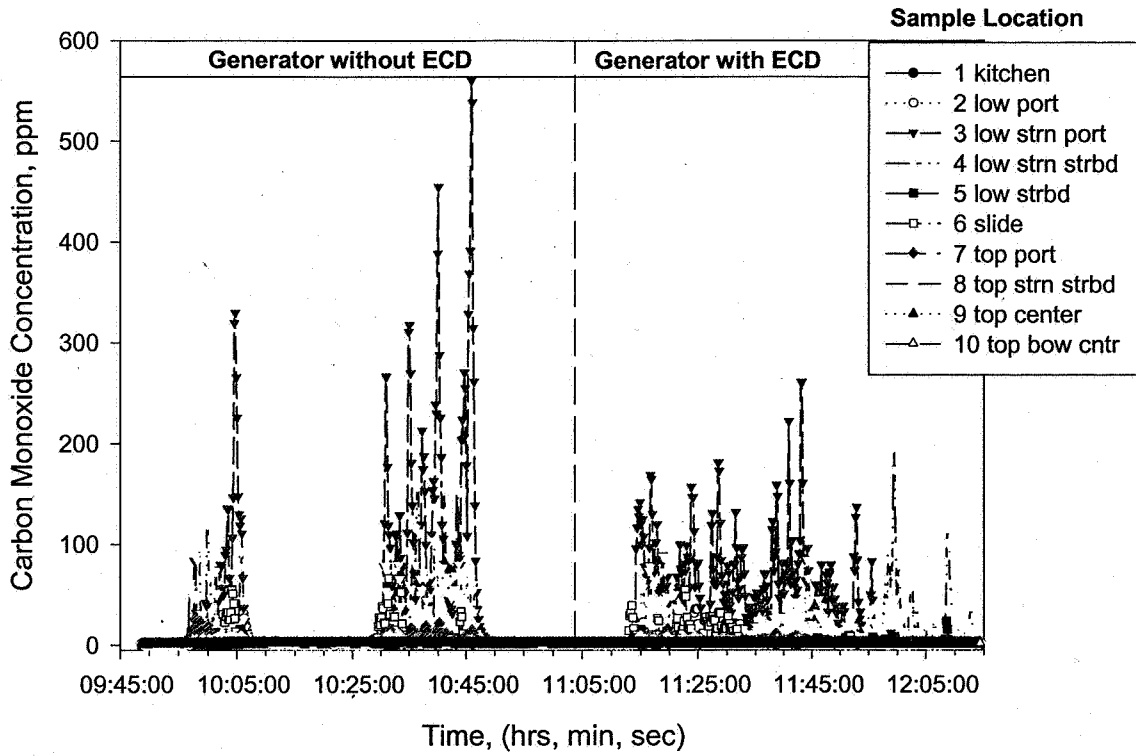
Figure 10. CO sampling on houseboat #22 showing degradation in the ECD's performance (Wed, 10/2).
