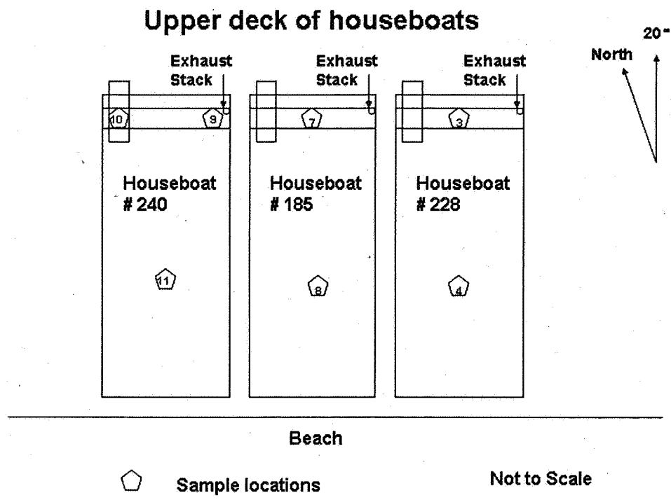
Figure 7. Sampling locations on boats evaluated Tuesday afternoon (Upper deck)
