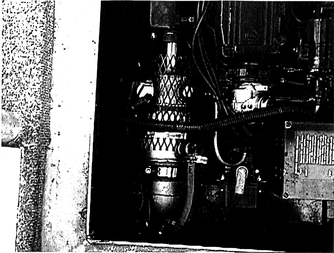
Figure 2. Production ECD with heat shield attached to Westerbeke generator. Note that this ECD has a thermocouple installed to shut off the generator if the temperatures gets too high.
