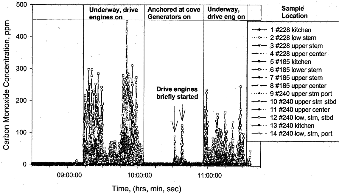
Figure 9. Comparison of CO concentrations with 3 houseboats with vertical exhaust stacks underway and 3 houseboats tied together and stationary. (Tues. aft. 10/1)
