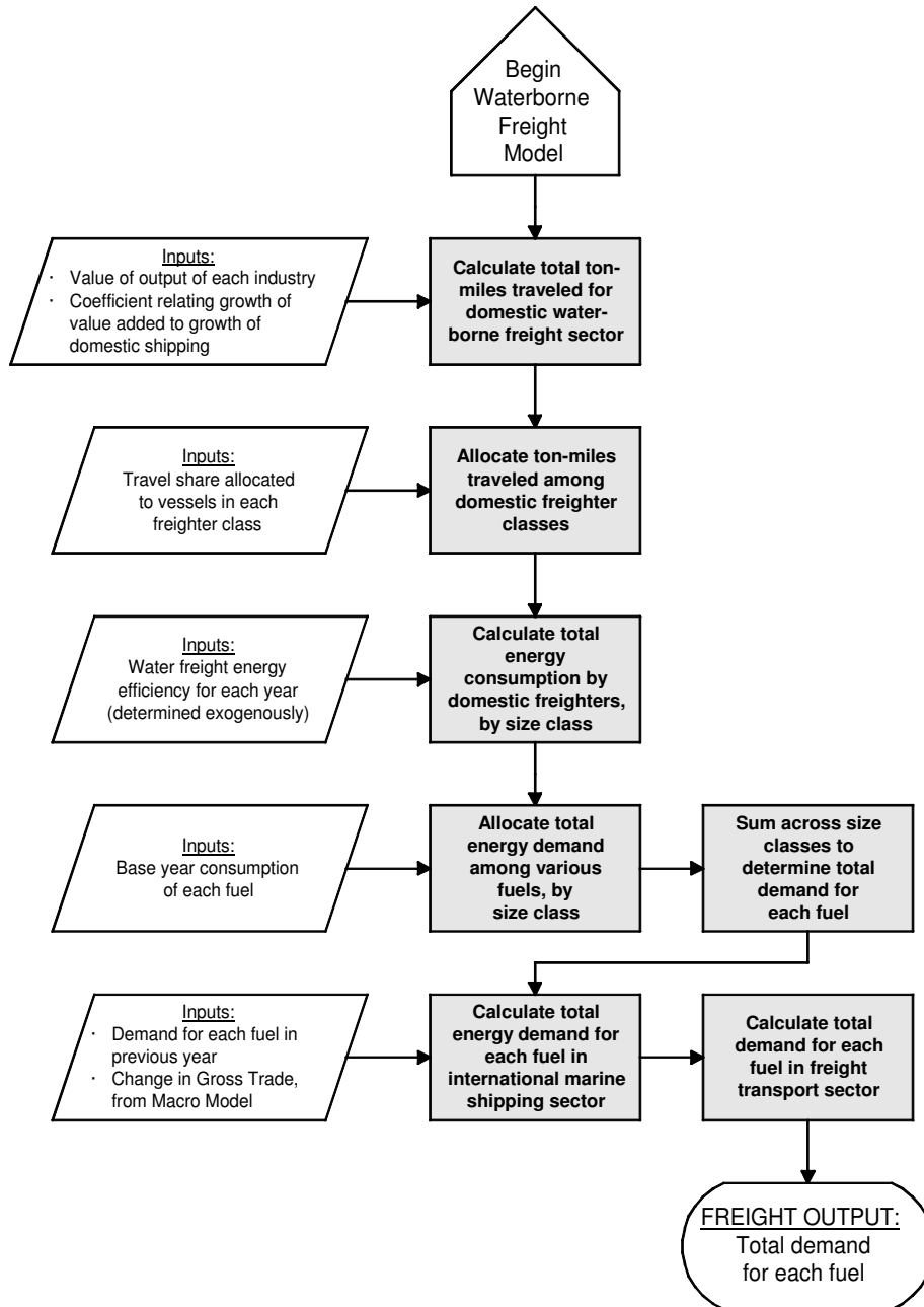
Figure 16. Waterborne Freight Module
