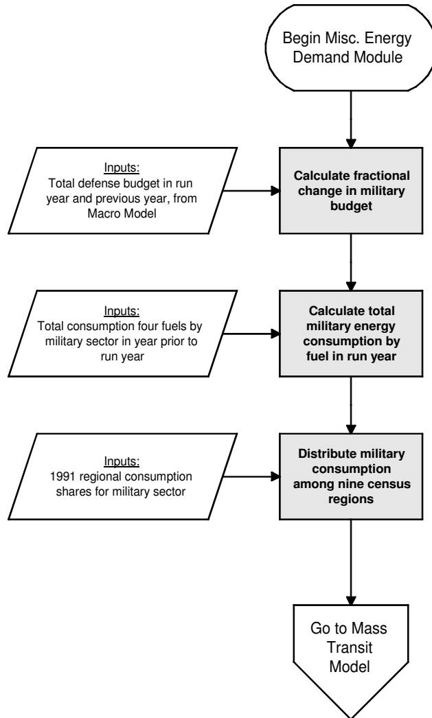
Figure 18. Military Demand Module
