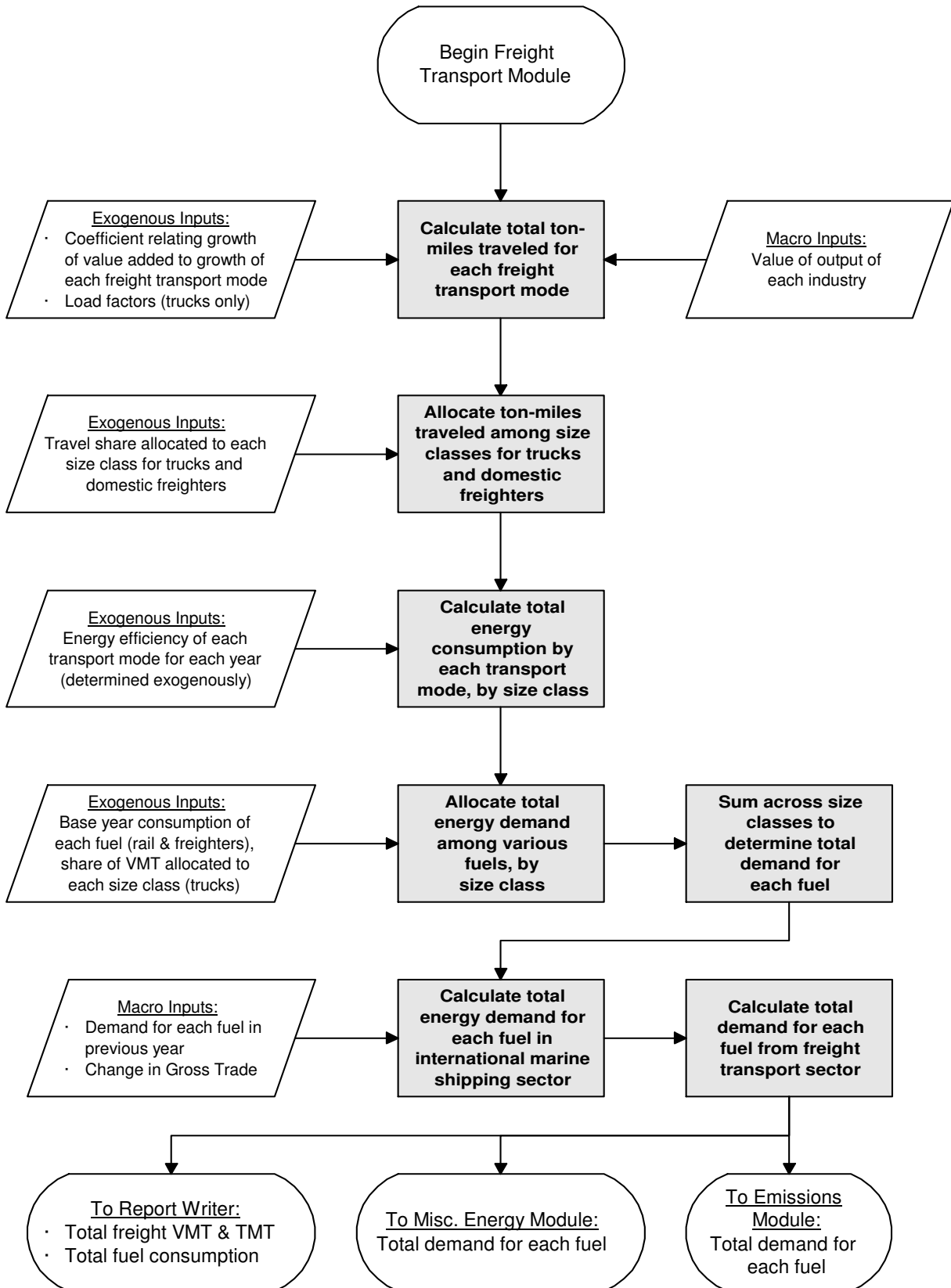
Figure 13. Freight Transport Module
