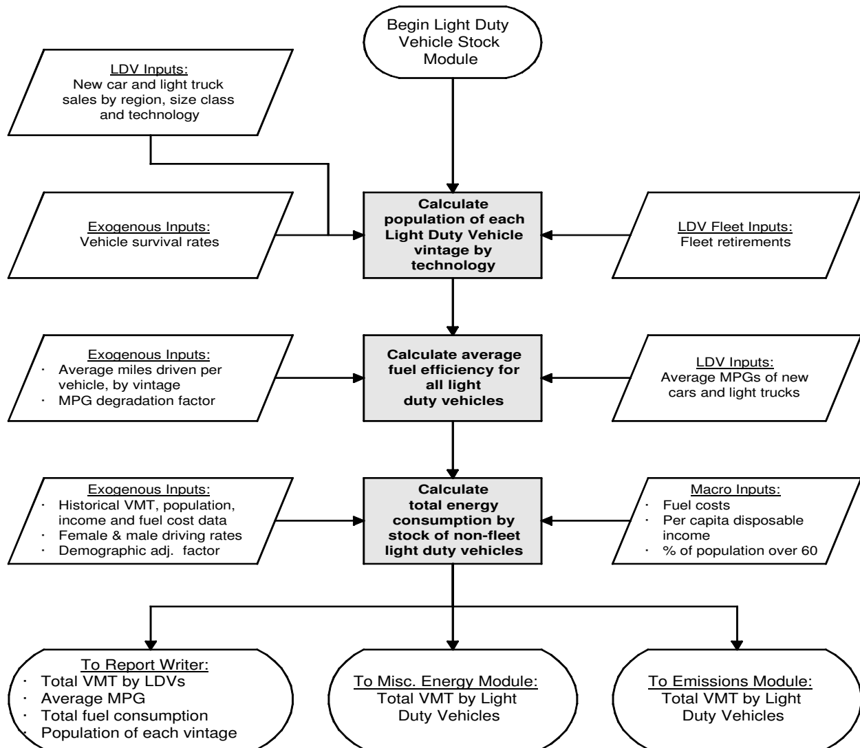
Figure 11. Light Duty Vehicle Stock Module
