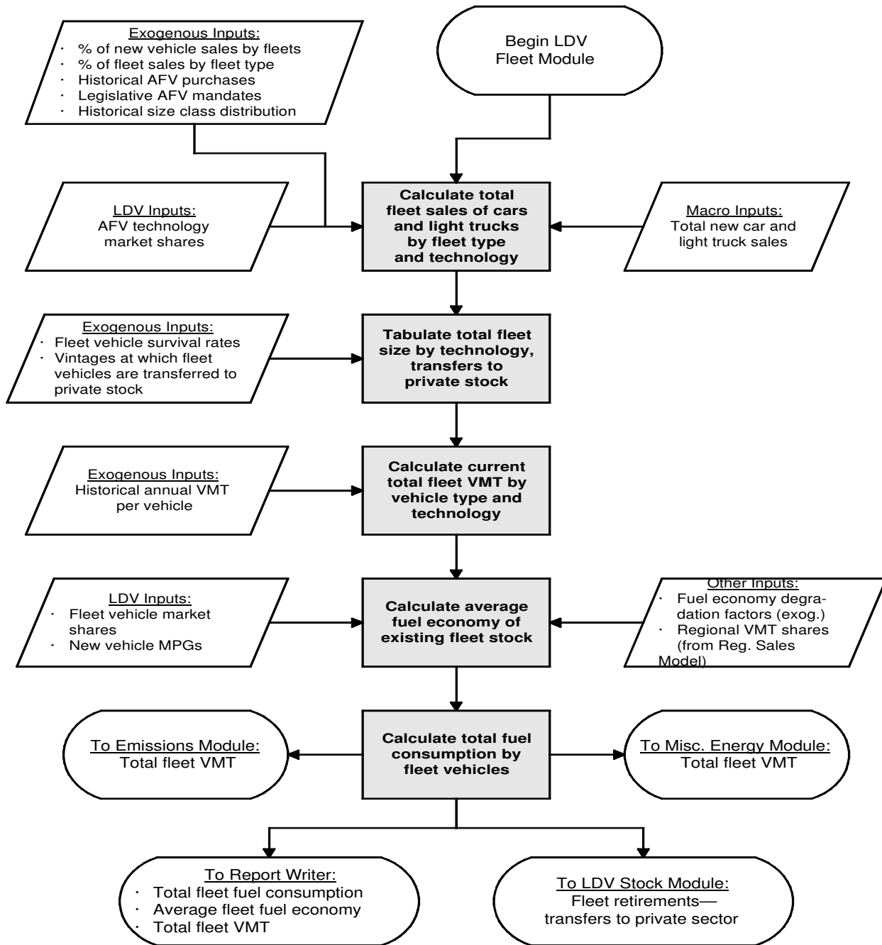
Figure 7. Light Duty Vehicle Fleet Module
