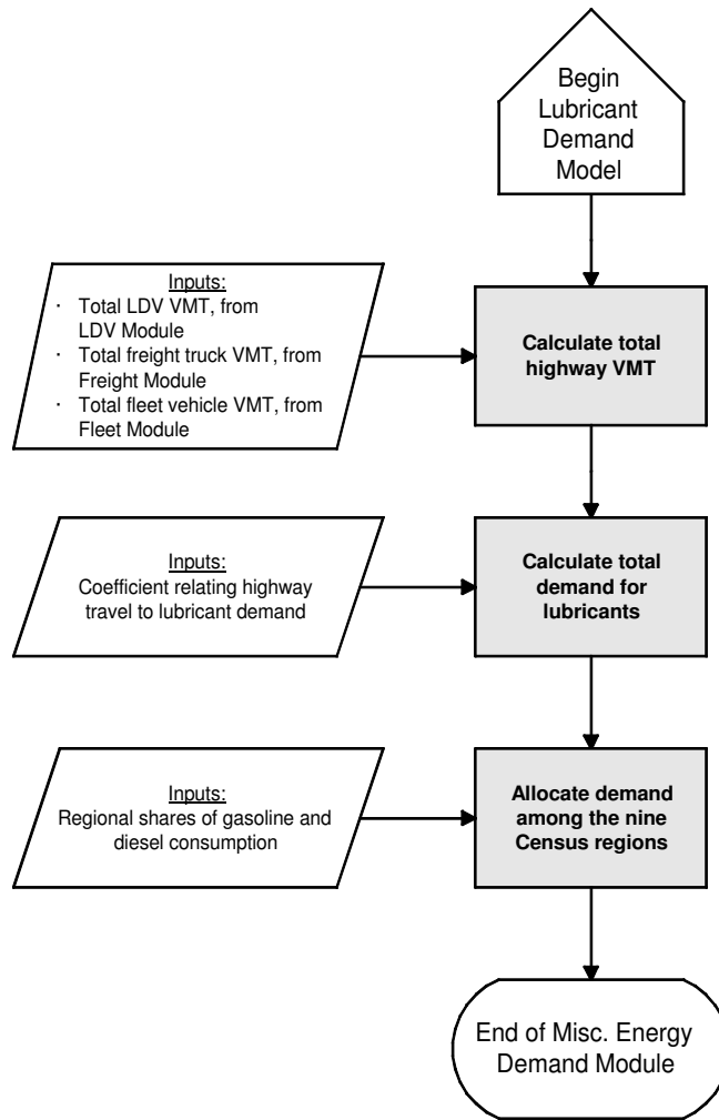
Figure 21. Lubricant Demand Module
