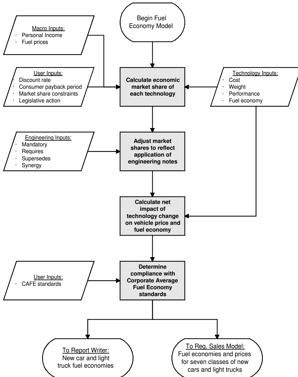
Figure 2. Manufacturers Technology Choice Module
