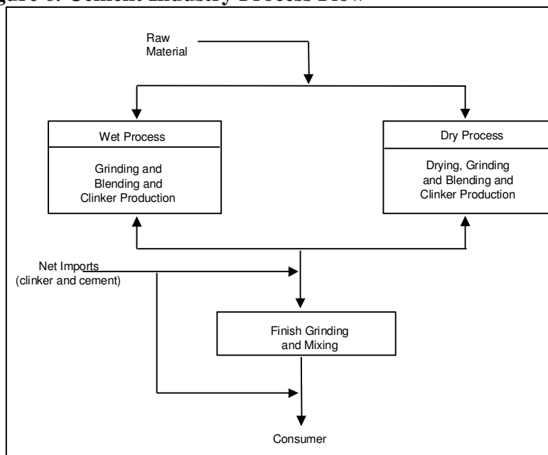
Figure 6. Cement Industry Process Flow
