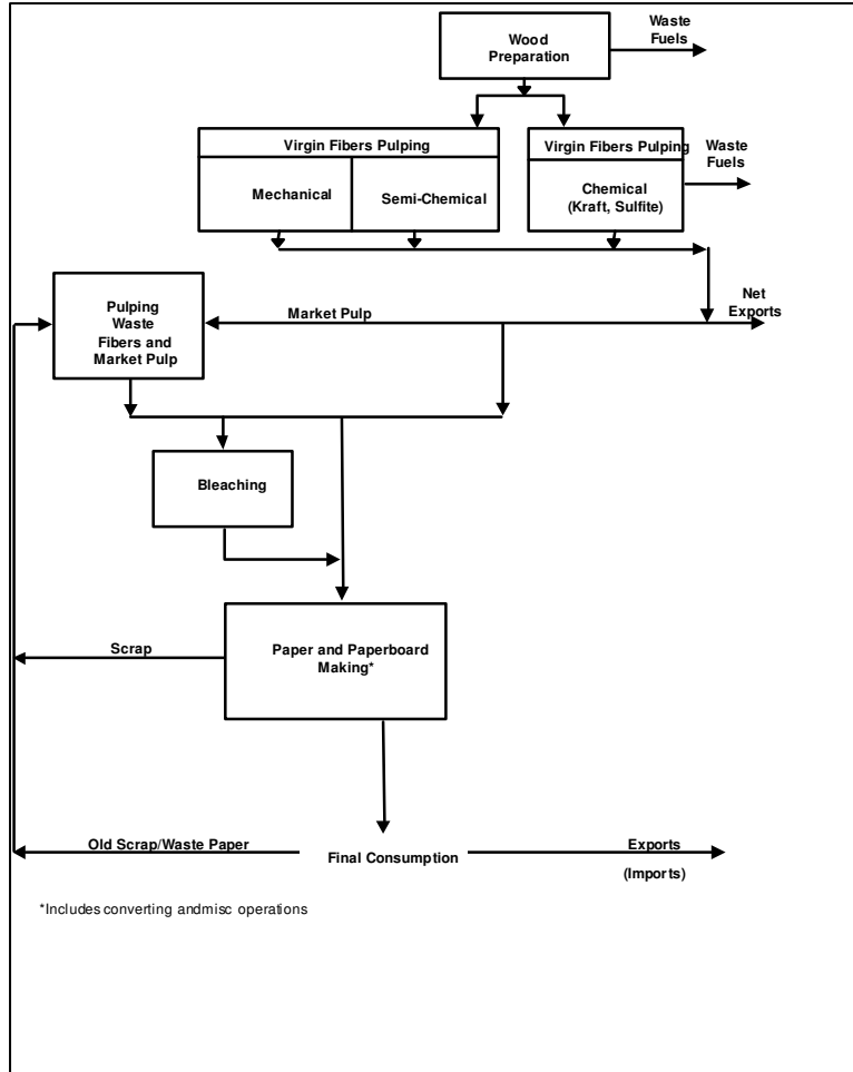
Figure 3. Paper Manufacturing Industry Process Flow
