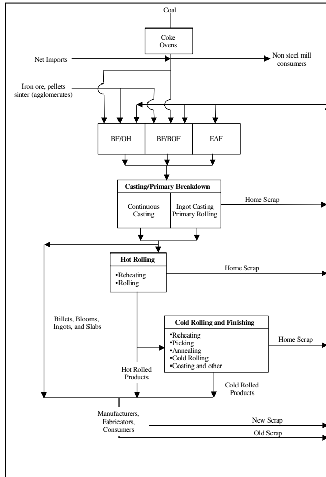
Figure 7. Steel Industry Process Flows
