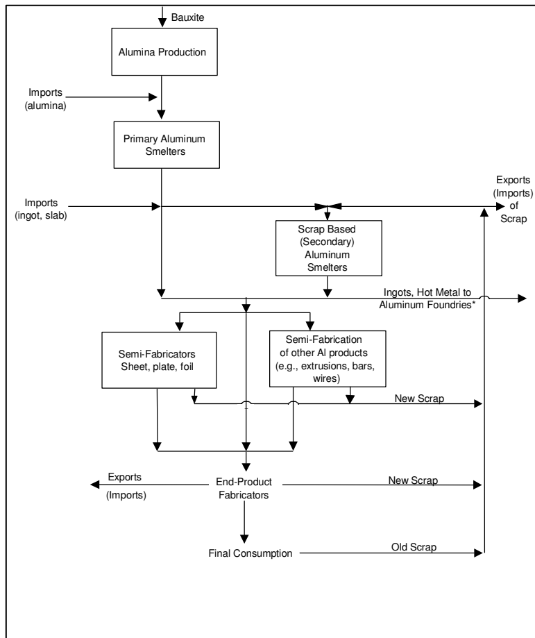
Figure 8. Aluminum Industry Process Flow
