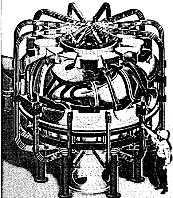
ORNL researchers have designed the compact Quasi-Poloidal Stellarator, a fusion research device that will be built at ORNL this decade.
