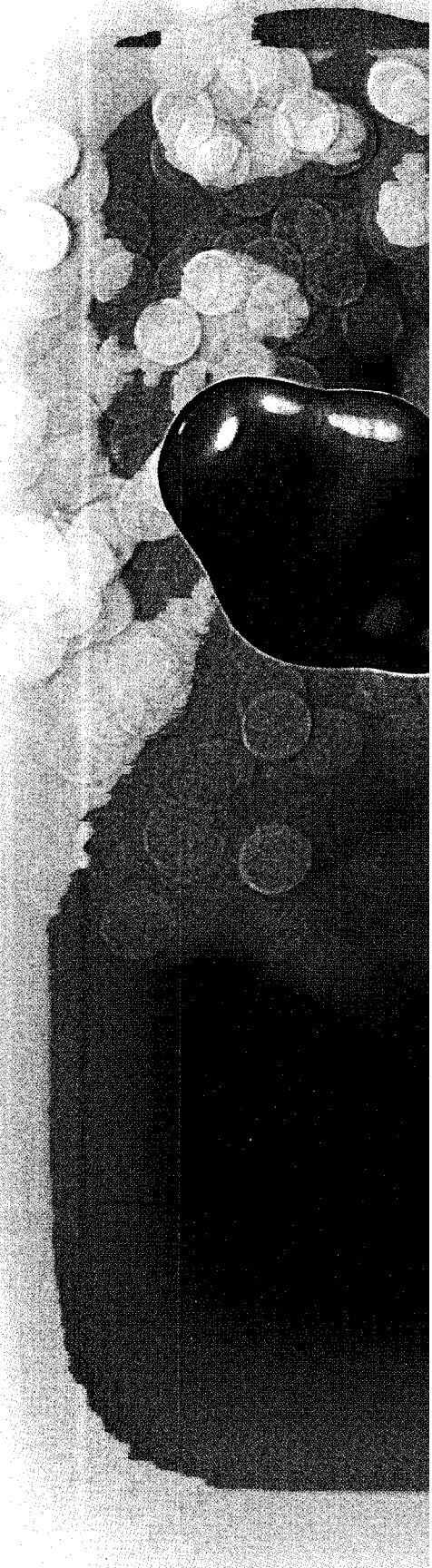
The likely shape of a deformed uranium-234 nucleus was determined in 1971 by ORNL physicists.
