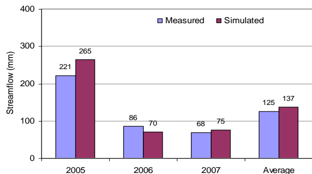
Figure 3. Measured and SWAT predicted annual stream flows for Turkey Creek watershed.
