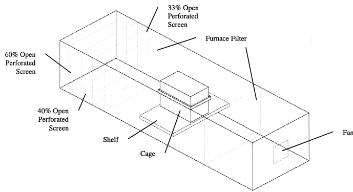
Figure 6 Parallel cage orientation CFD model.
