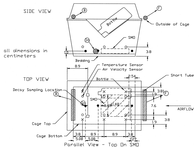
Figure 3 Sensor, air inlet, and sampling location for cage parallel to horizontal airflow. Mouse heater representation: SMO.
