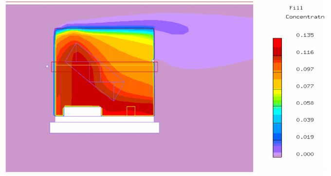
Figure 11 Close-up plot of the CO 2 concentration field mid-plane of tunnel. Series set six: parallel orientation, heater on (SMO), 40 fpm (0.2 m/s).
