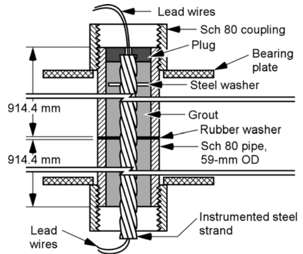
Figure 3.—Pull-test apparatus.
