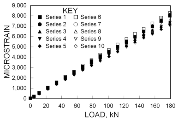
Figure 4.—Calibration curve for instrumented cable bolt.
