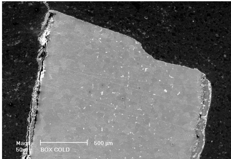
Figure 4-7. Cross Section of Car 50 Roof Approximately 40 cm [16 in] from the Edge Directly Exposed to the Fire. Thickness of the Metal Was Approximately 1,761 \mu\text{m} [0.069 in].
