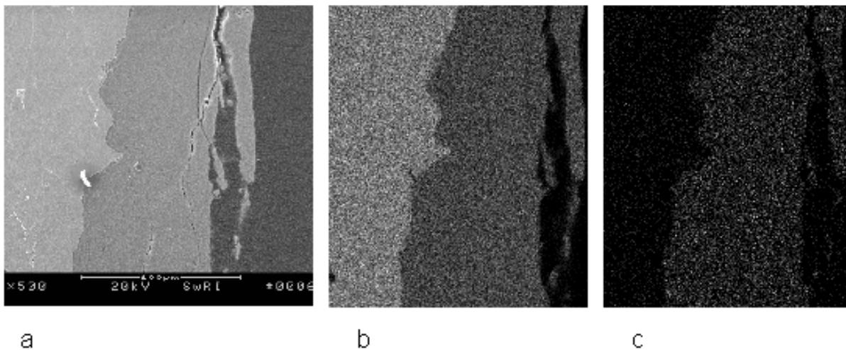
Figure 4-10. (a) Secondary Electron Image from Car 50 Roof at Edge Directly Exposed to the Fire, (b) Iron Image Map, and (c) Oxygen Image Map
