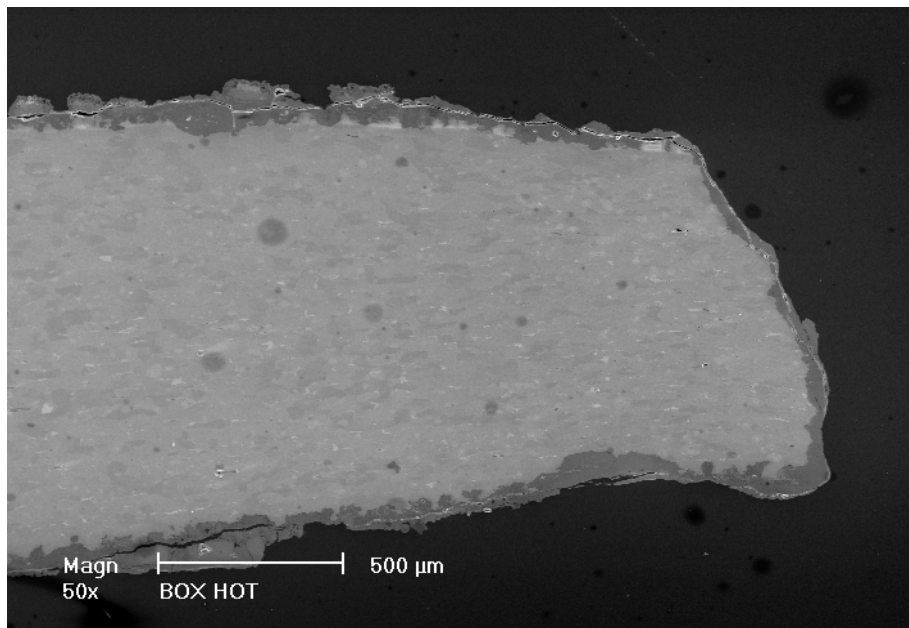
Figure 4-9. Cross Section of Car 50 Roof at Edge Directly Exposed to the Fire. Thickness of the Metal Ranged from 829 to 930 \mu\text{m} [0.033 to 0.037 in].
