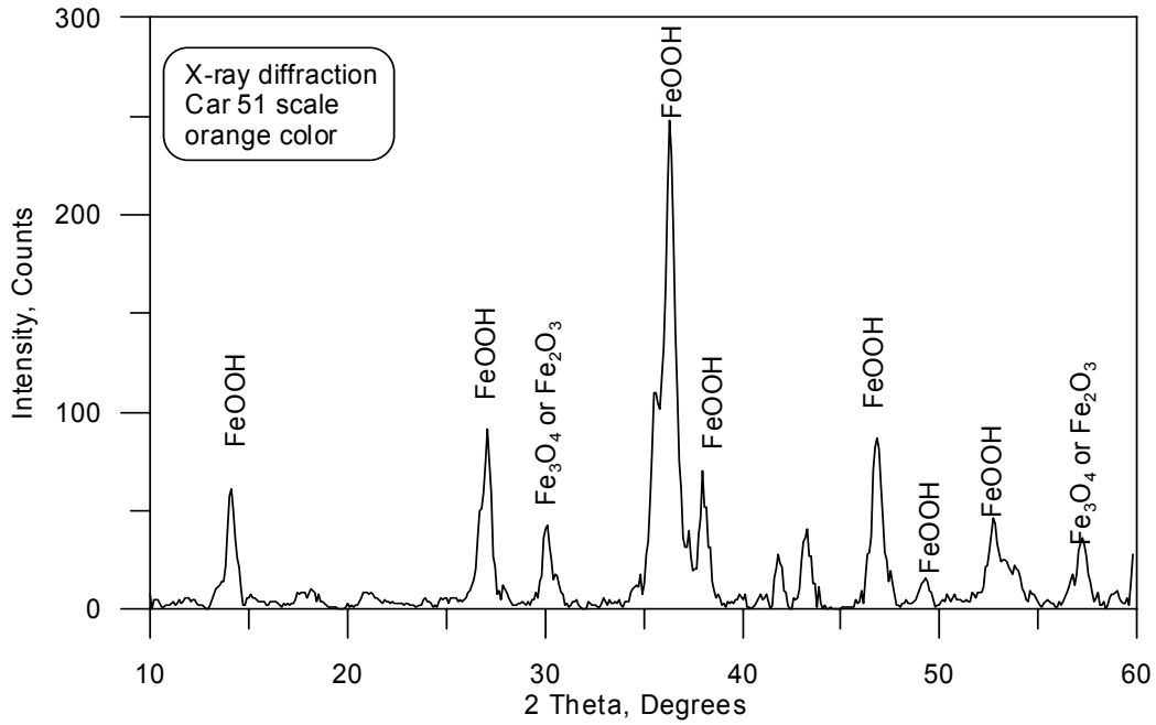
Figure 4-5. X-Ray Diffraction of Orange Colored Oxide Scales from Car 51
