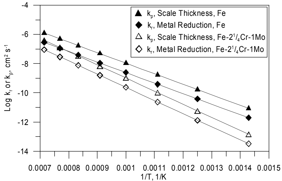
Figure 4-1. Oxidation Rate Constants for Fe-2 1 / 4 Cr-1Mo Steel and Iron as a Function of Temperature Based on Results Reported by Simms and Little (1987) and Kubaschewski and Hopkins (1962)
