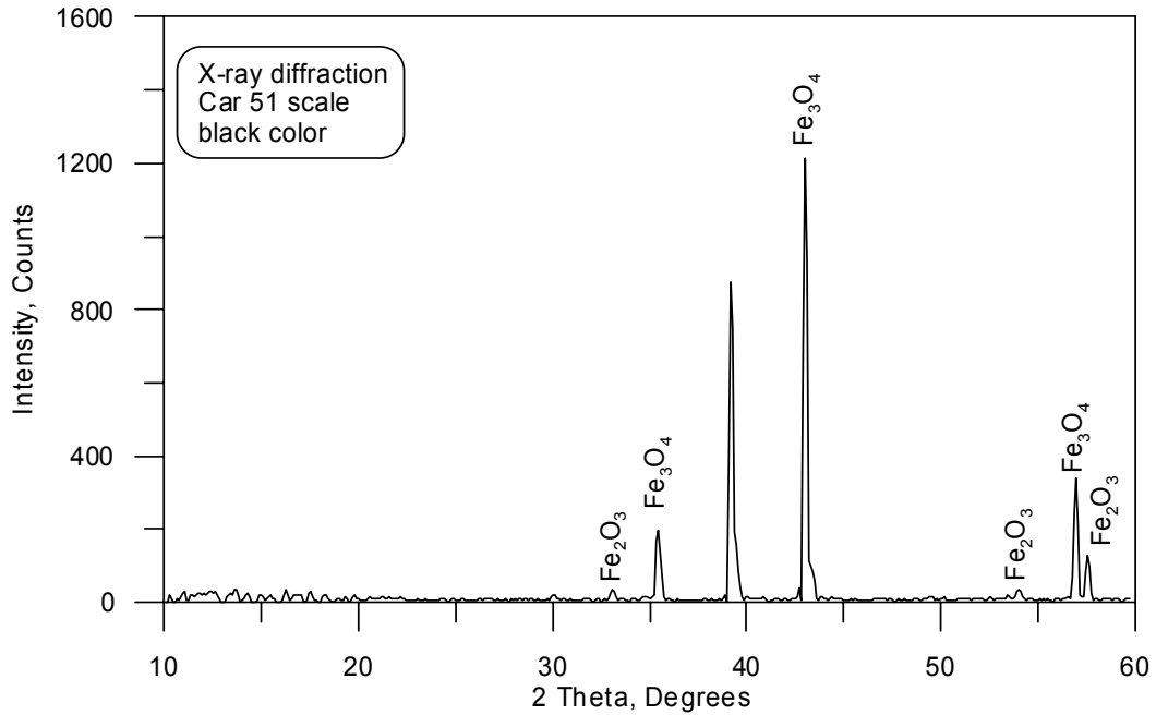
Figure 4-6. X-Ray Diffraction of Black Colored Oxide Scales from Car 51
