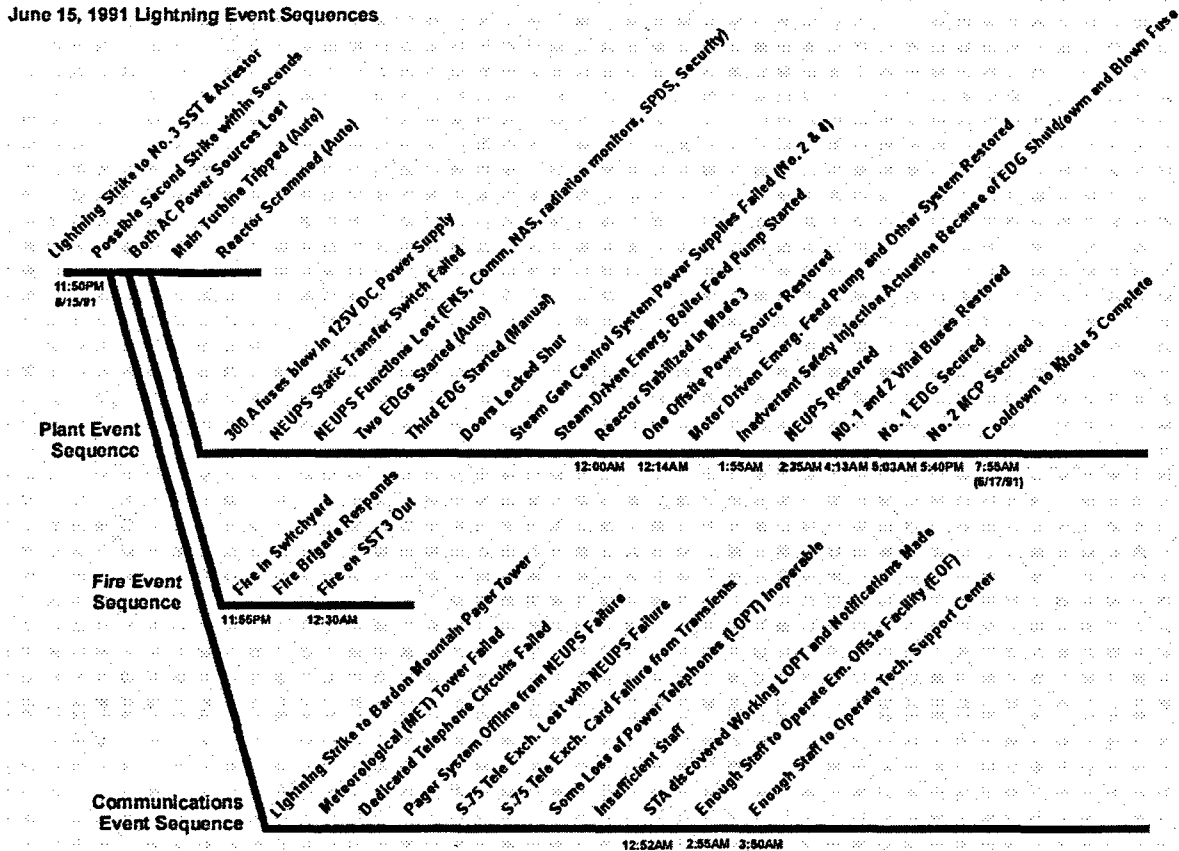
Figure 6. Yankee Nuclear Power Station June 15, 1991 Lightning Event Sequence
