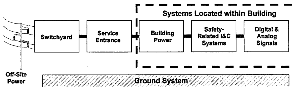
Figure 2. Elements of the power plant system.
