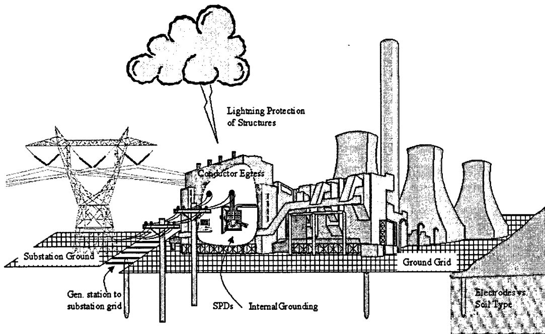
Figure 7. Issues for lightning protection in generating stations.
