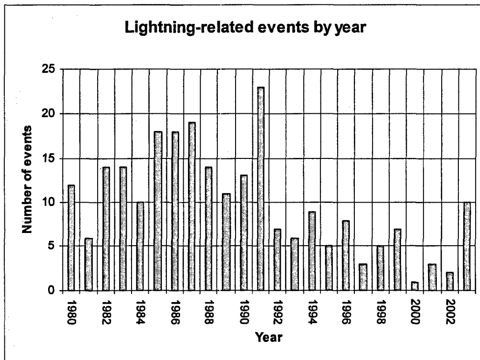
Figure 5. Lightning-related events by year.
