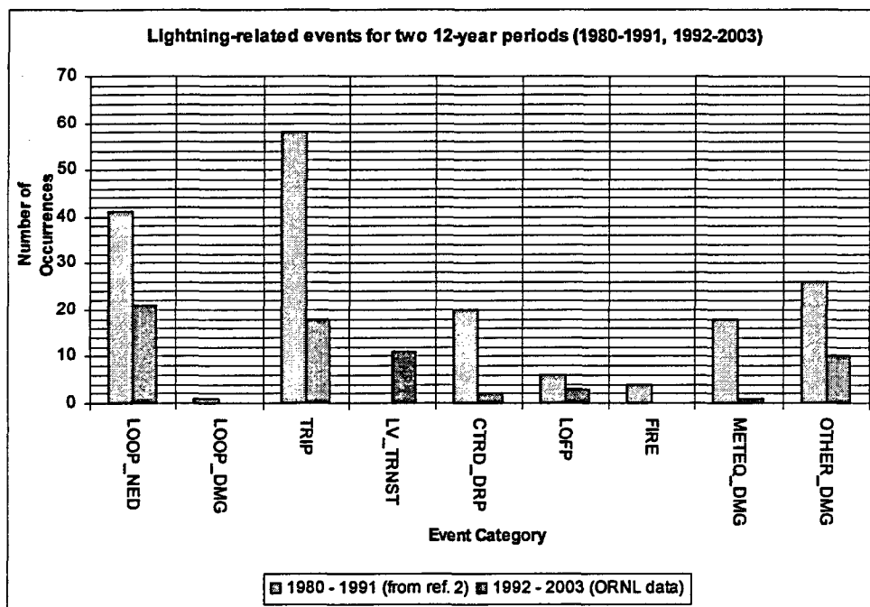
Figure 4. Lightning-related events for 2, 12-year periods (1980-1991, 1992-2003)
