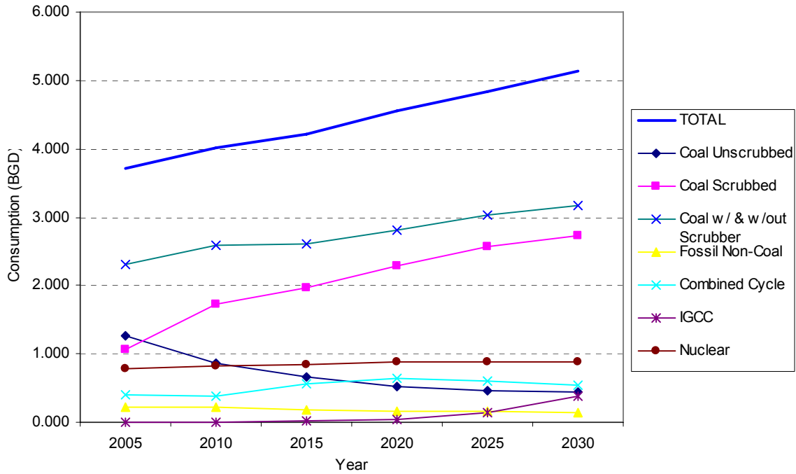
Figure 14 - Average Daily National Freshwater Consumption by Fuel for Thermolectric Power Generation – Case 1
