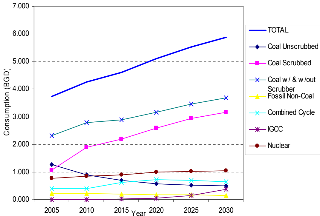
Figure 22 - Average Daily National Freshwater Consumption by Fuel for Thermolectric Power Generation – Case 5
