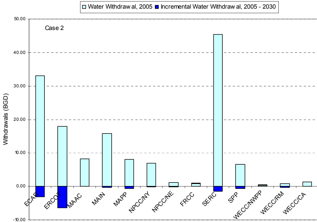
Figure ES-1 – Average Daily Regional Freshwater Withdrawal for Thermolectric Power Generation – Case 2
