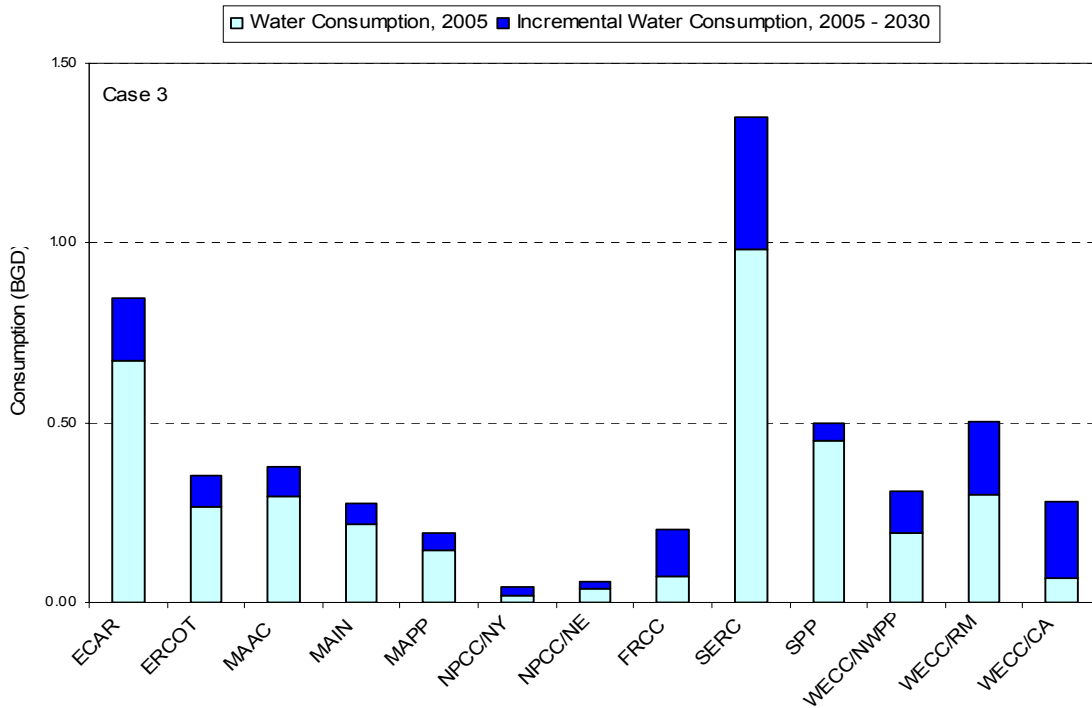
Figure 30 – Average Daily Regional Freshwater Consumption for Thermoelectric Power Generation – Case 3
