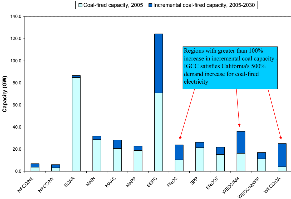
Figure 7 – Coal-Fired Capacity, 2005 vs. 2030, by NERC region
