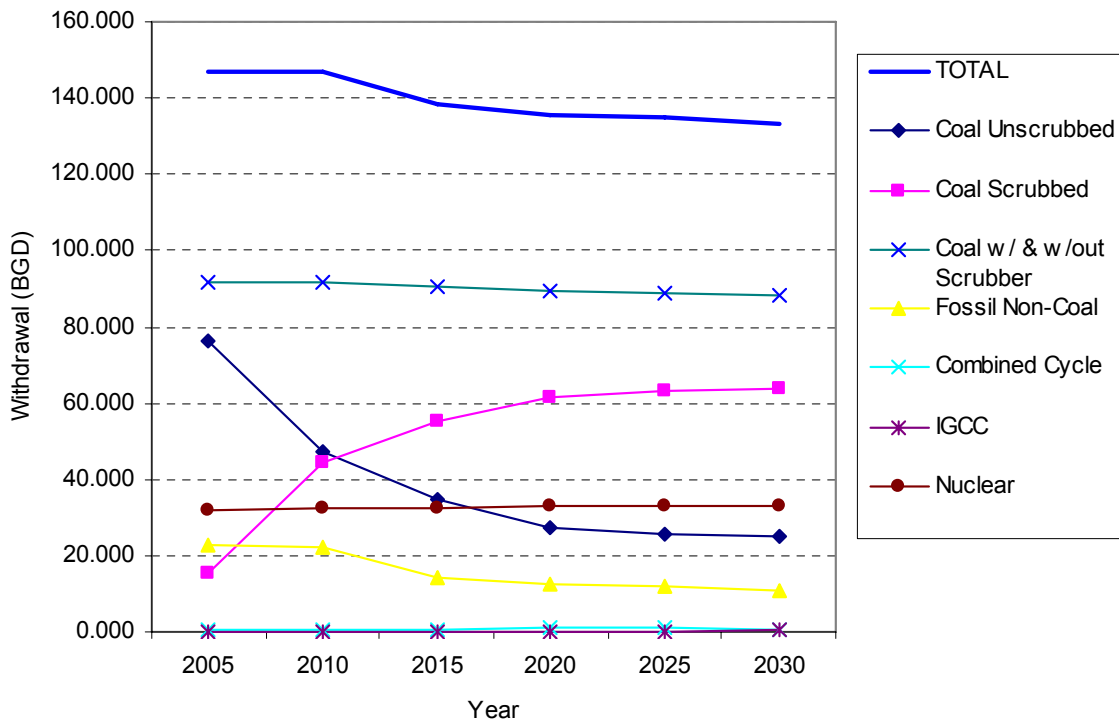
Figure 17 - Average Daily National Freshwater Withdrawal by Fuel for Thermoelectric Power Generation – Case 3
