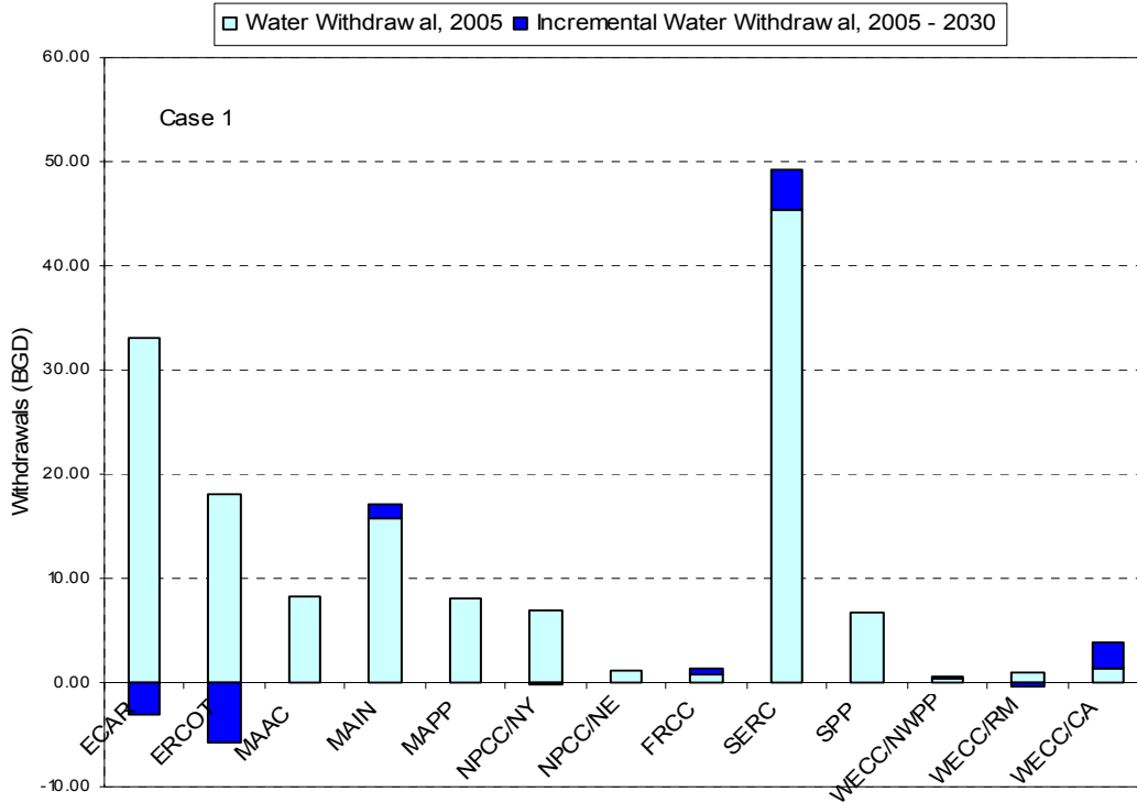
Figure 23 – Average Daily Regional Freshwater Withdrawal for Thermoelectric Power Generation – Case 1
