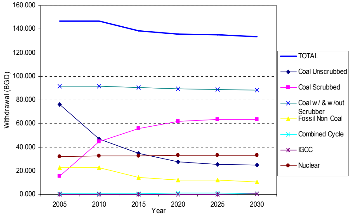
Figure 15 - Average Daily National Freshwater Withdrawal by Fuel for Thermolectric Power Generation – Case 2
