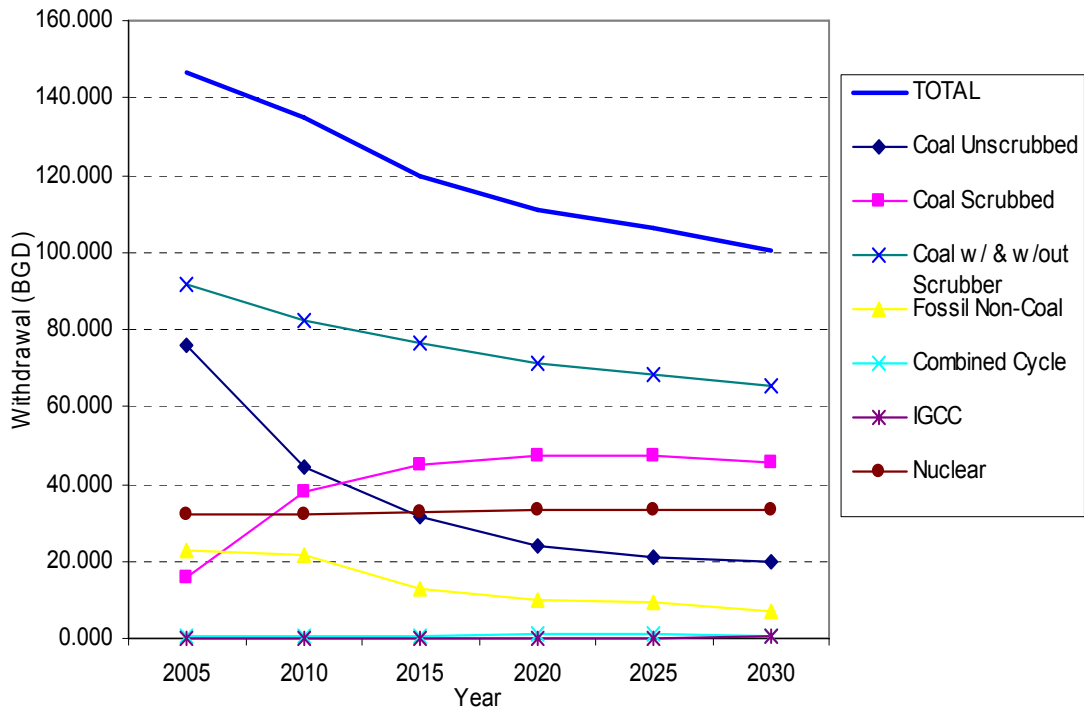
Figure 21 - Average Daily National Freshwater Withdrawal by Fuel for Thermolectric Power Generation – Case 5
