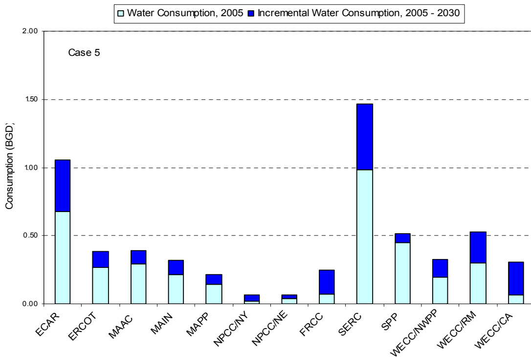
Figure 32 – Average Daily Regional Freshwater Consumption for Thermolectric Power Generation – Case 5
