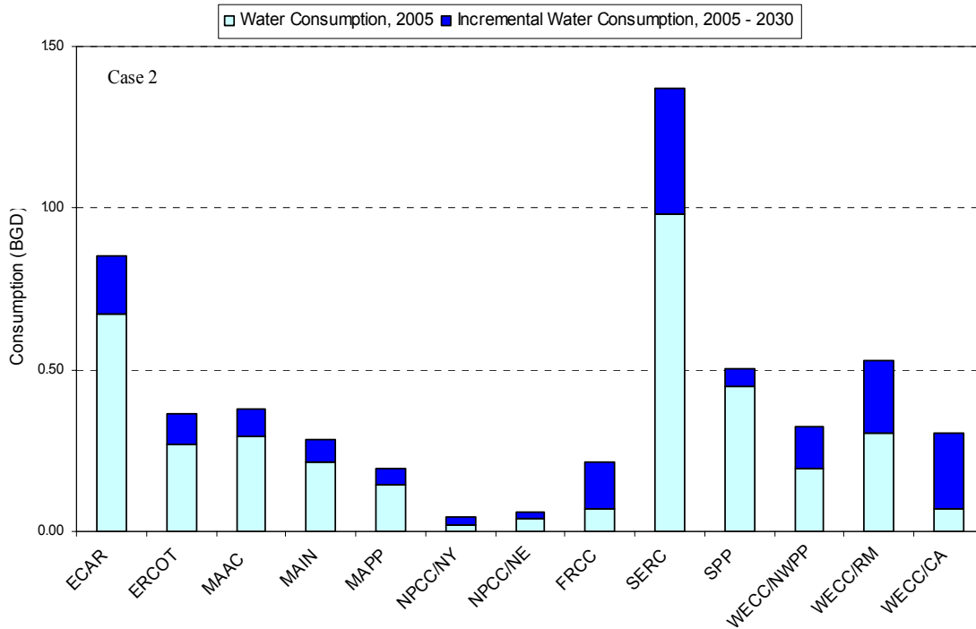
Figure ES-2 - Average Daily Regional Freshwater Consumption for Thermoelectric Power Generation – Case 2
