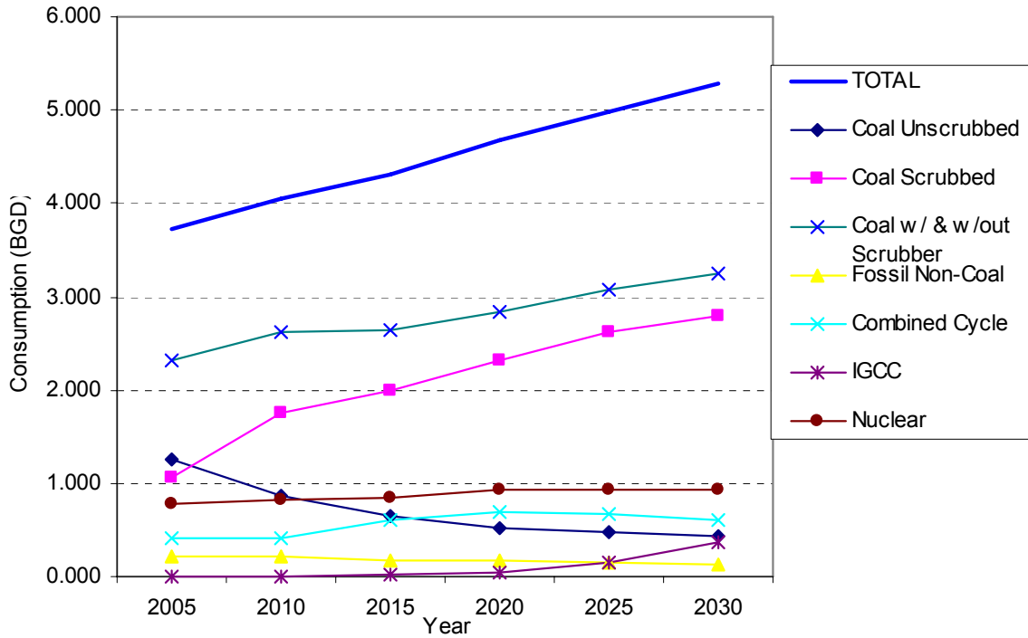
Figure 18 - Average Daily National Freshwater Consumption by Fuel for Thermolectric Power Generation – Case 3
