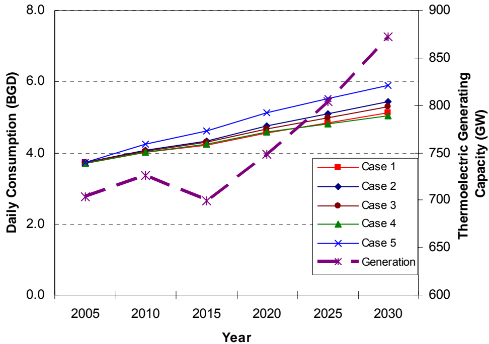
Figure 12 – Average Daily National Freshwater Consumption for Thermolectric Power Generation
