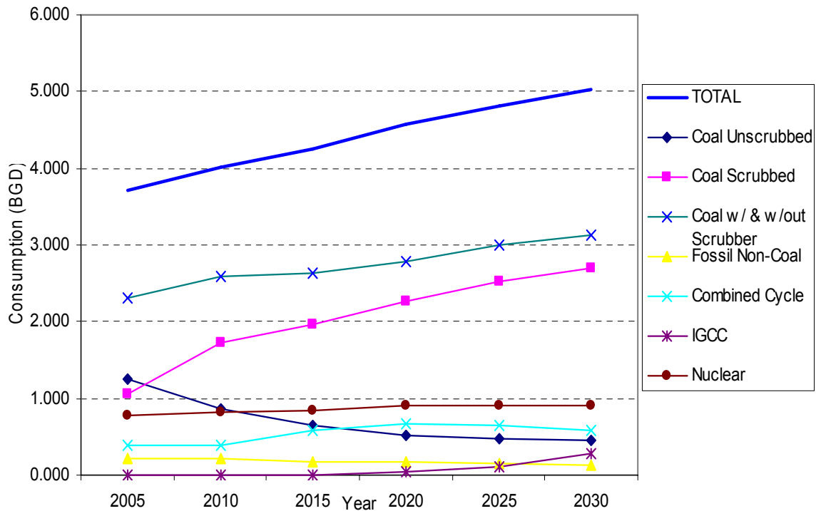
Figure 20 - Average Daily National Freshwater Consumption by Fuel for Thermolectric Power Generation – Case 4
