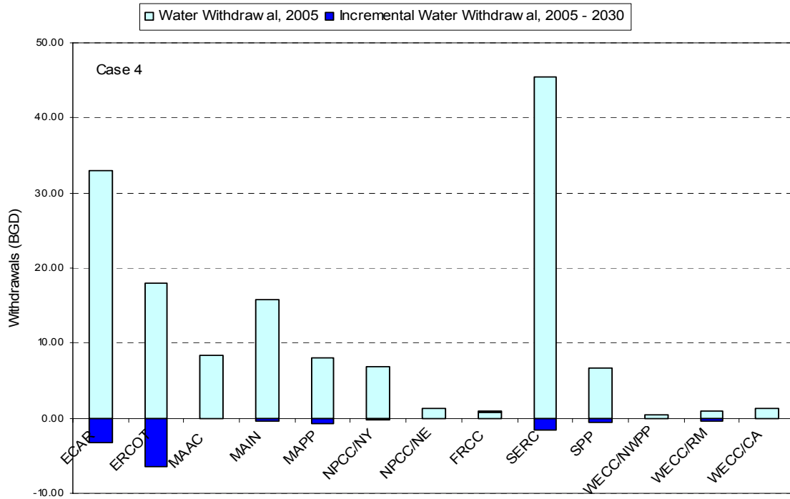
Figure 26 – Average Daily Regional Freshwater Withdrawal for Thermolectric Power Generation – Case 4
