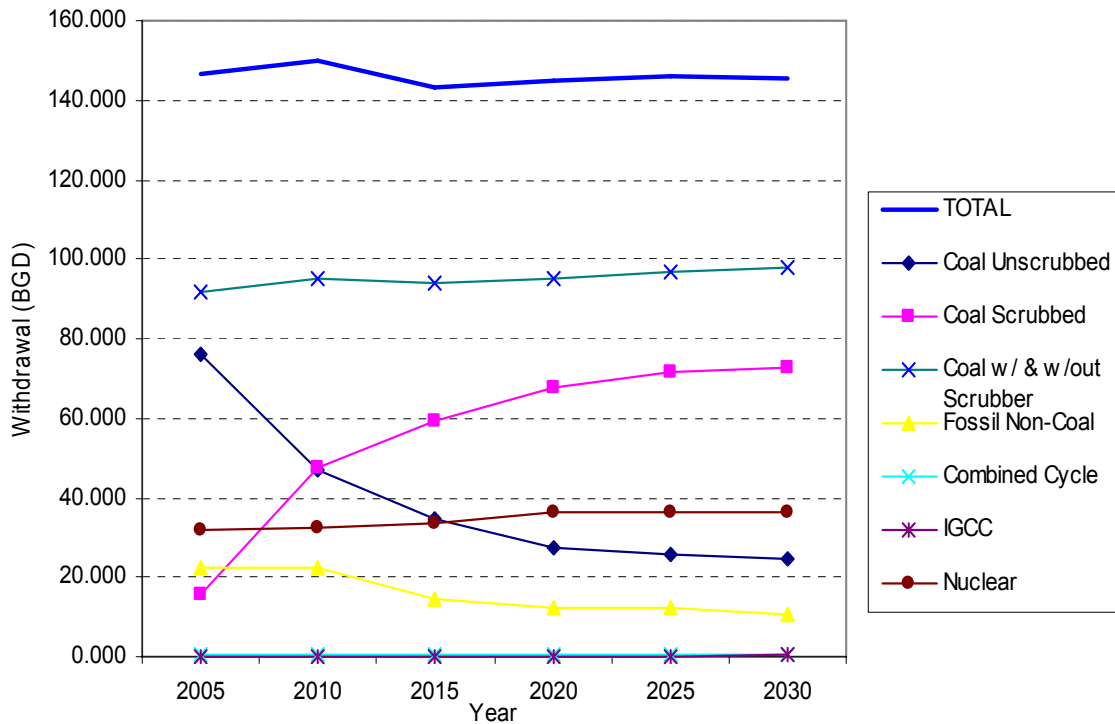
Figure 13 - Average Daily National Freshwater Withdrawal by Fuel for Thermolectric Power Generation – Case 1
