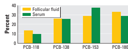
Figure 1. Distribution pattern of PCB congeners in follicular fluid and serum ( n = 9 ) according to their fractions. The concentration of the sum of PCBs was set at 100%.
