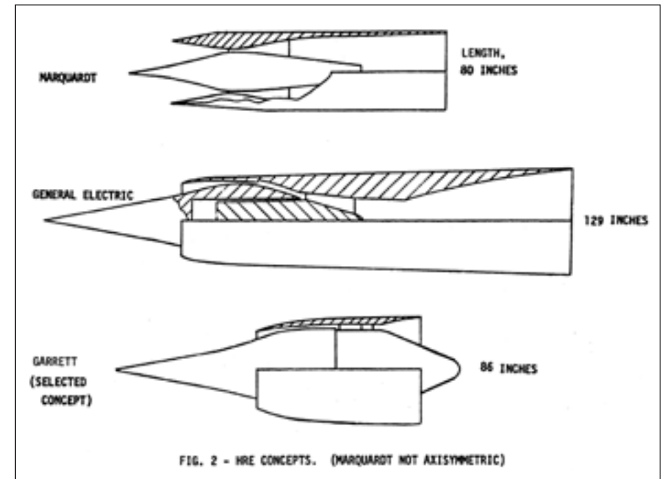
The HRE concepts of three competing contractors. (NASA)
