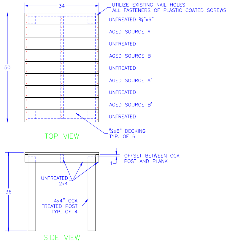
Figure 2-2. Schematic of Mini-Deck Construction (note that untreated 34" specimens shall be planed so that 1/8" of space is provided between each pair of specimens)
