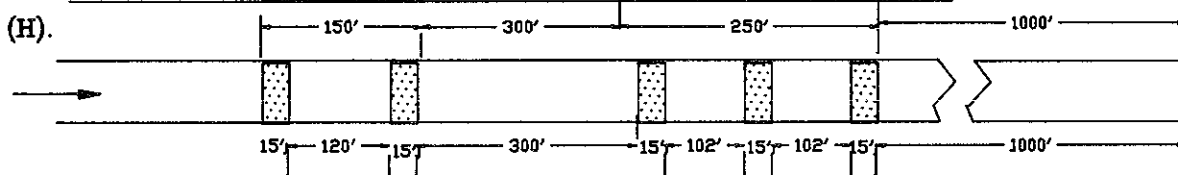
Figure 3. Intermittent rumble strips for stop-sign controlled intersections
