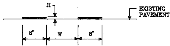
PART-SECTION A-A
