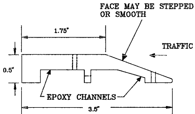
A-A DETAIL OF RUMBLE STRIPS
