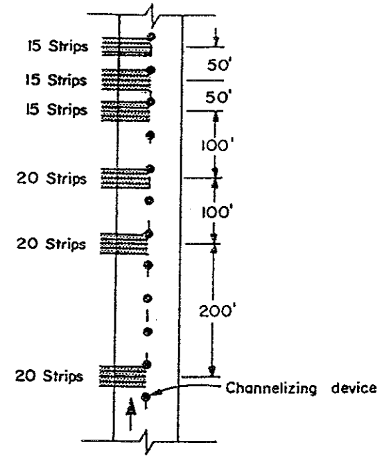
RUMBLE STRIP PATTERN B
