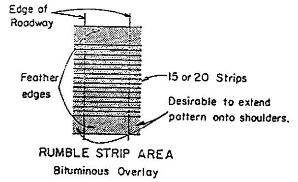
RUMBLE STRIP PATTERN A
