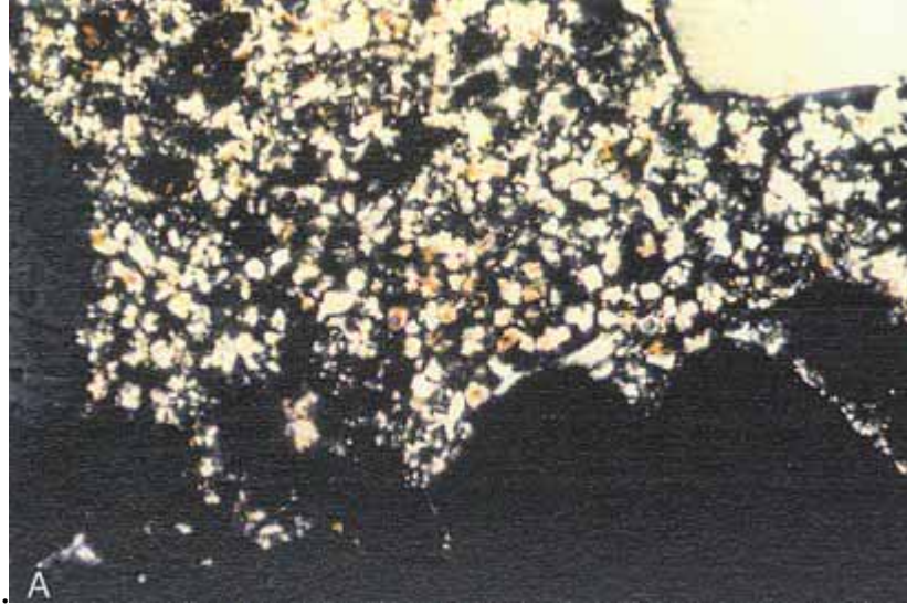
Figure 159. Thin section of interior portion of HCC: (A) Viewed with crossed nicols (bright area shows the high birefringence of the calcite of the carbonated area).
