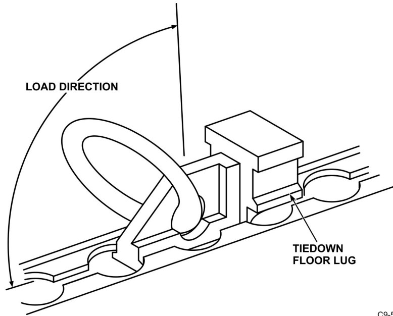
Figure 2. Floor Attachment Assembly Installed Dimension (representative of NASA C-9B)
