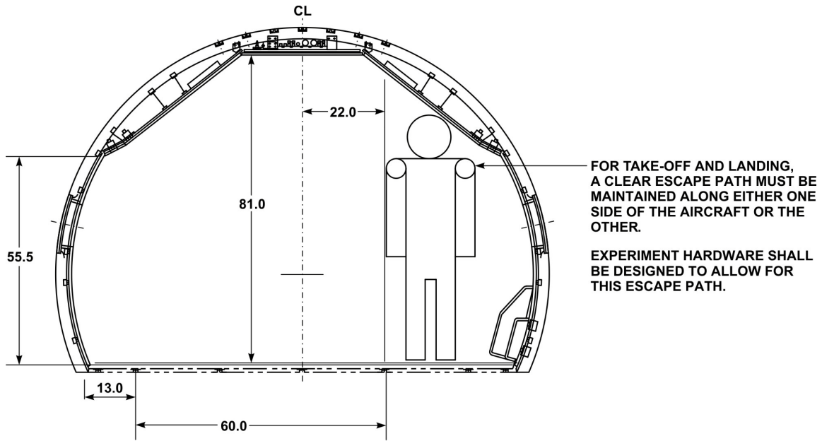
VIEW LOOKING FORWARD C-9B INTERIOR CROSS SECTION
