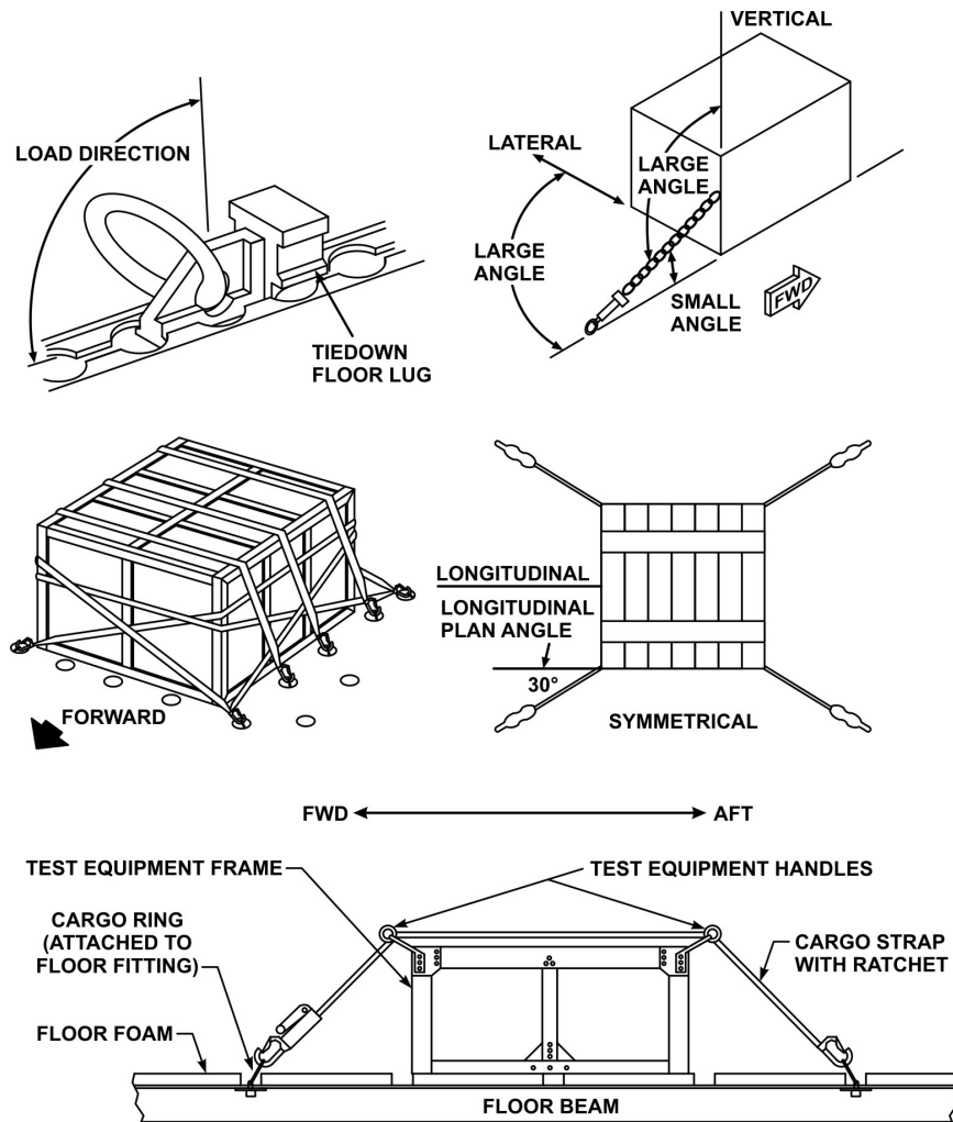
Figure 1. Cargo Strap (for Reference Only)
