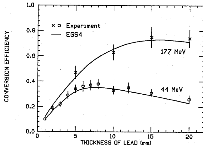
Figure 4. Absolute comparison of EGS4 simulation with a conversion efficiency experiment by Darriulat et al 6 .
