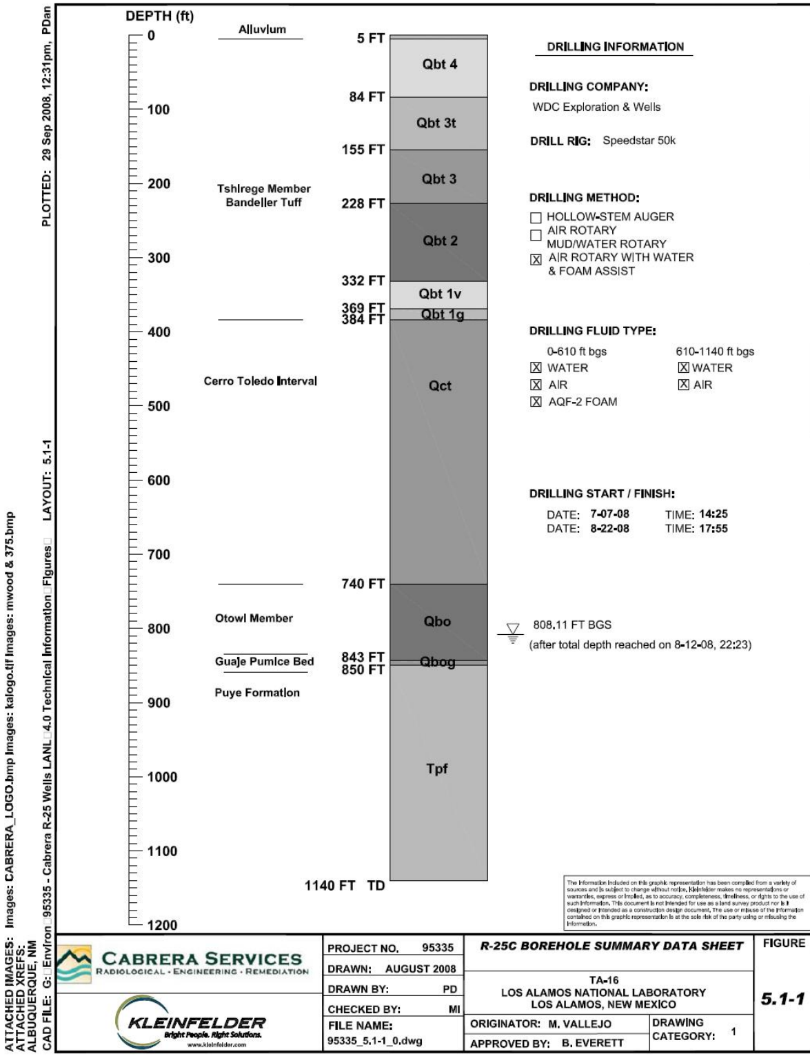
Figure 5.1-1 R-25c borehole summary data sheet
