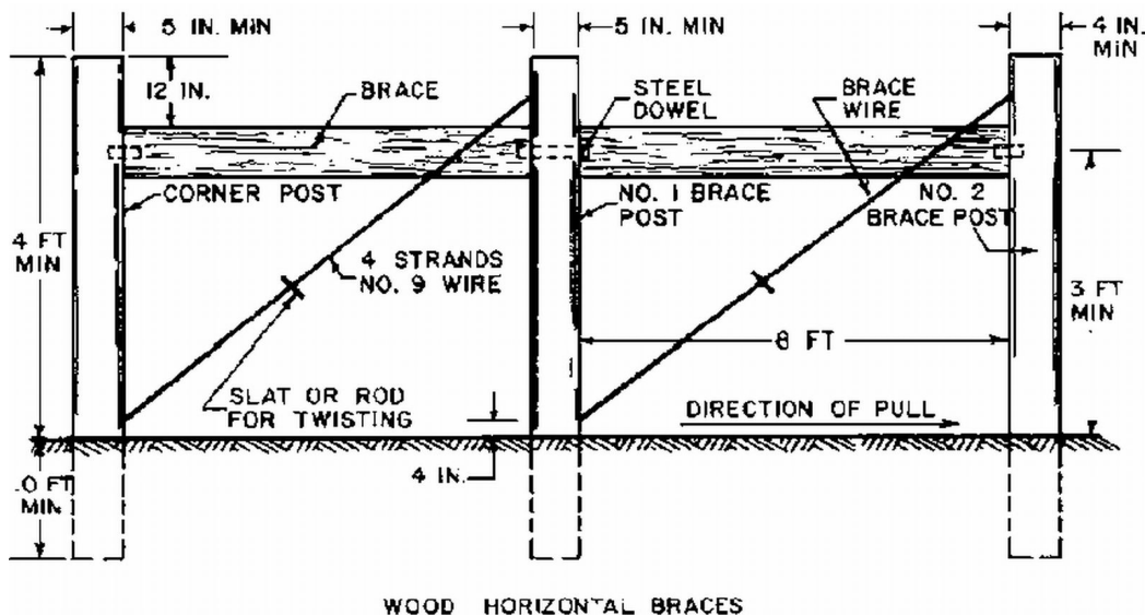
Figure 2. Corner and End Brace Assemblies.
