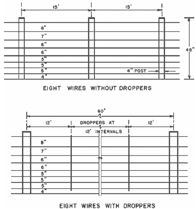
Figure 1. High-Tensile Wire Spacing.
