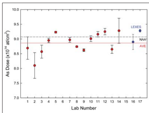
Figure 4. As round robin results for medium dose sample with point-by-point normalization to matrix signal. SIMS lab results shown in red with error bars indicating within-lab repeatability. Relative standard deviation among labs is 3.9 %. Also shown are LEXES results (blue dots), average of SIMS lab results (red line), and NAA result (black dashed line).
