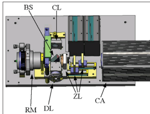
Figure 1a. NIST's infrared interferometer ( IR^2 ). The main components of the interferometer are: collimator lens (CL), polarizing beam splitter (BS), phase-shifting reference mirror mount (RM), diverger lens (DL), zoom lens system (ZL), and camera (CA).
