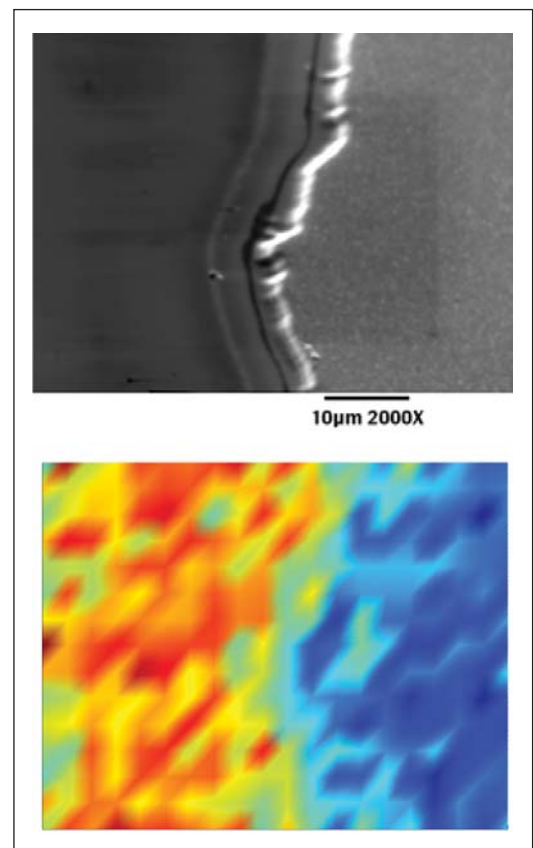
Figure 7. SEM photo (top) of an aluminum film partially covering a sapphire substrate and a false-color map (bottom) of the shift in the mean X-ray energy of the Al Ka peak taken using a microcalorimeter EDS system. The shift in energy is due to the chemical bonding of the aluminum with the oxygen. The average energy shift is \sim 0.2 eV.
