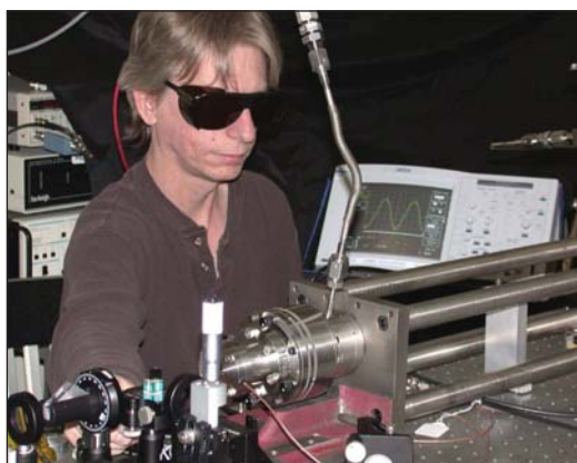
Figure 3. Frequency-stabilized CRDS system.
